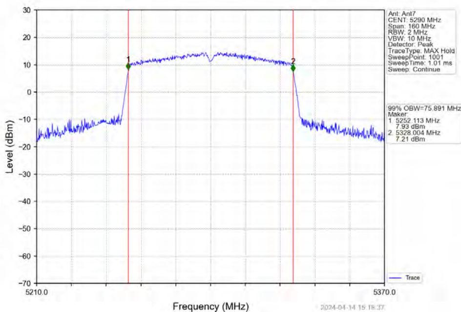
802.11ac(VHT80)_MCH_5290MHz_Ant7_NTNV
