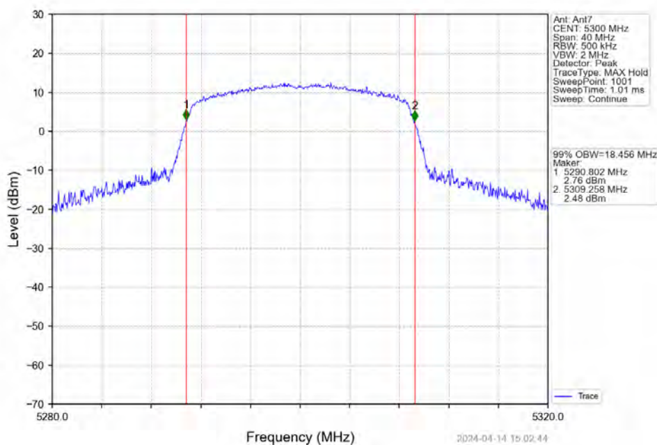
802.11ac(VHT20)_MCH_5300MHz_Ant7_NTNV
