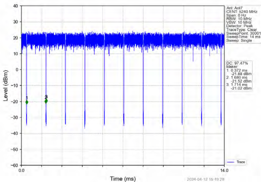
802.11ac(VHT20)_HCH_5240MHz_Ant7_NTNV
