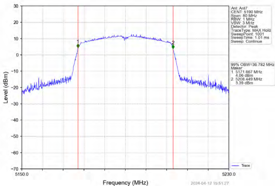
802.11ac(VHT40)_LCH_5190MHz_Ant7_NTNV
