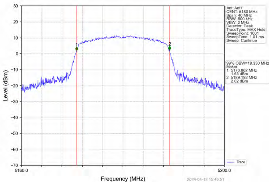
802.11ac(VHT20)_LCH_5180MHz_Ant7_NTNV
