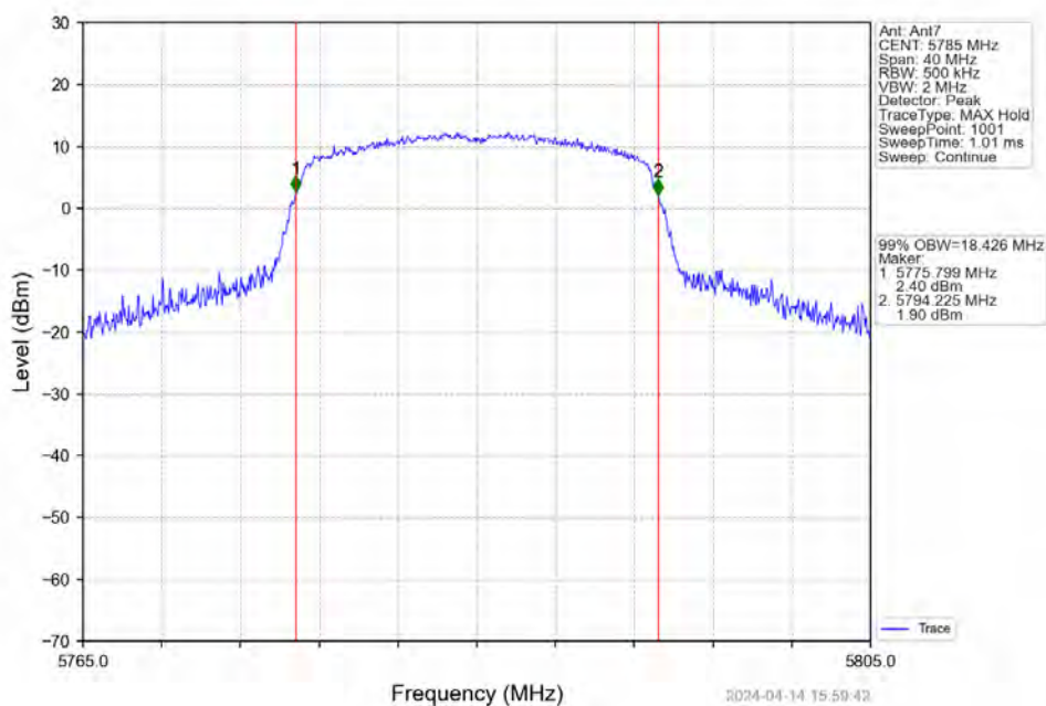
802.11ac(VHT20)_MCH_5785MHz_Ant7_NTNV
