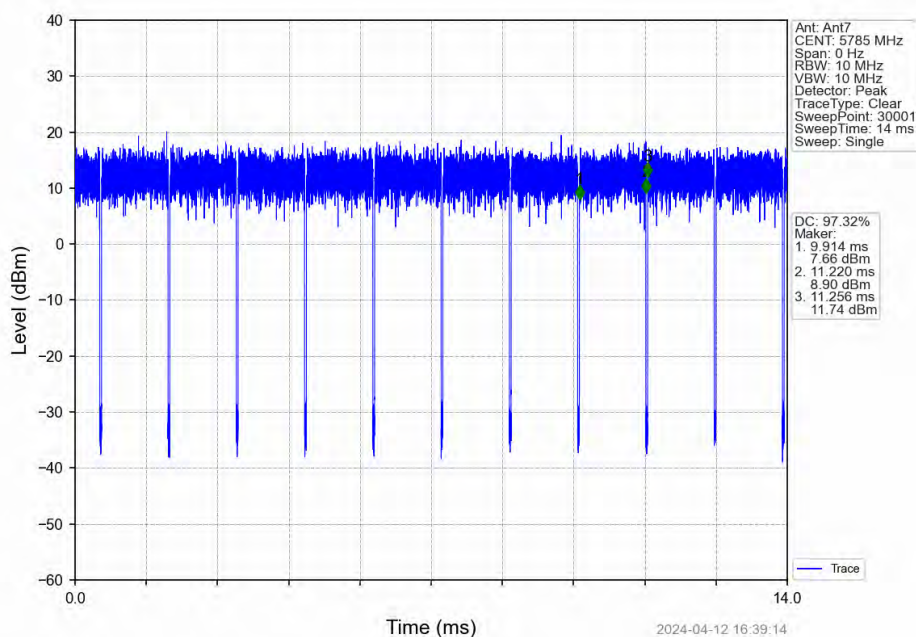
802.11ac(VHT20)_MCH_5785MHz_Ant7_NTNV
