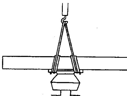
FIG. 2.3 SCANNER SUSPENSION
