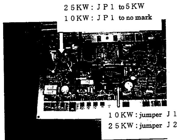
FIG. 6. 2 SETTING OF POWER SUPPLY
