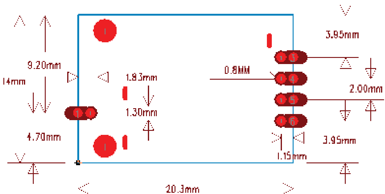
Figure 6 Module dimension
