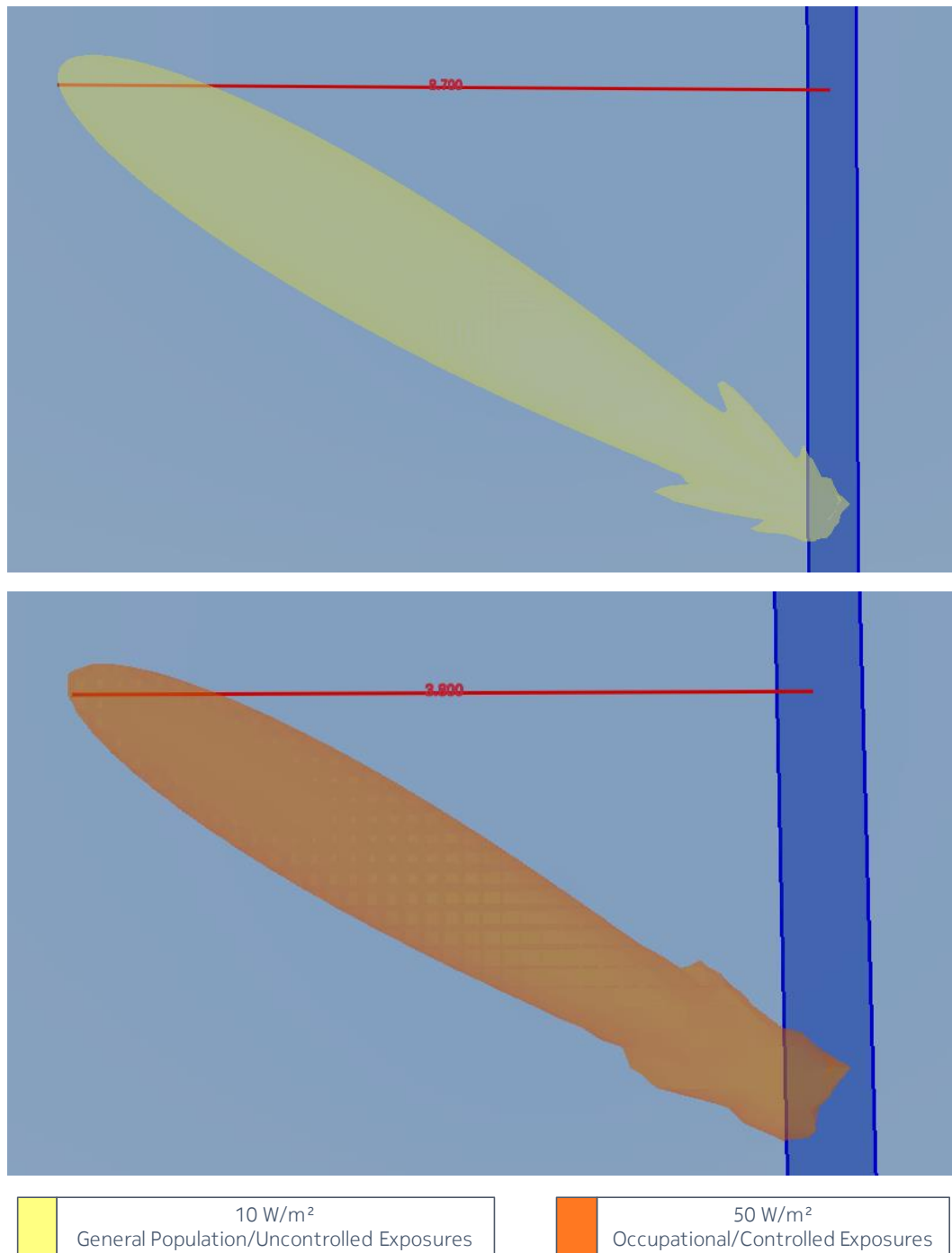
Figure 6 – Compliance distance on the side ( D_{s,c} ) for the time-averaged maximum transmitted power of 127 W and the beam oriented in azimuth = 60° & elevation = - 3°
