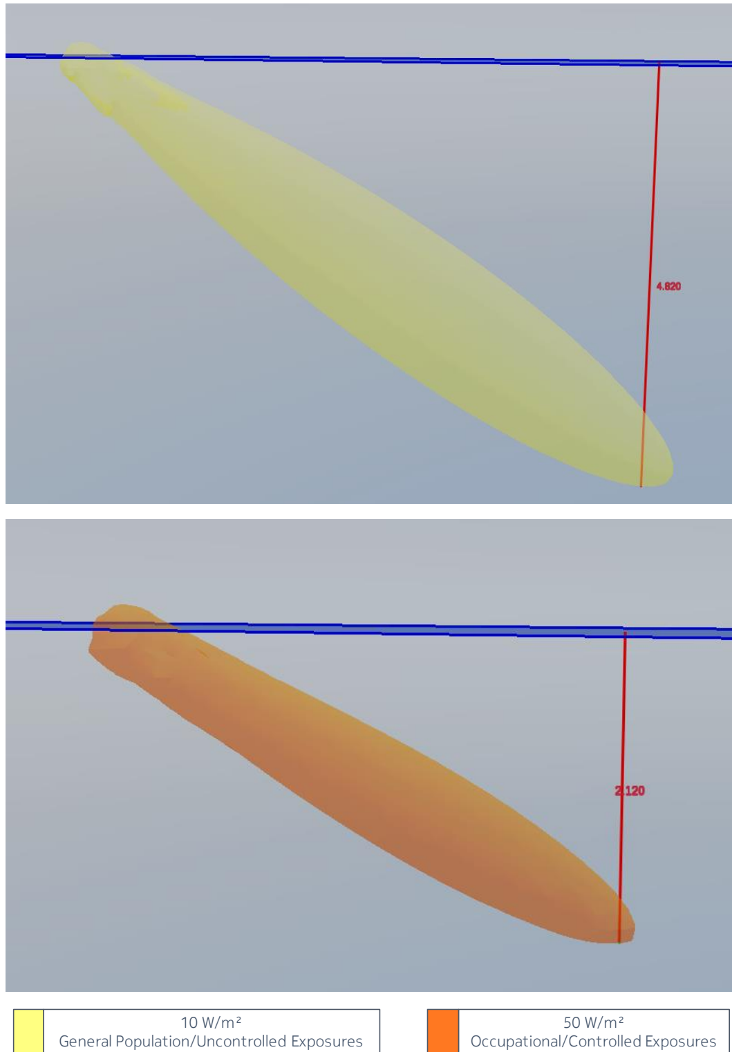
Figure 4 – Compliance distance down ( D_{d,c} ) for the time-averaged maximum transmitted power of 127 W and the beam oriented in azimuth = 0^\circ & elevation = -23^\circ
