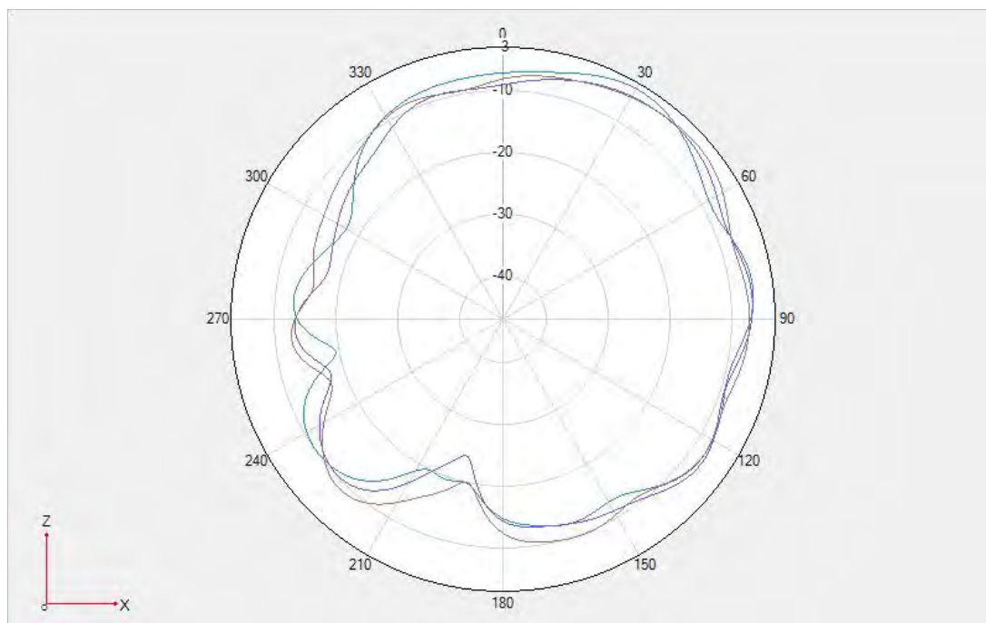
Fold- LTE B40/N40 \Phi=0^\circ
