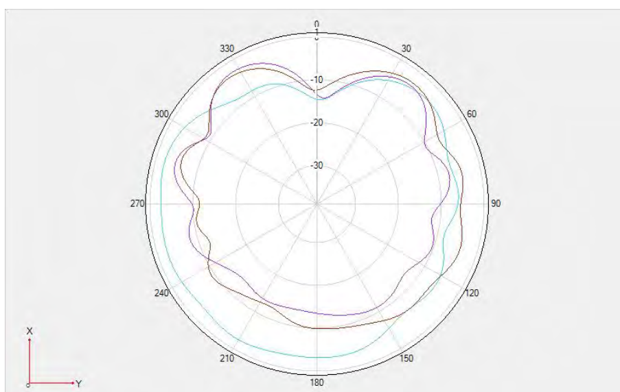
Unfold- NR n38/41DRX1 theta =90
