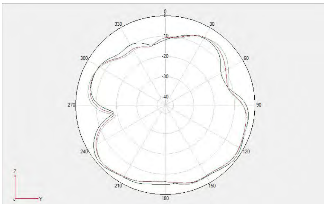
Unfold- DCS/WCDMA B4/ LTE B3/B4/B66/N3/N66 \Phi=90\text{deg}
