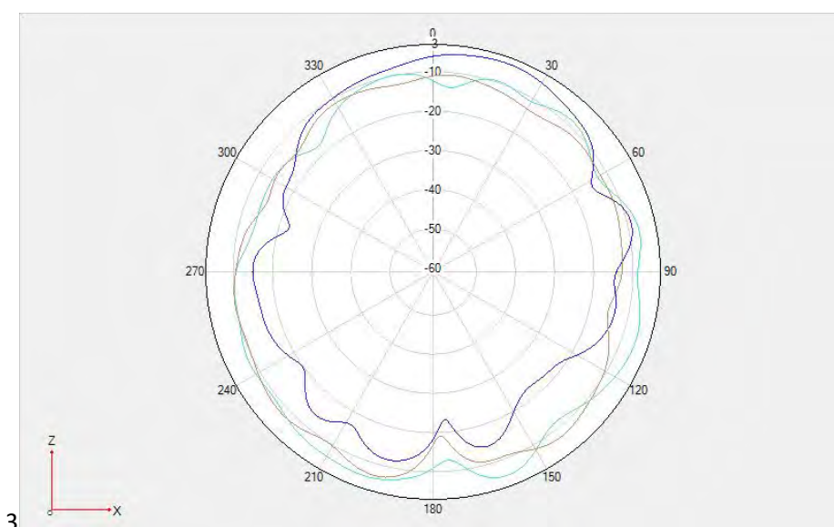
Unfold- NR n77/78/79 DRX3 theta =90
