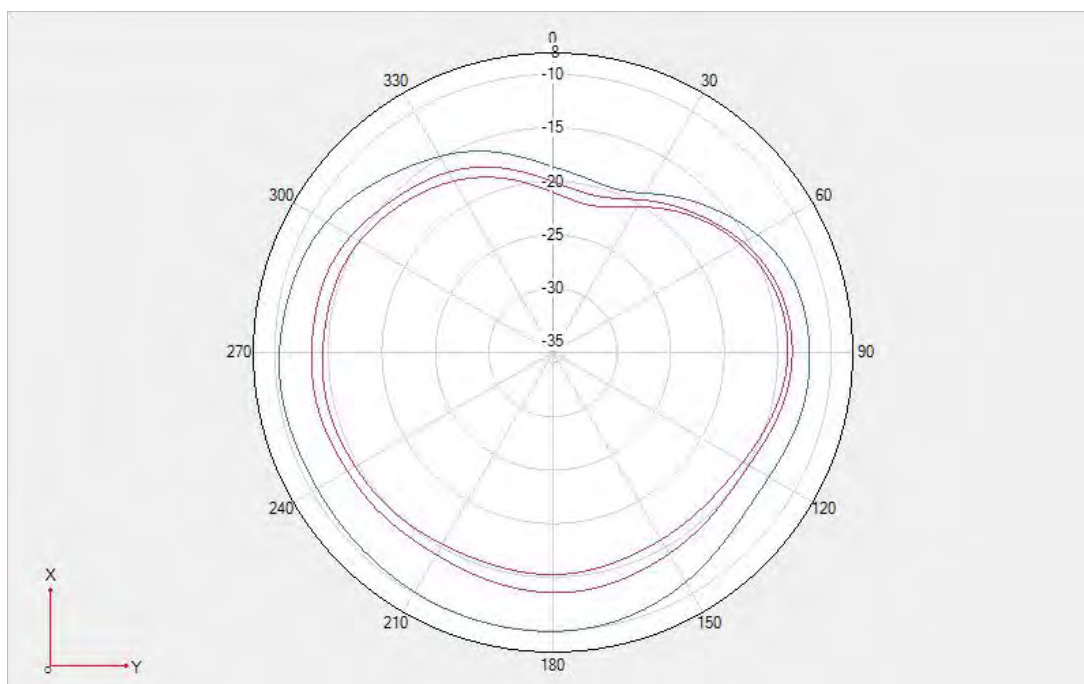
Unfold-DPDT SWAP:GSM 900/WCDMA B8/LTE B8 \Theta=90^\circ
