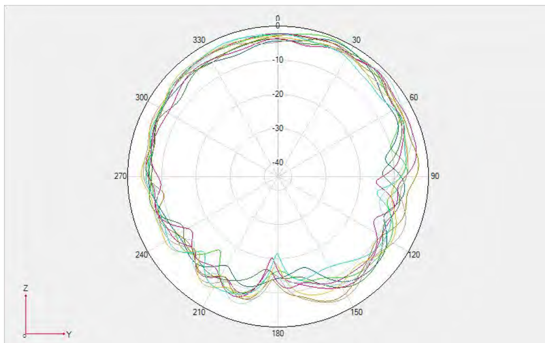
Unfold- N77/N78 \Phi=90\text{deg}
