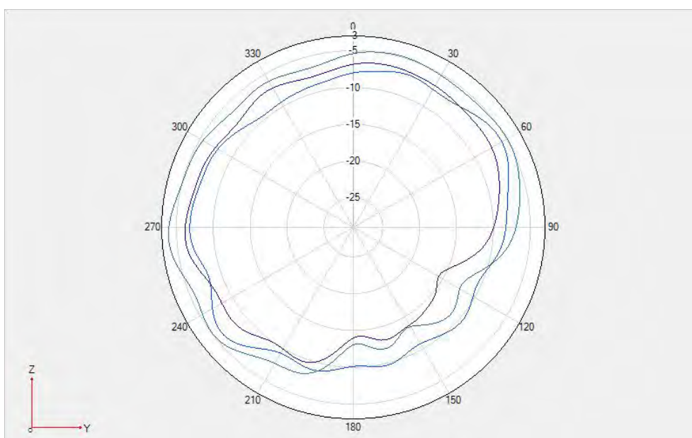
Unfold-Lte B28/N28 \Phi = 90^\circ
