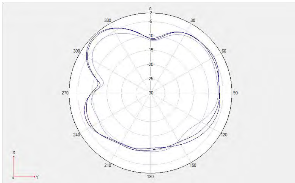
Unfold-Wifi Miomo 0-2.4G \Theta=90^\circ
