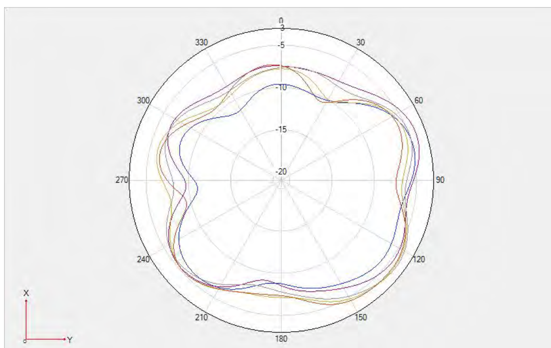
Unfold- LTE B38/41 N38/41 \Theta = 90^\circ
