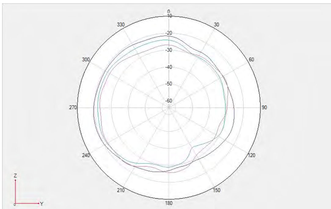
Fold- DPDT SWAP LTE B20/N20 Phi=90deg
