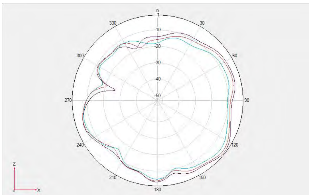
Fold- DCS/WCDMA B4/ LTE B3/B4/B66/N3/N66 \Phi=0^\circ
