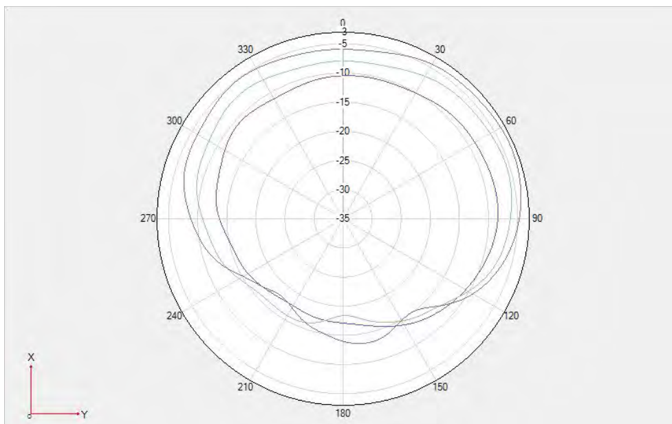
Unfold-LTE B5/B20N20 \Theta = 90^\circ
