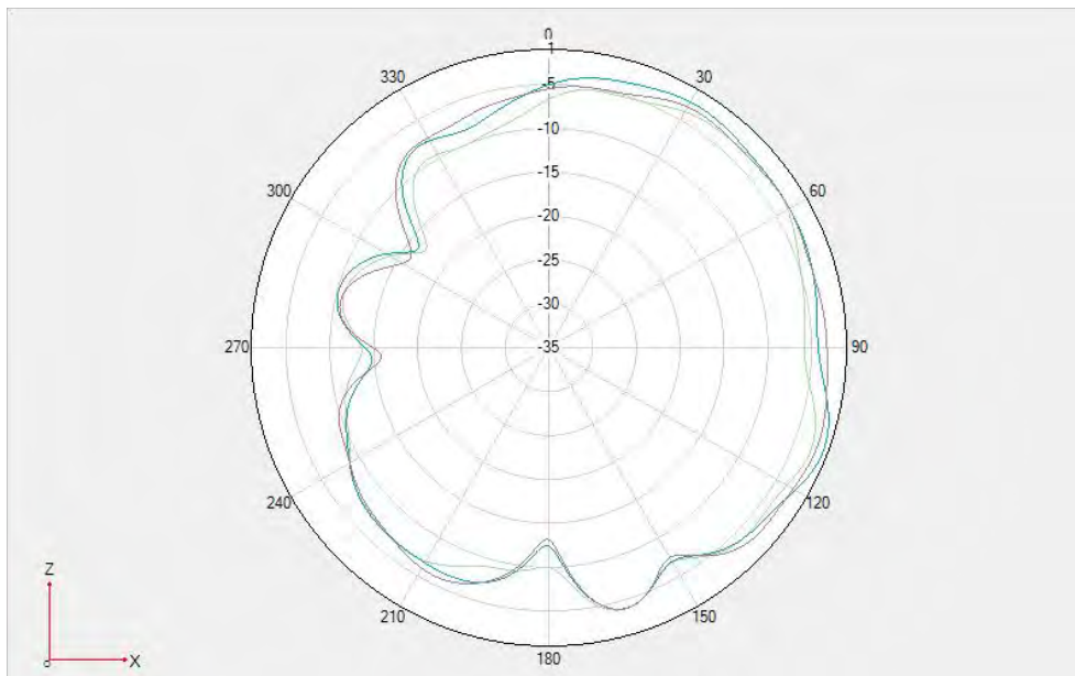
Unfold-Wifi Miomo 1-2.4G \Phi=0\text{deg}
