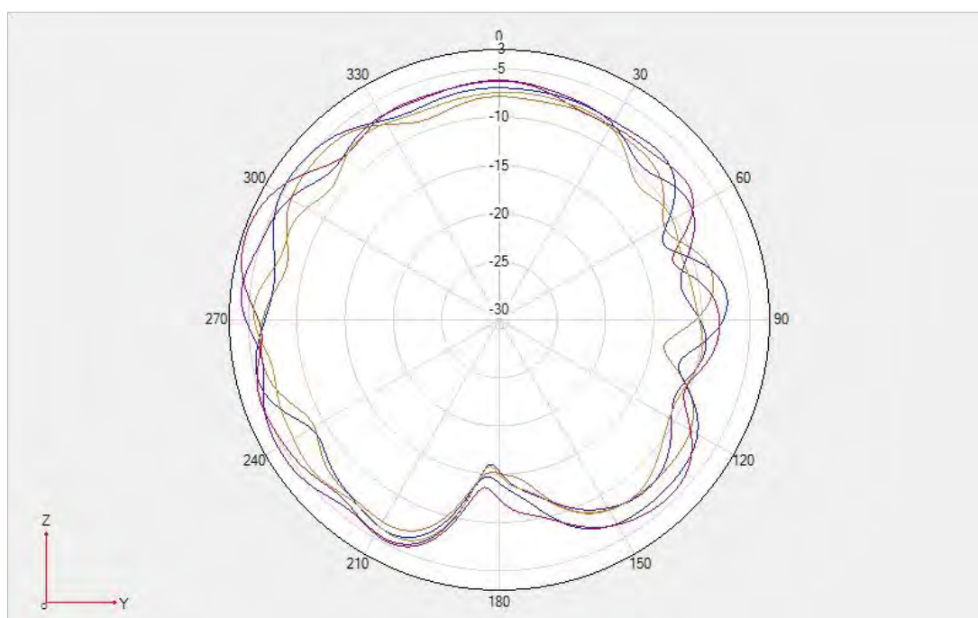
Fold- LTE B38/41 N38/41 \Phi=90^\circ
