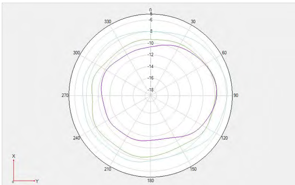
Fold-Lte B28/N28 \Theta = 90^\circ
