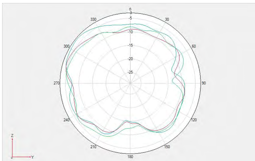
Fold- LTE B40/N40 \Phi=90^\circ
