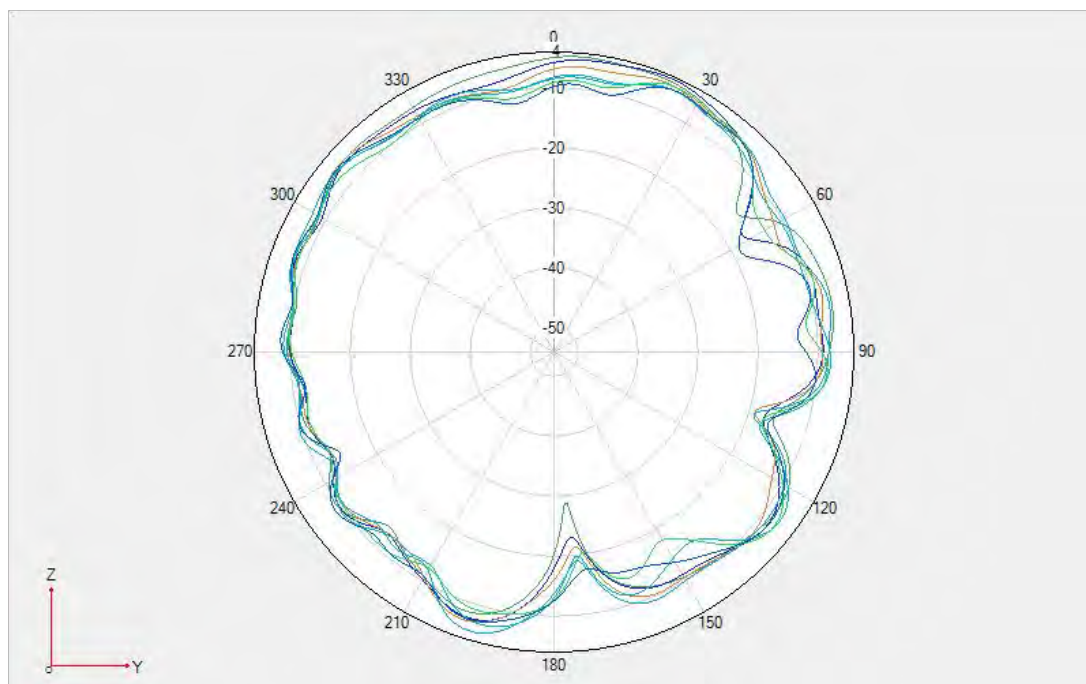
Unfold- N79 \Phi=90^\circ
