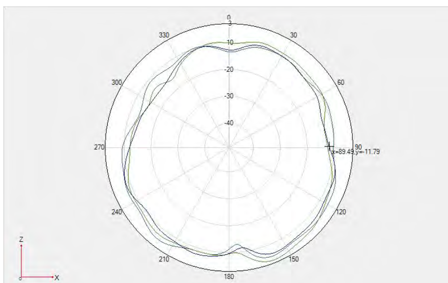
Unfold- NR n38/41 DRX3 \theta = 90
