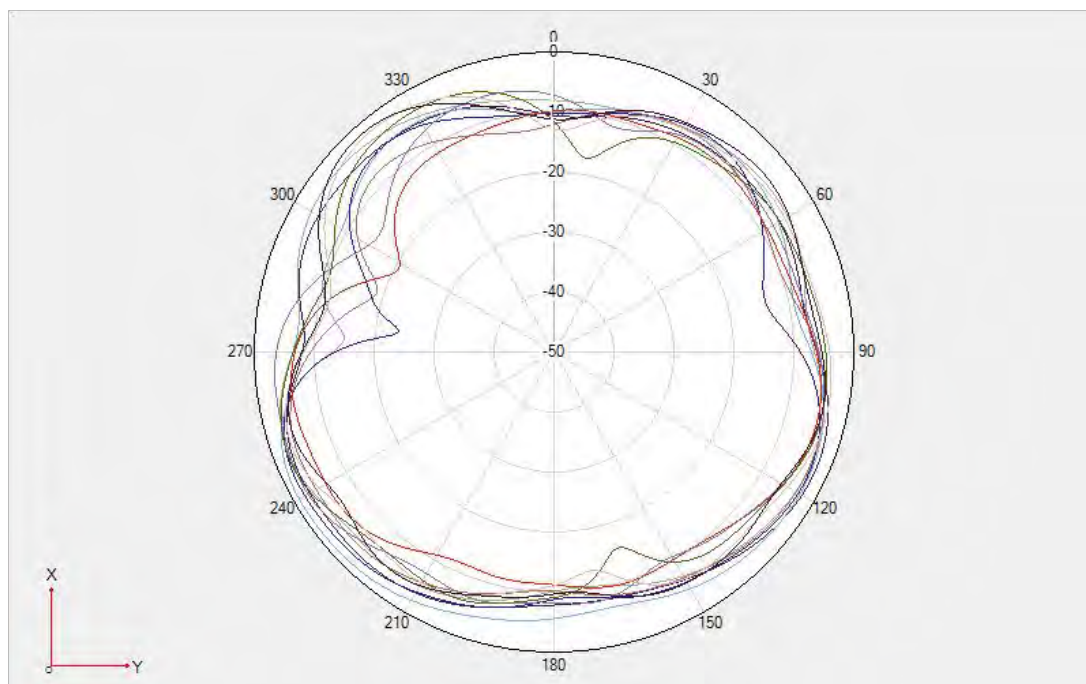
Unfold- N77/N78 \Theta=90\text{deg}
