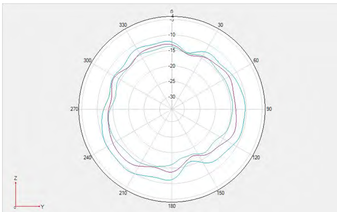
Unfold-DPDT SWAP:GSM 900/WCDMA B8/LTE B8 \Phi=90^\circ
