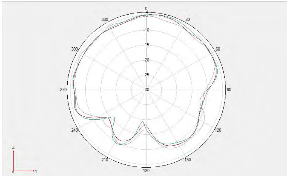
Unfold-Wifi Miomo0-2.4G \Phi = 90^\circ
