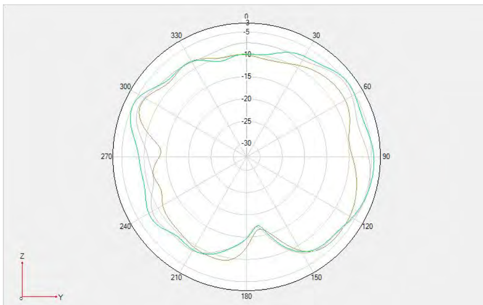
Fold-Wifi Miomo1-2.4G \Phi = 90^\circ
