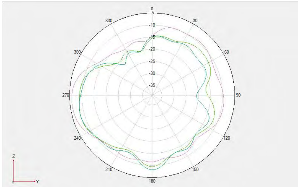
Fold-GSM 900/WCDMA B8/LTE B8 \Phi=90\text{deg}
