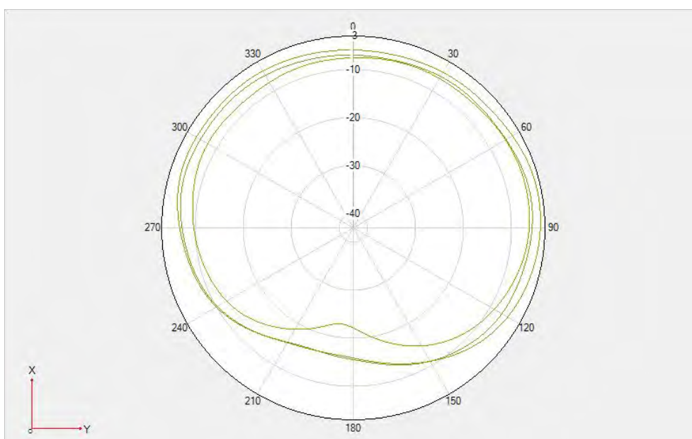
Unfold-Lte B28 \Theta=90^\circ
