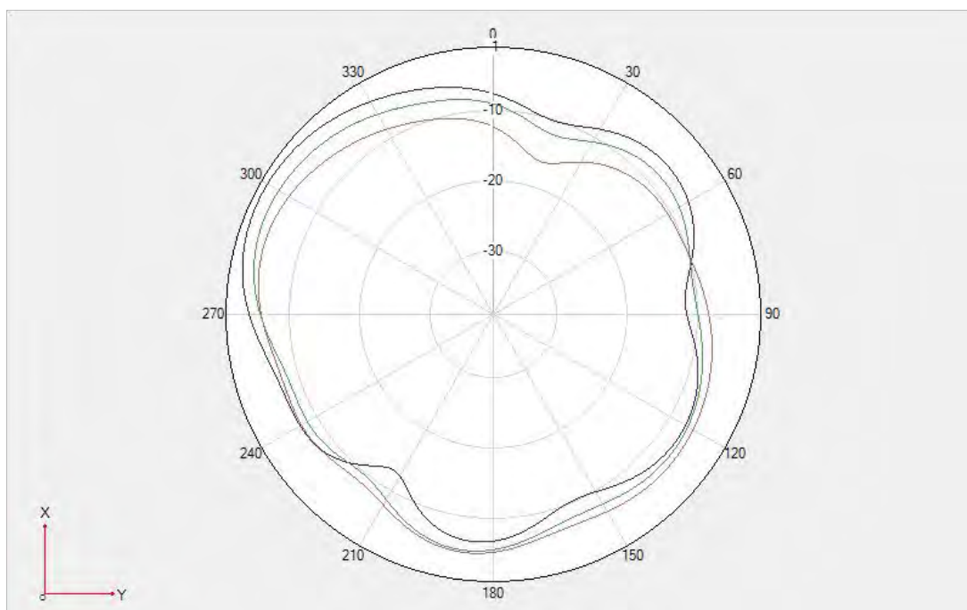
Unfold- DCS/WCDMA B4/ LTE B3/B4/B66/N3/N66 \Theta=90\text{deg}
