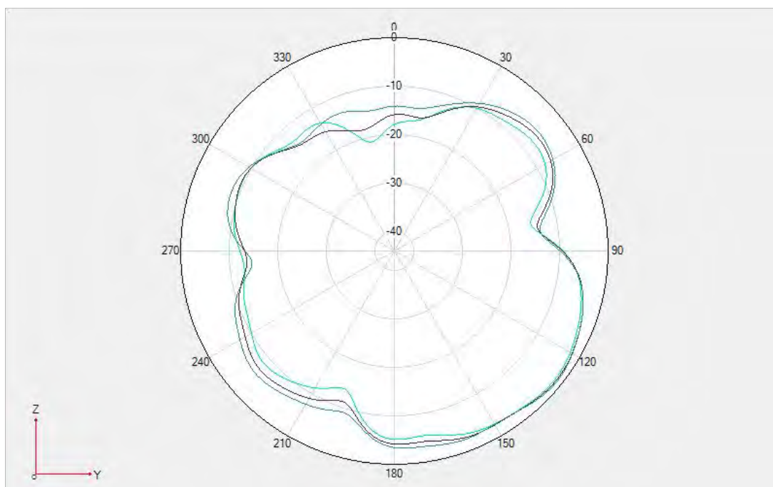
Fold- DCS/WCDMA B4/ LTE B3/B4/B66/N3/N66 \Phi=90^\circ
