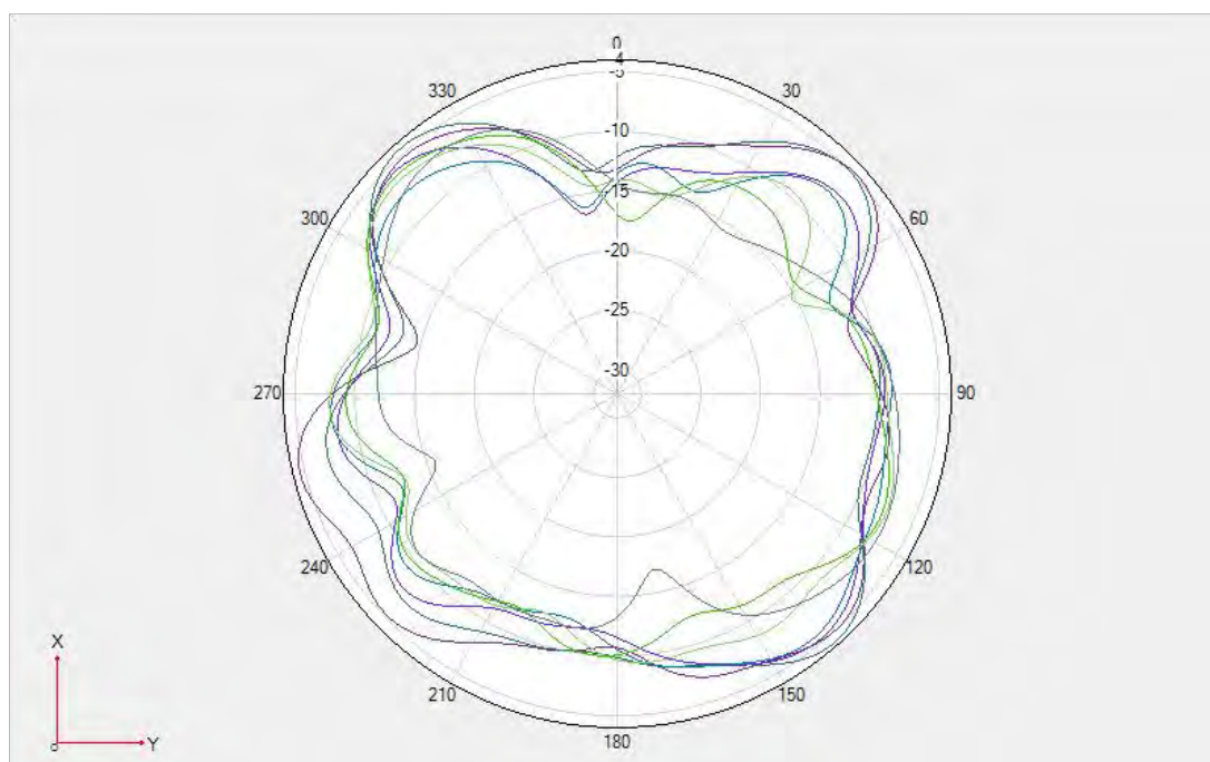
Unfold- N79 \Theta=90^\circ
