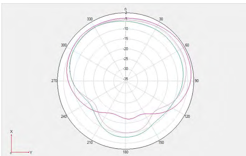
Unfold-GSM 900/WCDMA B8/LTE B8 \Theta=90^\circ
