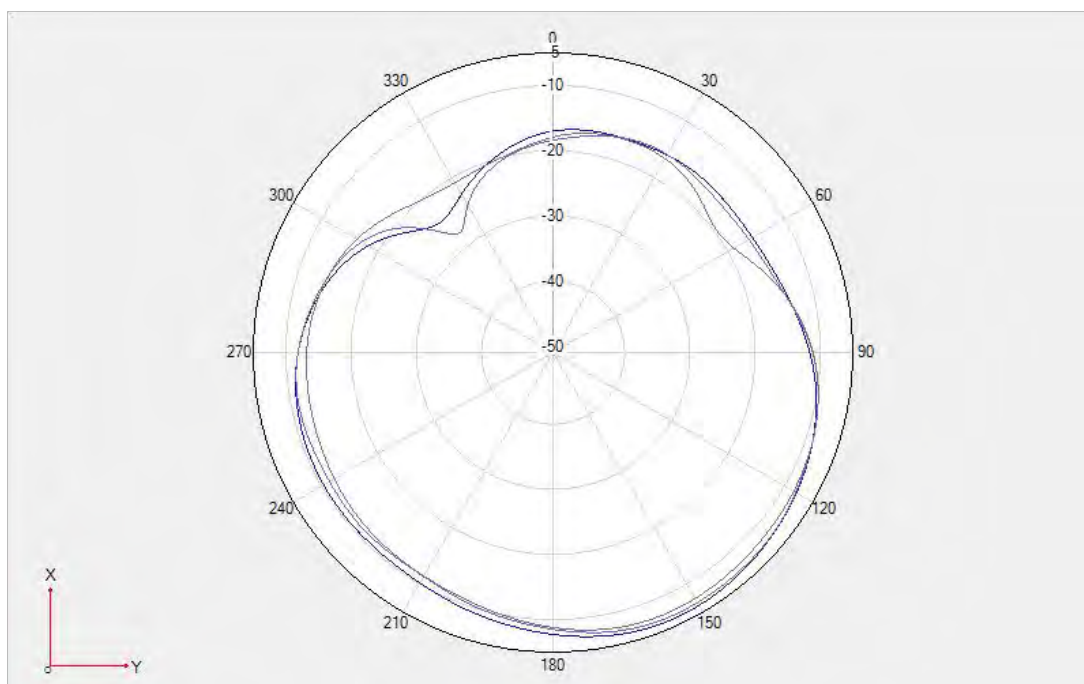
Fold- WCDMA B1/LTE B1 \Theta = 90^\circ
