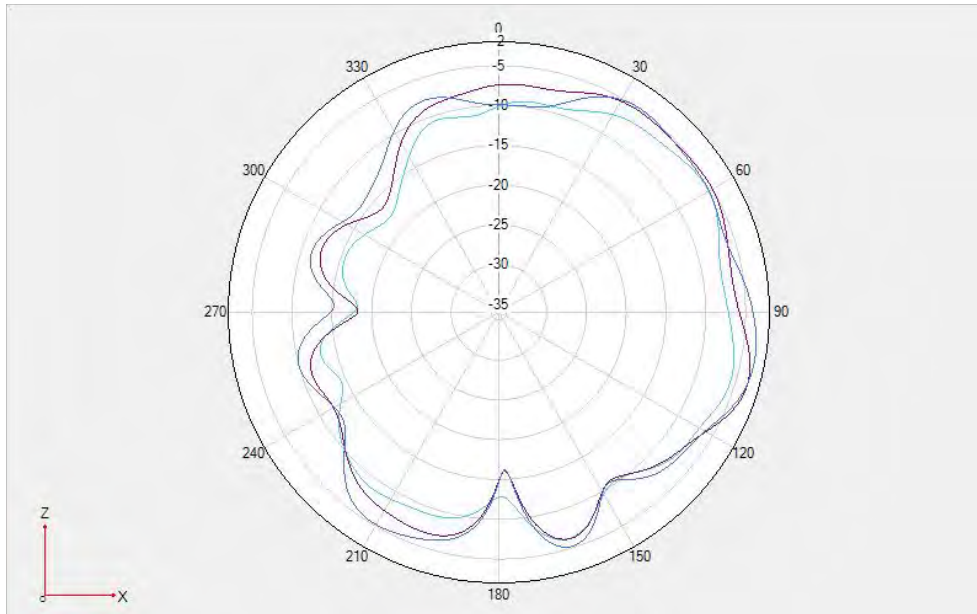
Fold-Wifi Miomo1-2.4G \Phi = 0^\circ
