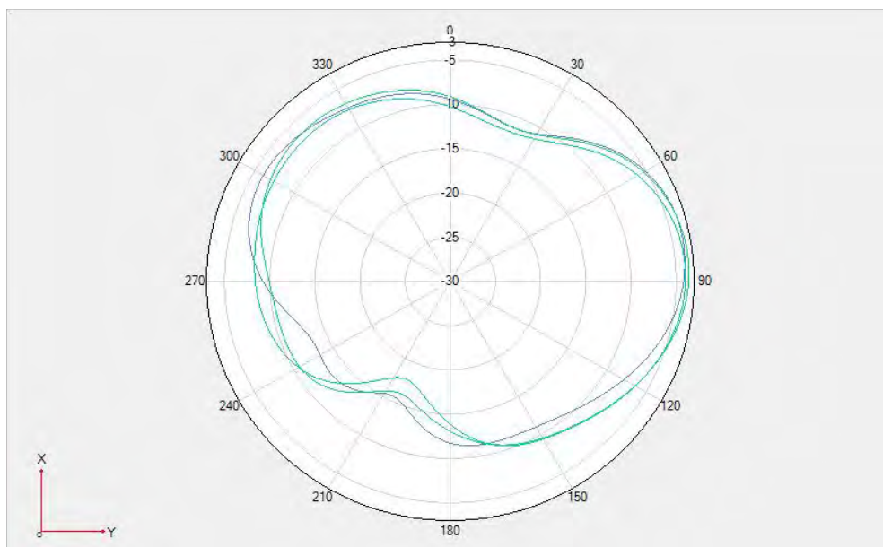
Fold-Wifi Miomo0-2.4G \Theta = 90^\circ
