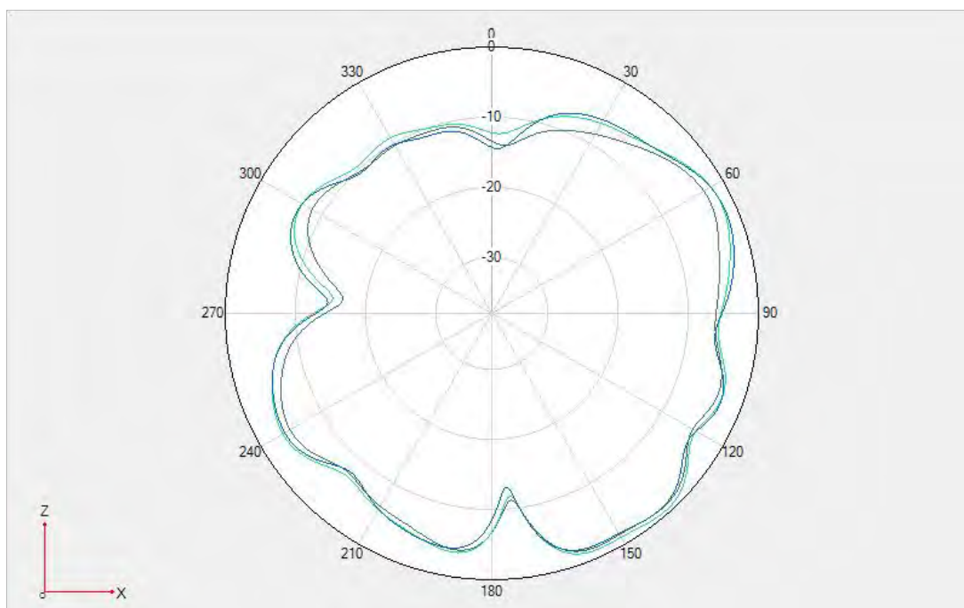
Unfold- PCS/WCDMA B2/LTE B2 \Phi = 0^\circ
