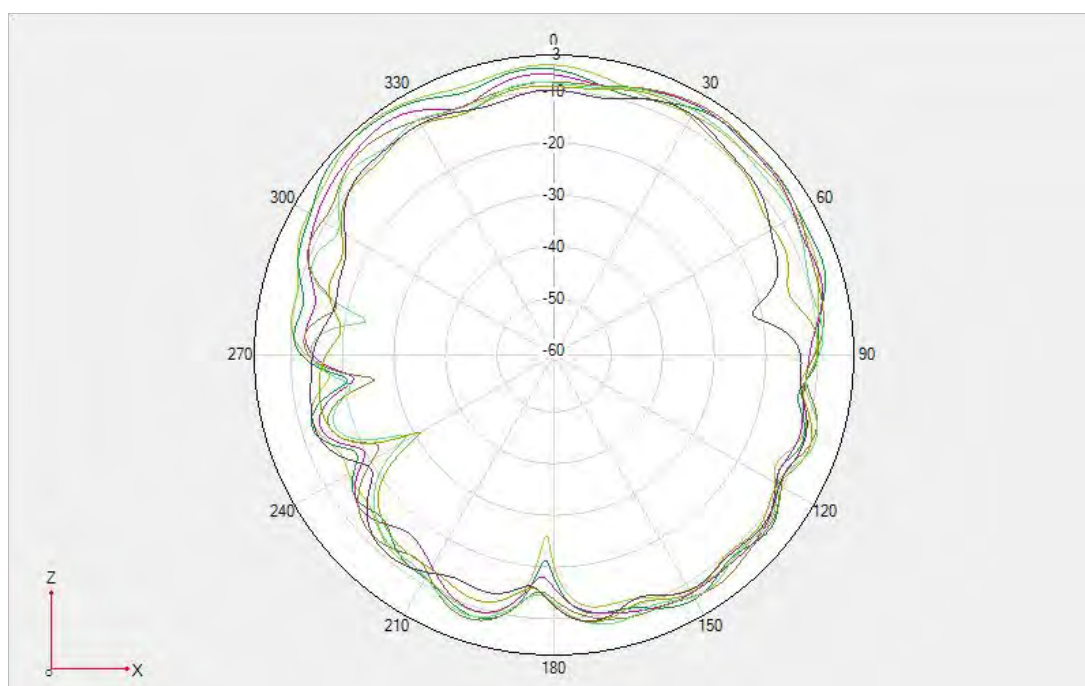
Unfold- N79 \Phi = 0^\circ
