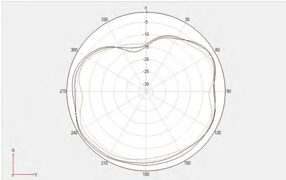
Unfold-Wifi Miomo 1-2.4G \Theta=90\text{deg}
