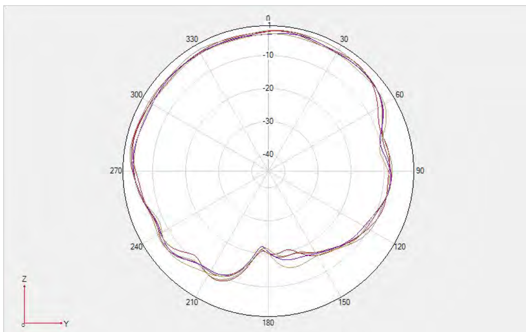
Unfold- LTE B40/N40 \Phi = 90^\circ
