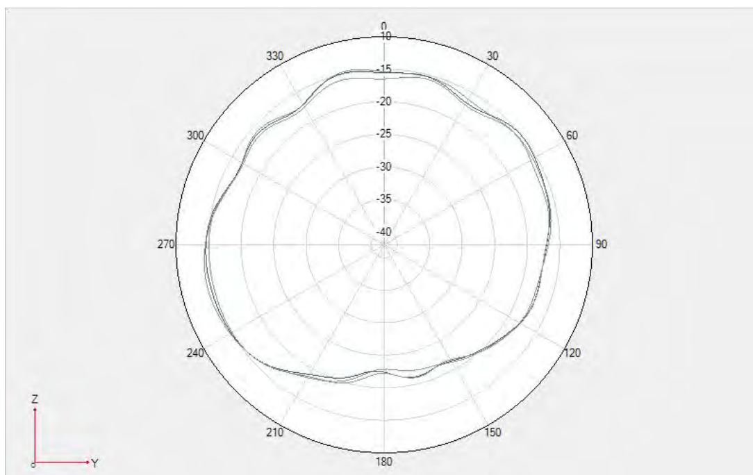
Unfold-DPDT SWAP N71 \Phi=90^\circ
