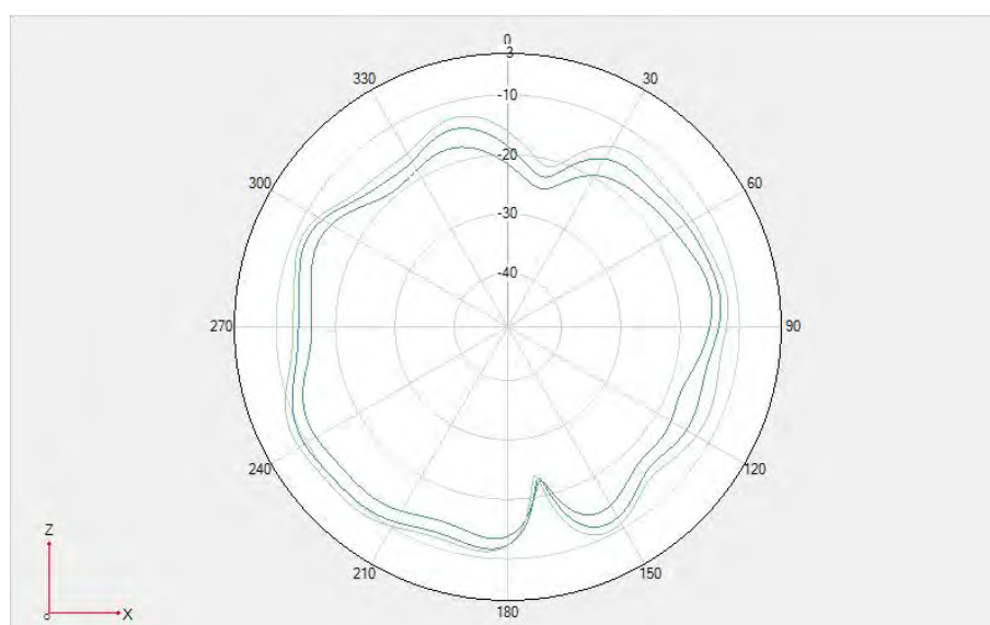
Unfold- NR n3/N66 DRX \theta = 90
