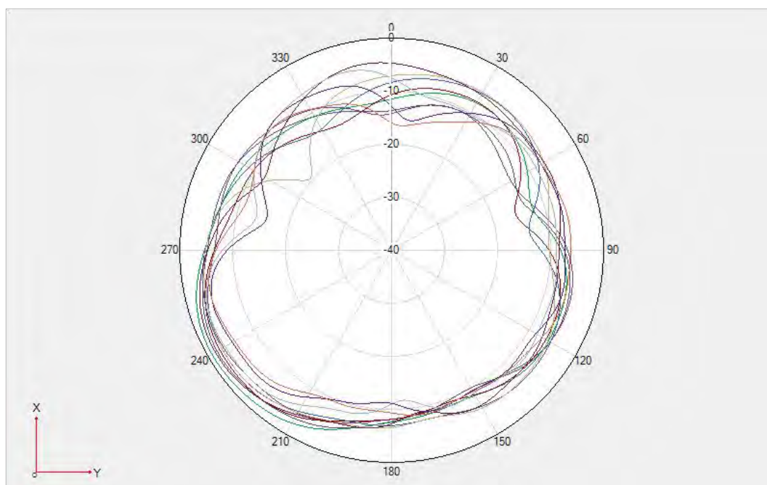
Fold- N77/N78 \Theta = 90^\circ
