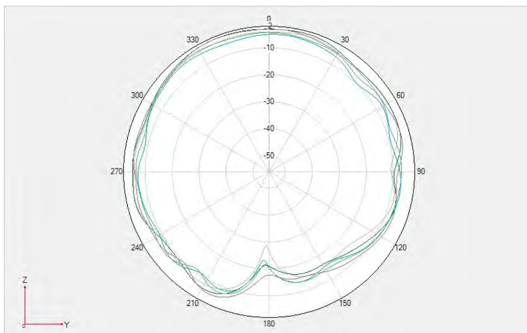
Unfold- LTE B38/41 N38/41 \Phi = 90^\circ
