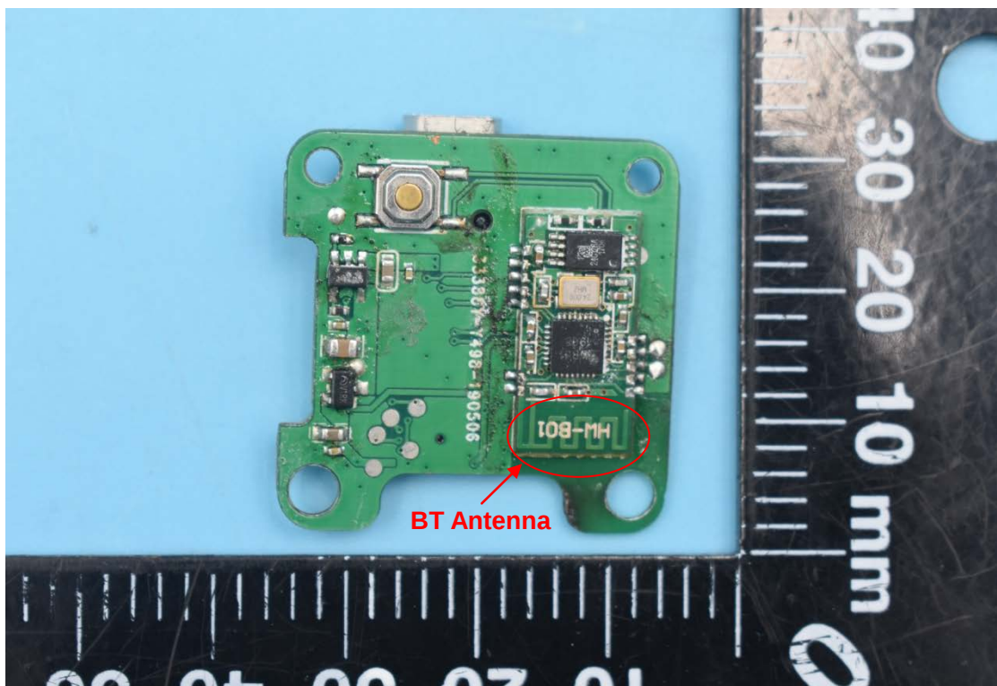
2. Antenna view
