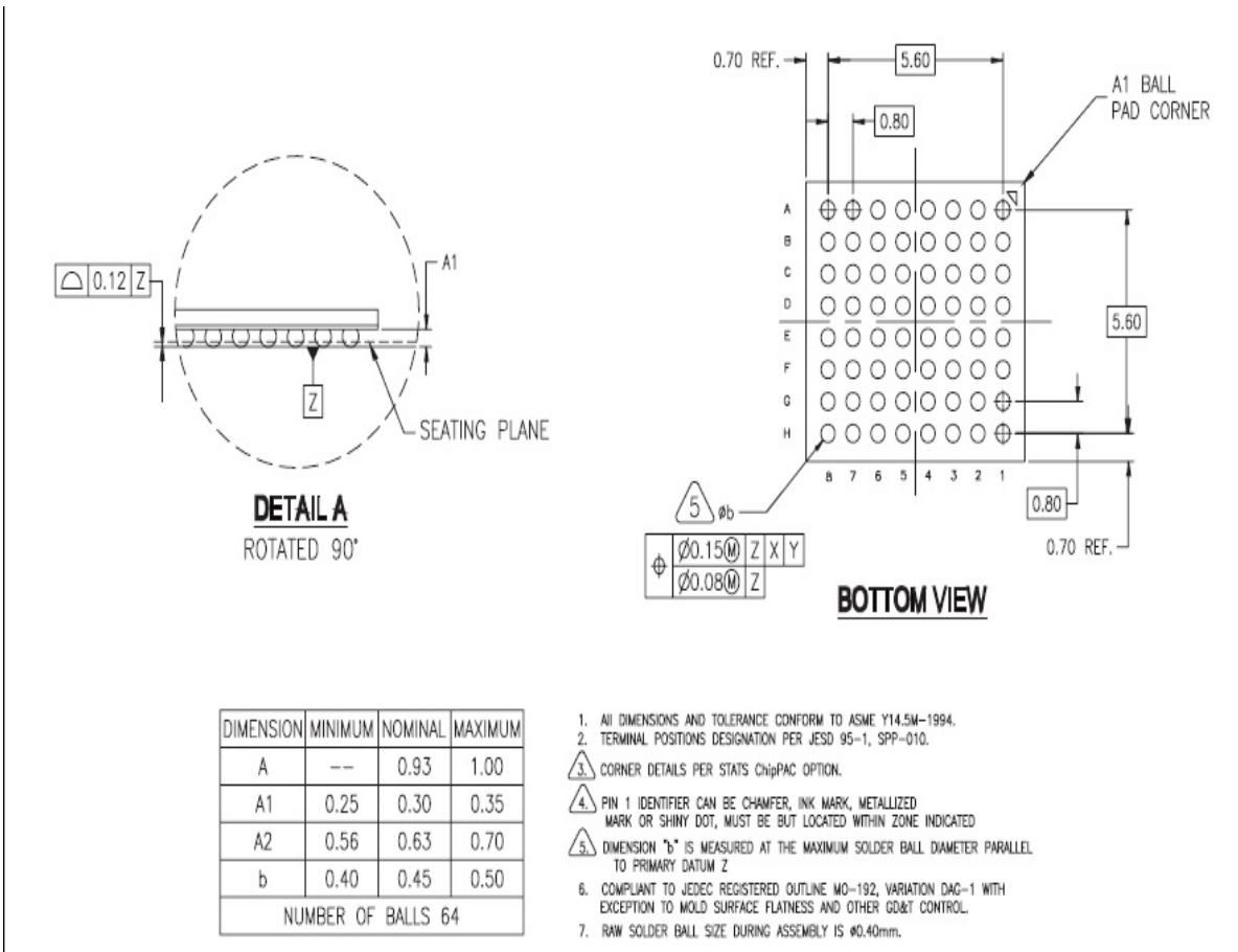
Figure 7: 64Pin FBGA Package
