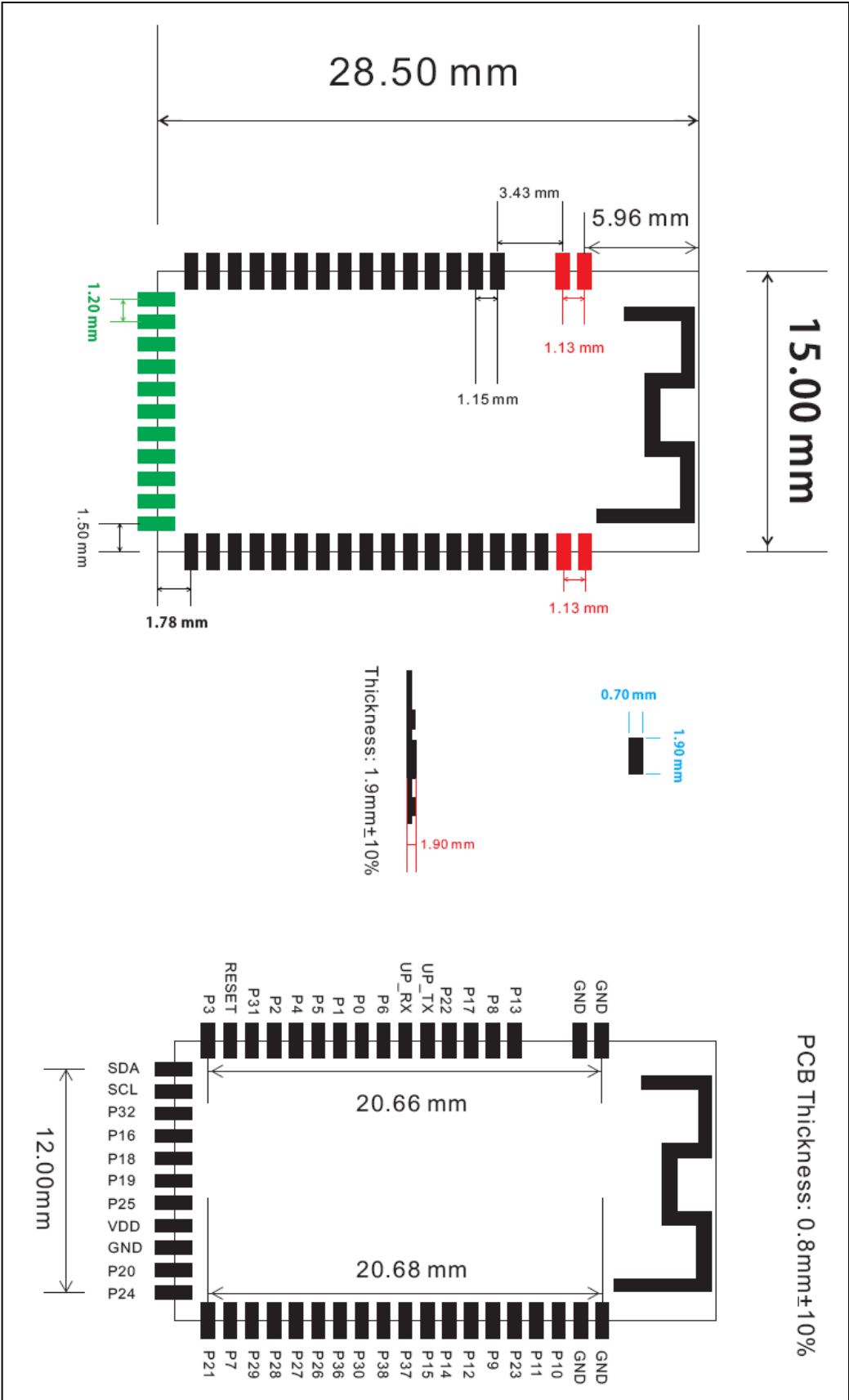
Figure 5: 47Pin-Bluetooth Module
