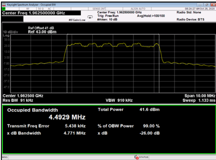
Figure 539: 16QAM 5MHz B.W.; 1962.5MHz, 15kHz - Output
