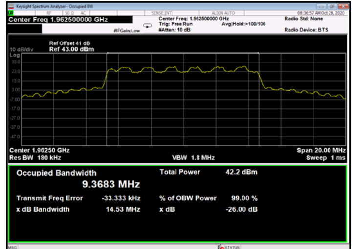
Figure 546: 16QAM 10MHz B.W.; 1962.5MHz, 15kHz - Output
