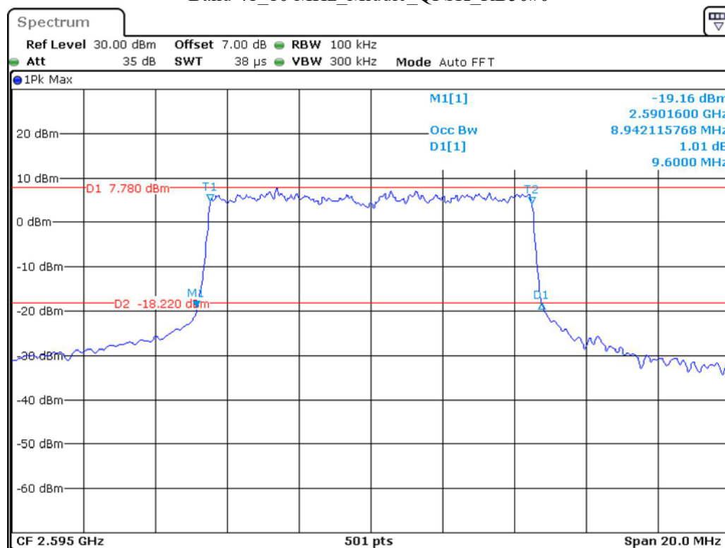
Band 41 10 MHz Middle QPSK RB50#0
