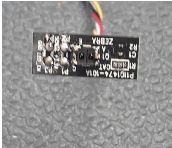
Sensor Board 1 Top
