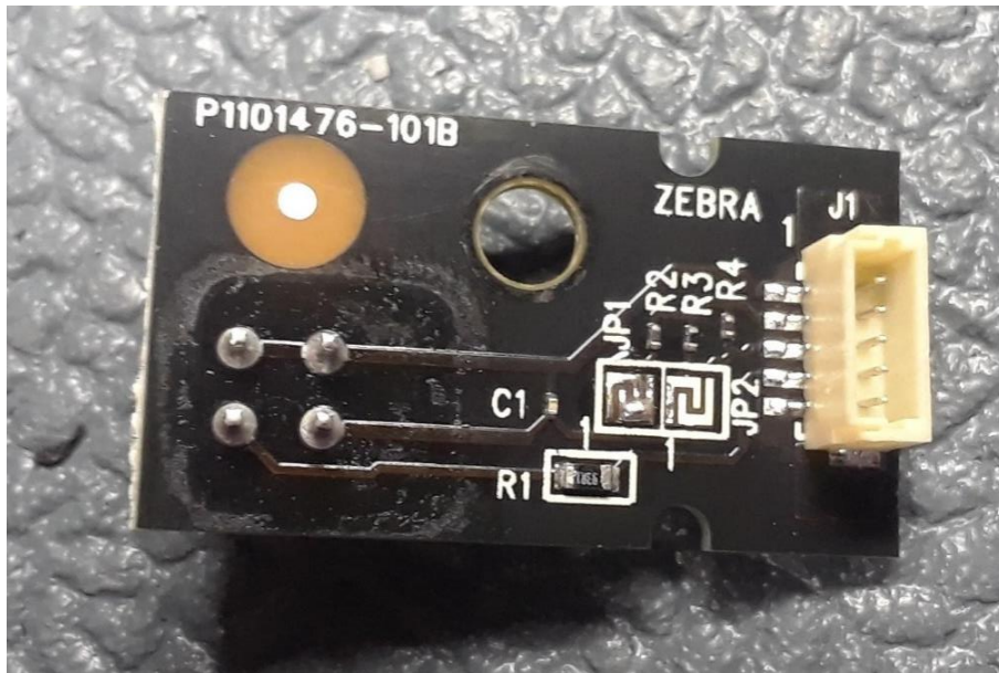
Sensor Board 3 Bottom
