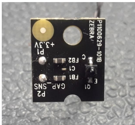
Sensor Board 2 Top
