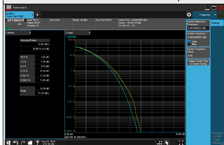
256QAM CH 631000 (3465 MHz)
