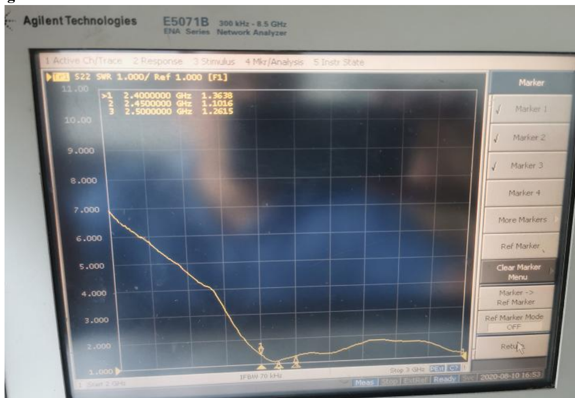
RC905 antenna VSWR
