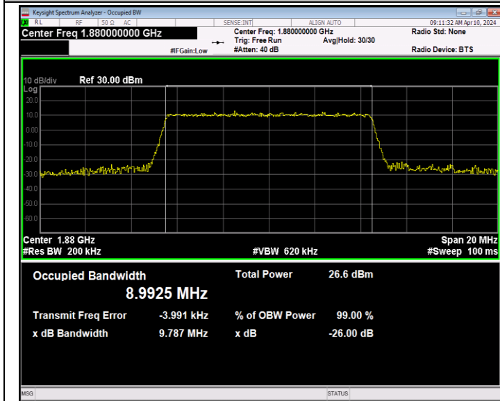
Band2-10MHz-64QAM-18900-50RB#0-PASS
