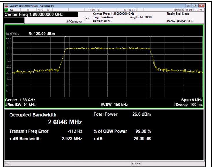
Band2-3MHz-16QAM-18900-15RB#0-PASS
