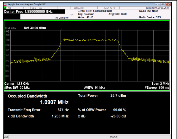
Band2-1.4MHz-64QAM-18900-6RB#0-PASS
