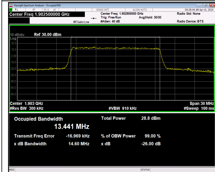
Band2-15MHz-QPSK-19125-75RB#0-PASS
