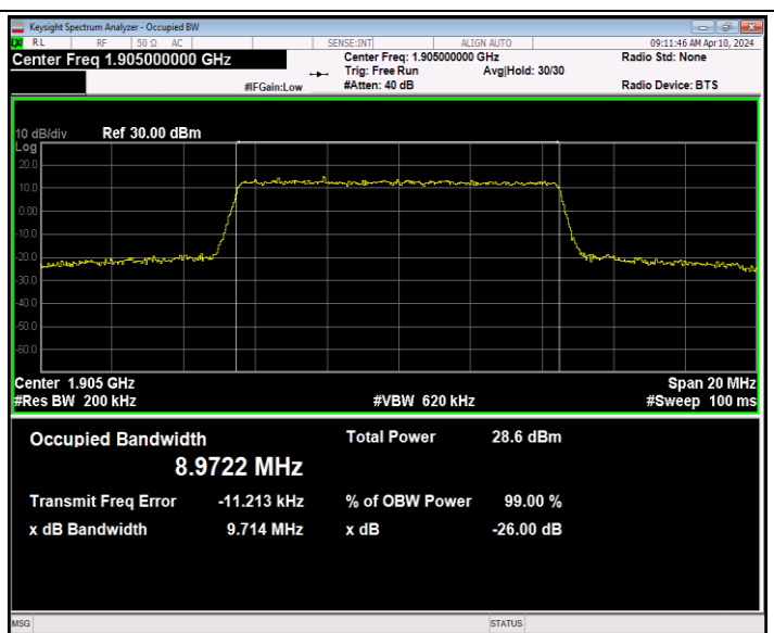
Band2-10MHz-QPSK-19150-50RB#0-PASS
