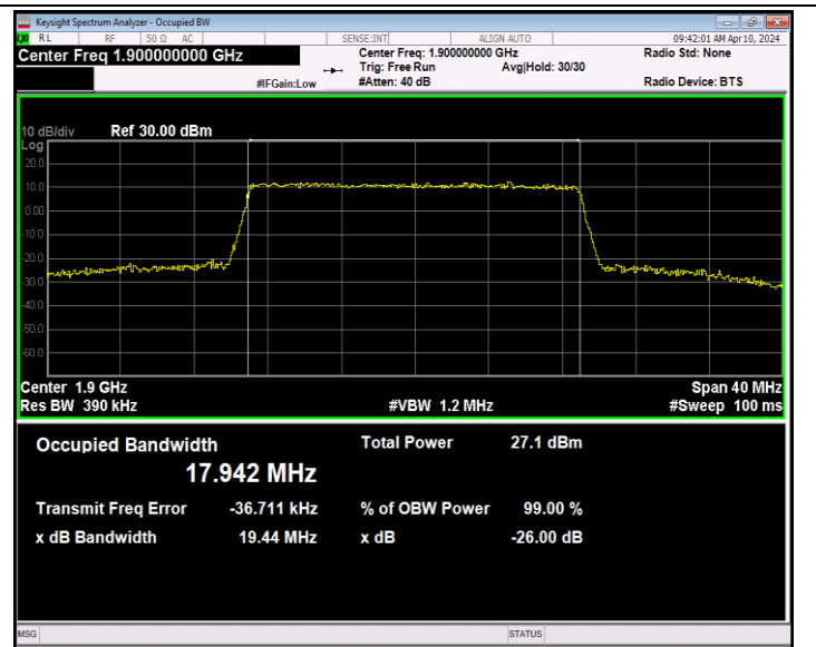
Band2-20MHz-64QAM-19100-100RB#0-PASS
