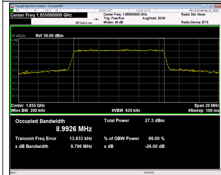
Band2-10MHz-16QAM-18650-50RB#0-PASS
