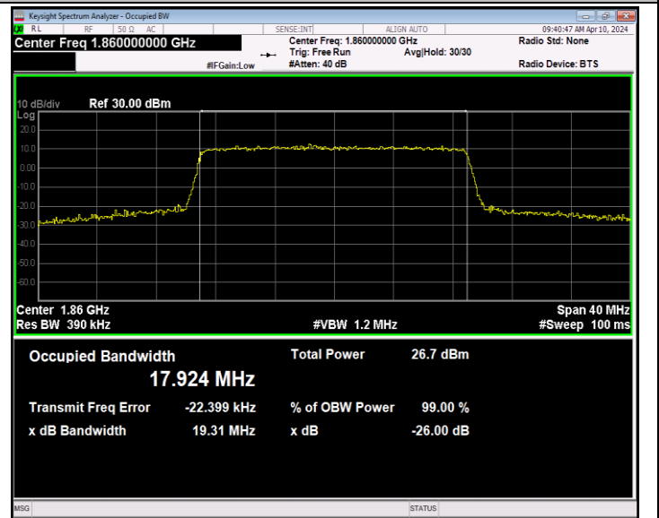
Band2-20MHz-64QAM-18700-100RB#0-PASS
