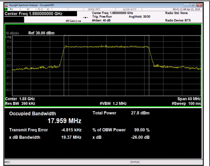
Band2-20MHz-16QAM-18900-100RB#0-PASS
