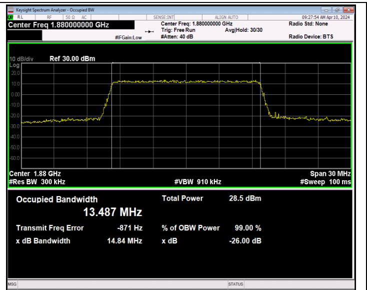
Band2-15MHz-QPSK-18900-75RB#0-PASS
