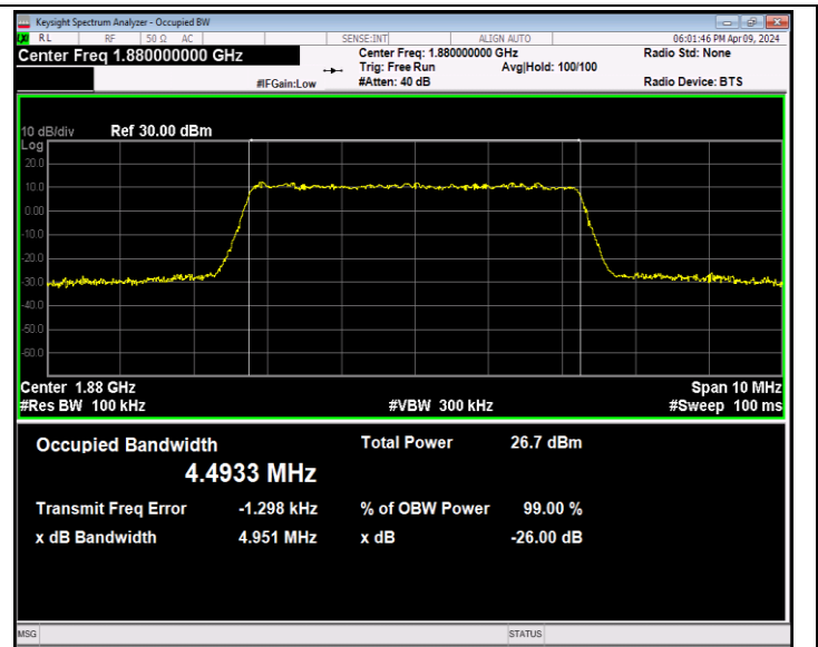
Band2-5MHz-64QAM-18900-25RB#0-PASS
