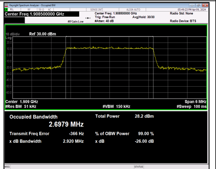
Band2-3MHz-QPSK-19185-15RB#0-PASS
