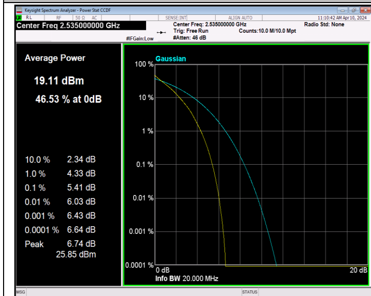
Band7-20MHz-QPSK-21100-100RB#0-PASS
