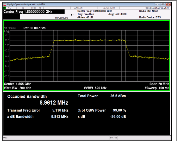
Band2-10MHz-64QAM-18650-50RB#0-PASS
