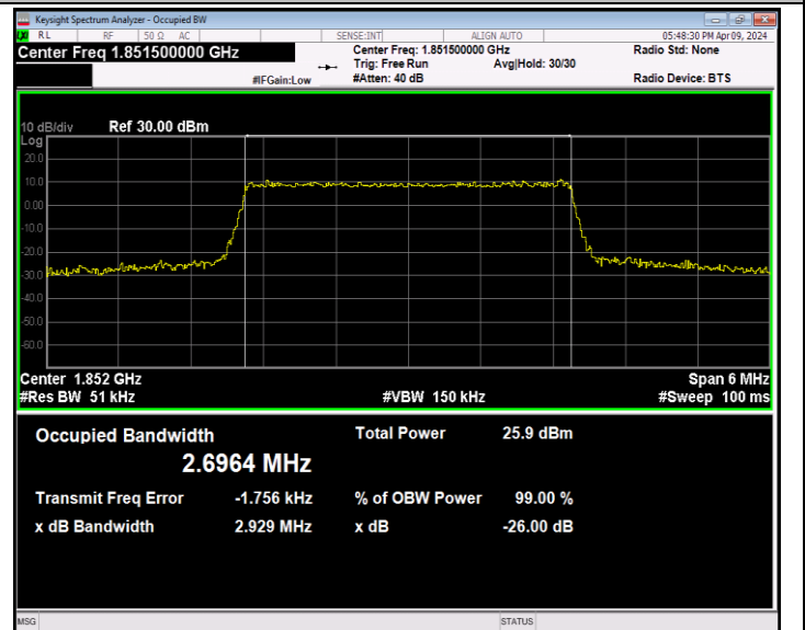
Band2-3MHz-64QAM-18615-15RB#0-PASS
