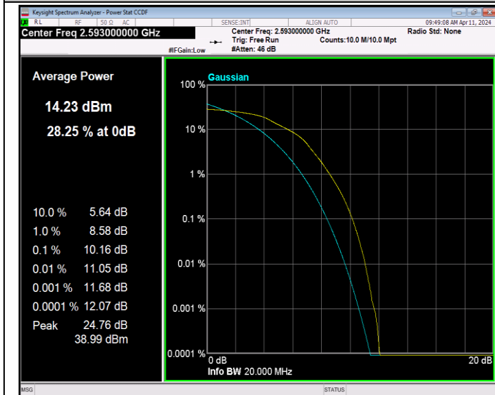
Band41-20MHz-16QAM-40620-100RB#0-PASS
