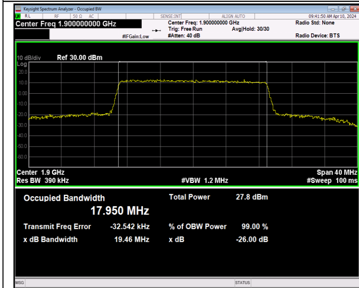
Band2-20MHz-16QAM-19100-100RB#0-PASS
