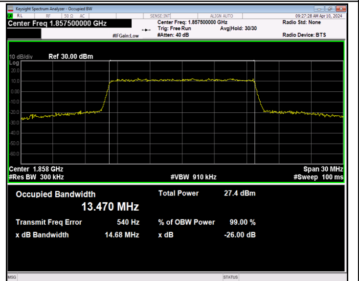
Band2-15MHz-16QAM-18675-75RB#0-PASS
