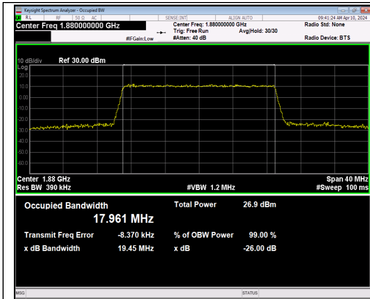
Band2-20MHz-64QAM-18900-100RB#0-PASS
