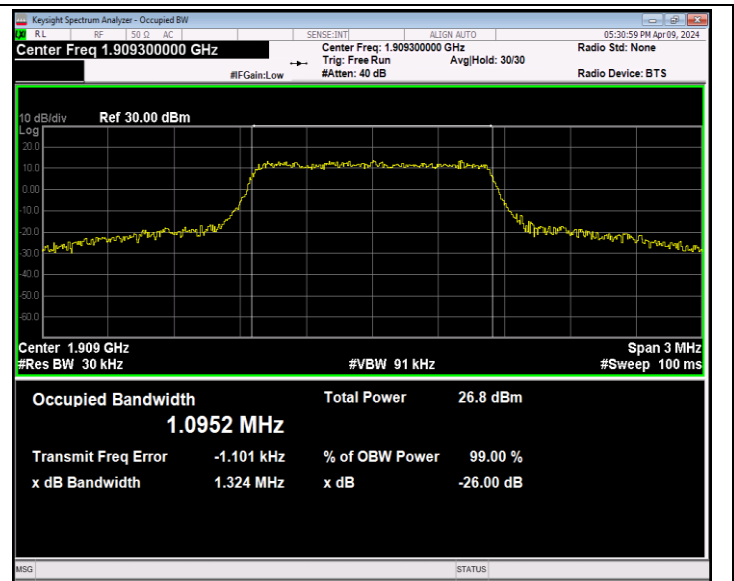
Band2-1.4MHz-16QAM-19193-6RB#0-PASS
