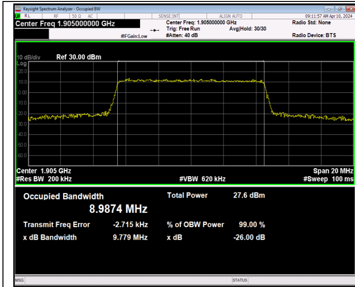
Band2-10MHz-16QAM-19150-50RB#0-PASS
