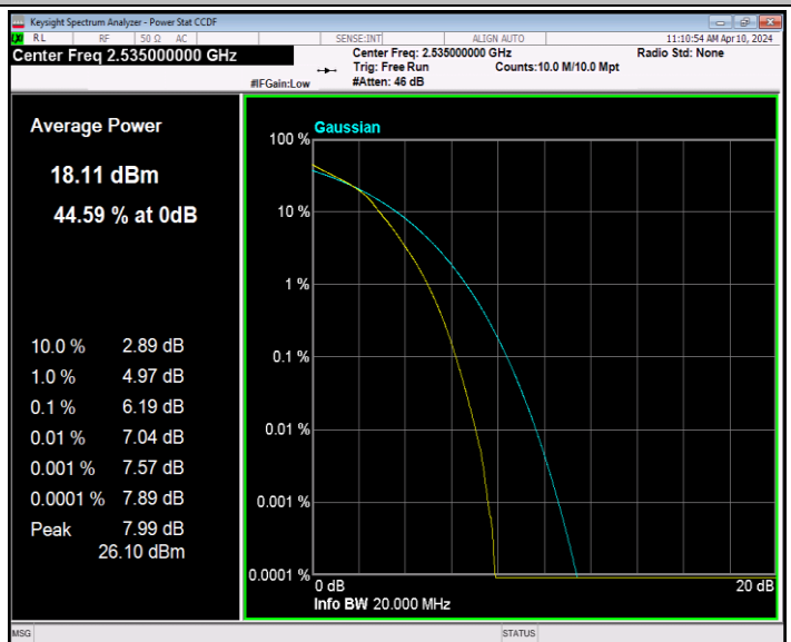
Band7-20MHz-16QAM-21100-100RB#0-PASS
