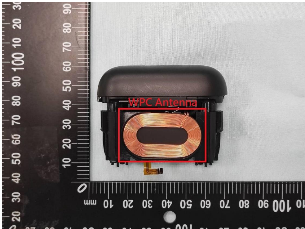
(33) EUT Photo_ Charging Case
