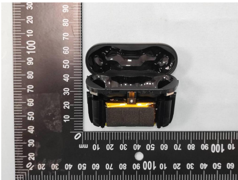
(24) EUT Photo_ Charging Case
