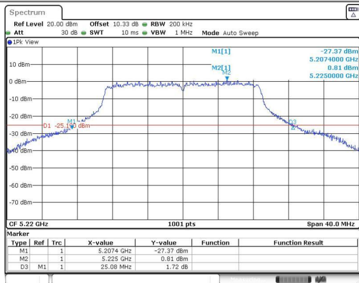
11AC20SISO_Ant1_5220
