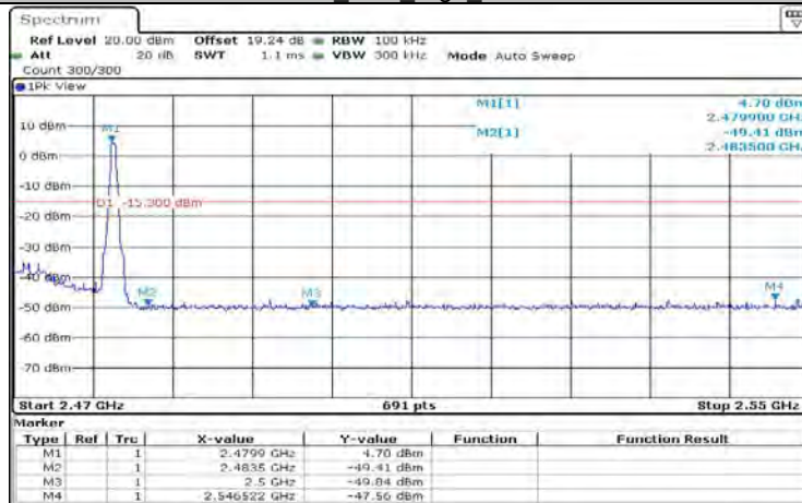
DH1_Ant1_High_2480
