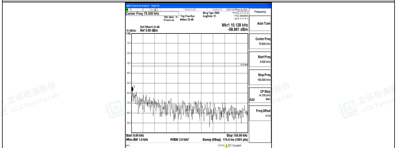
Band17_10MHz_16QAM_23780_1RB#0_0.009~0.15_0.009~0.15
