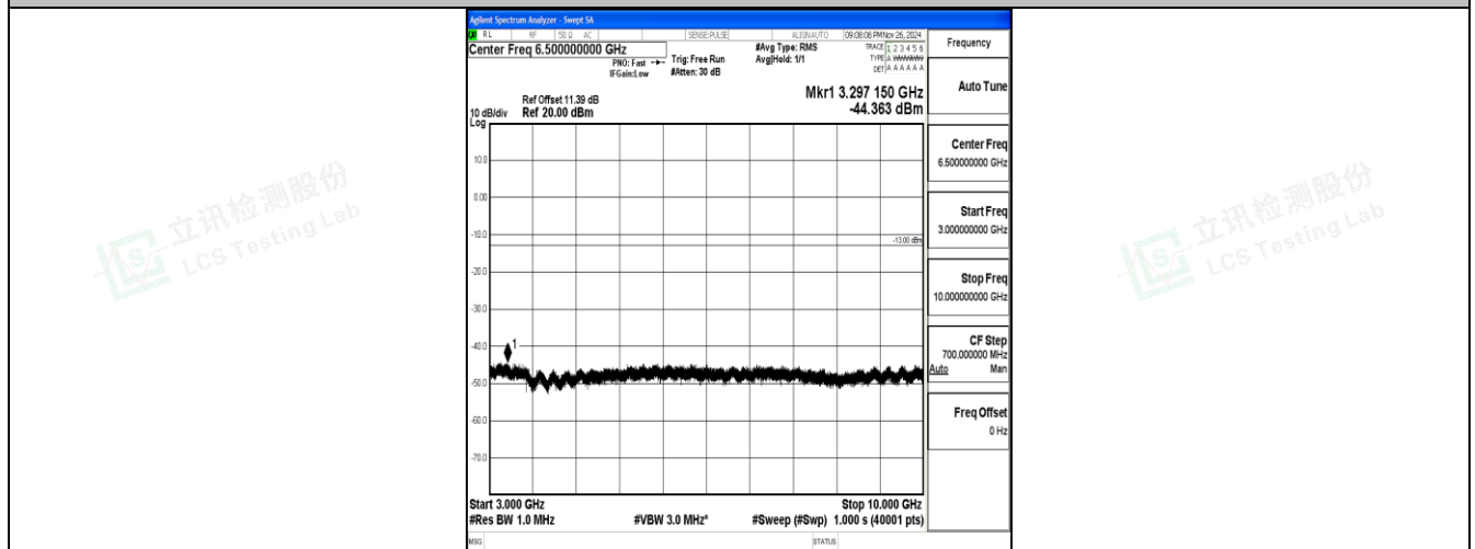
Band17_10MHz_16QAM_23780_1RB#0_3000~10000_3000~10000
