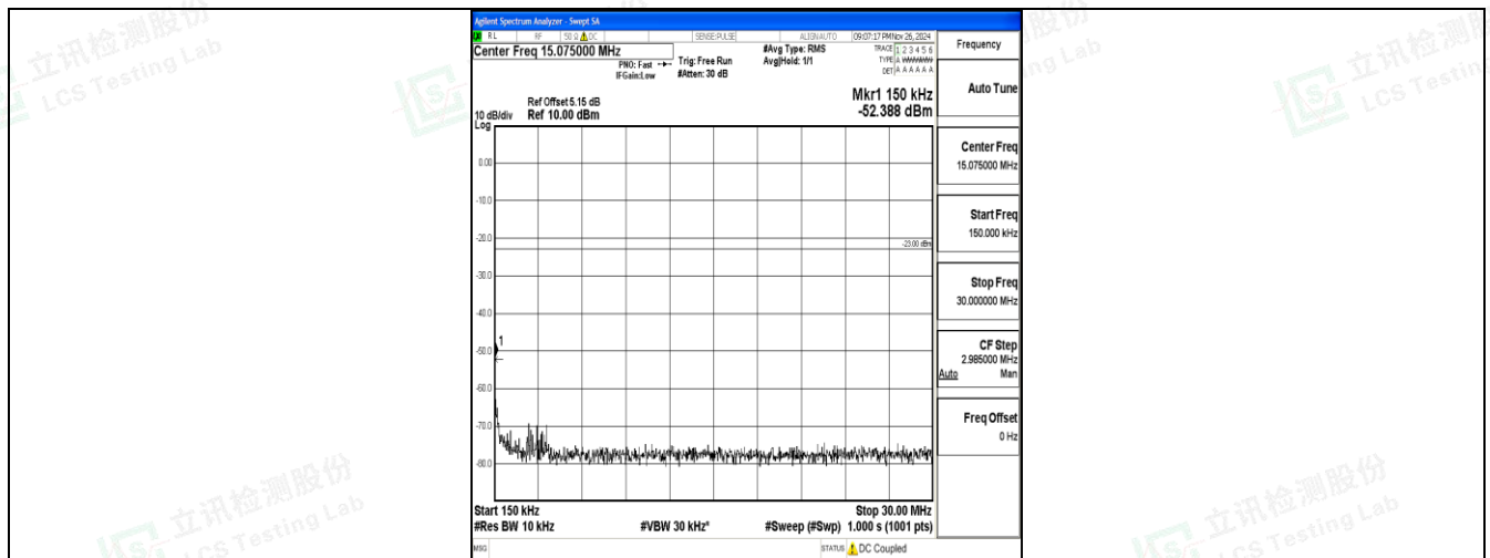
Band17_10MHz_QPSK_23780_1RB#0_0.15~30_0.15~30
