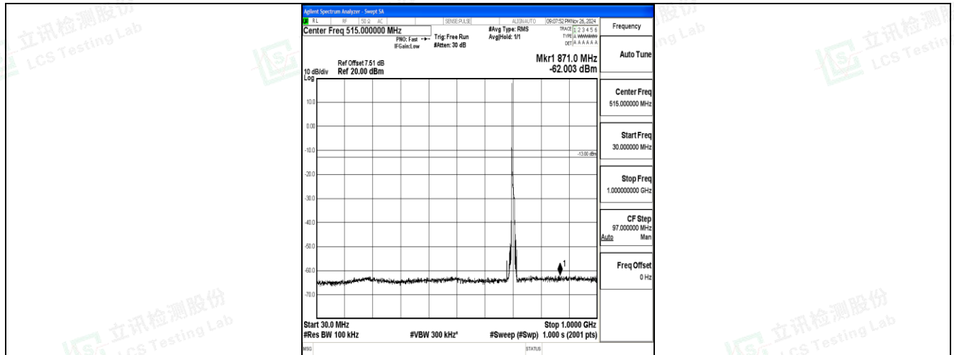
Band17_10MHz_16QAM_23780_1RB#0_30~1000_30~1000
