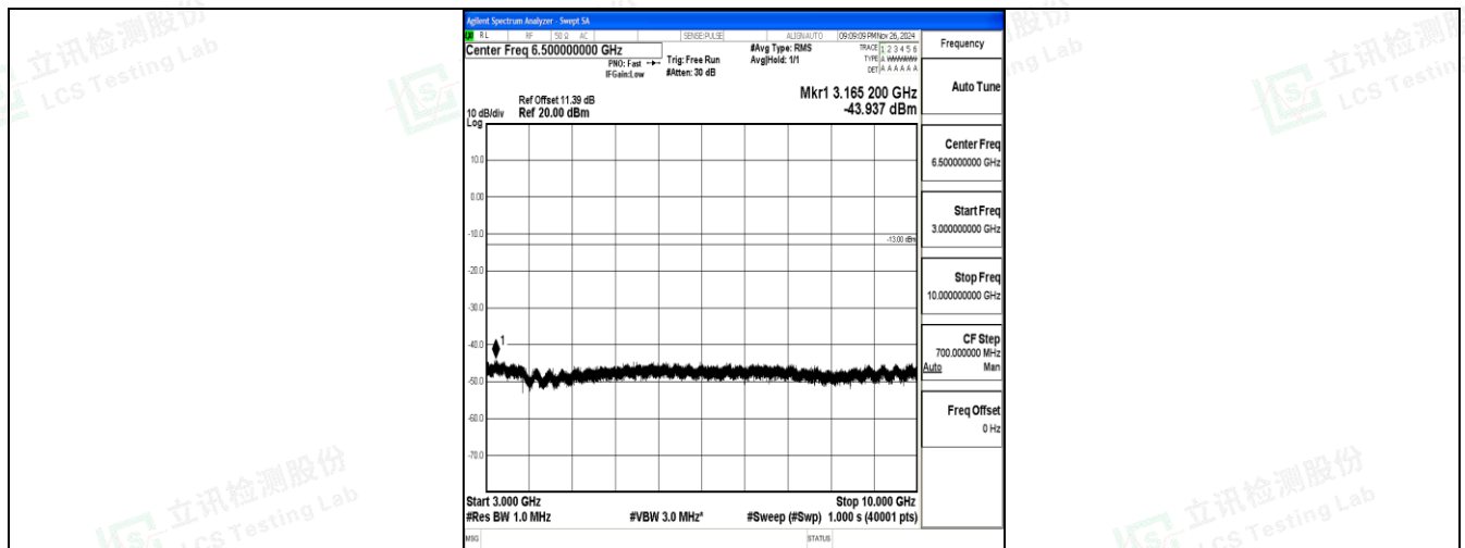
Band17_10MHz_16QAM_23790_1RB#0_3000~10000_3000~10000
