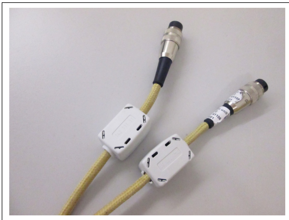
Photograph A3-12: Signal and power cable, detailed view of ferrites (Wuerth 742 711 31)
