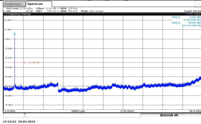
11N20SISO_Ant1_2417_1000~26500
