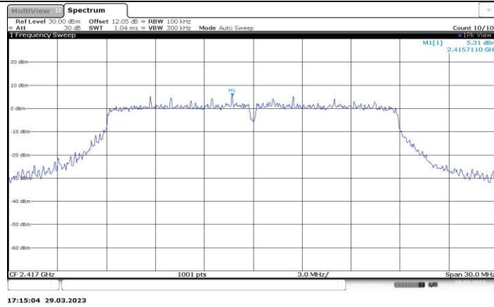
11N20SISO_Ant1_2417_0~Reference
