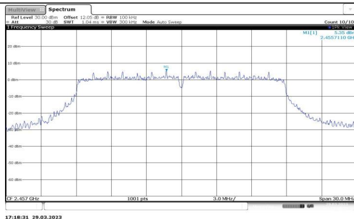
11N20SISO_Ant1_2457_0~Reference
