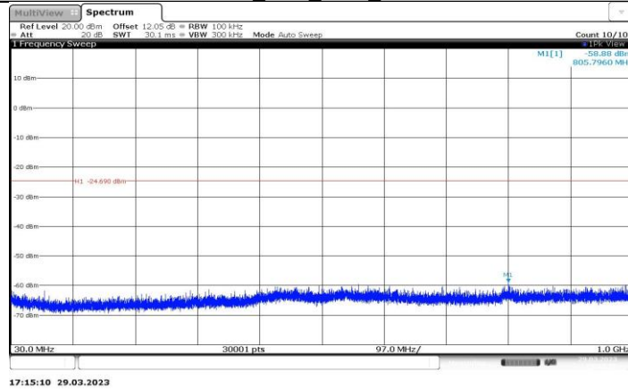
11N20SISO_Ant1_2417_30~1000
