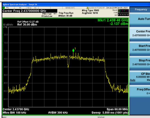
11N40SISO-Ant1-2437-30~1000--2.14
