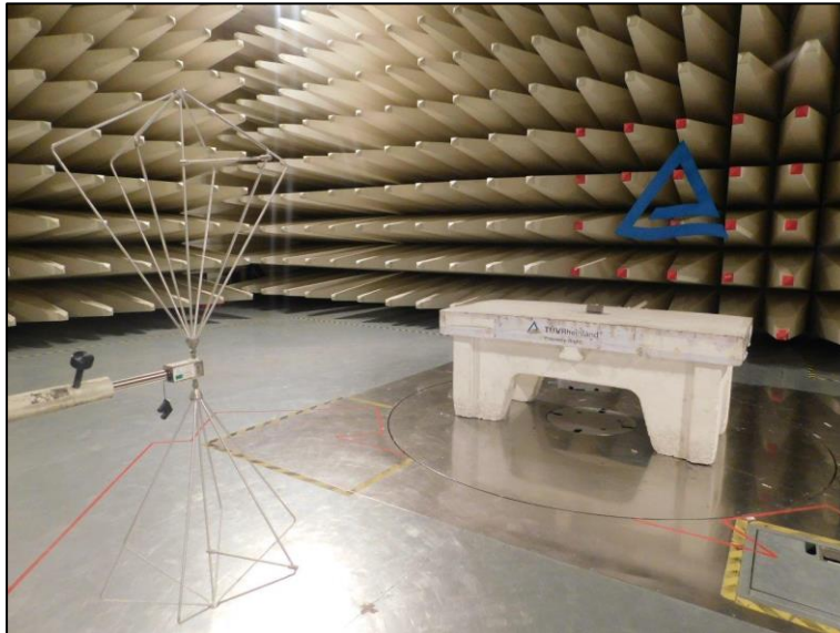
Frequency range :30MHz–200MHz Polarization : Vertical
