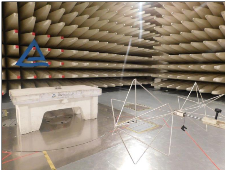
Frequency range : 30MHz–200MHz Polarization : Horizontal
