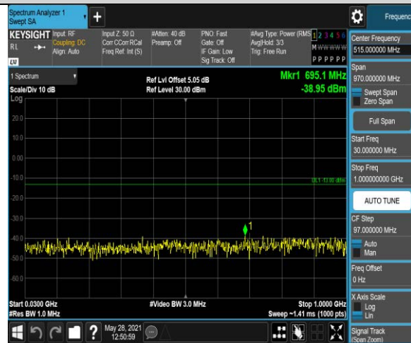
Band4-20MHz-16QAM-20050-1RB#0-Range1:30~1
