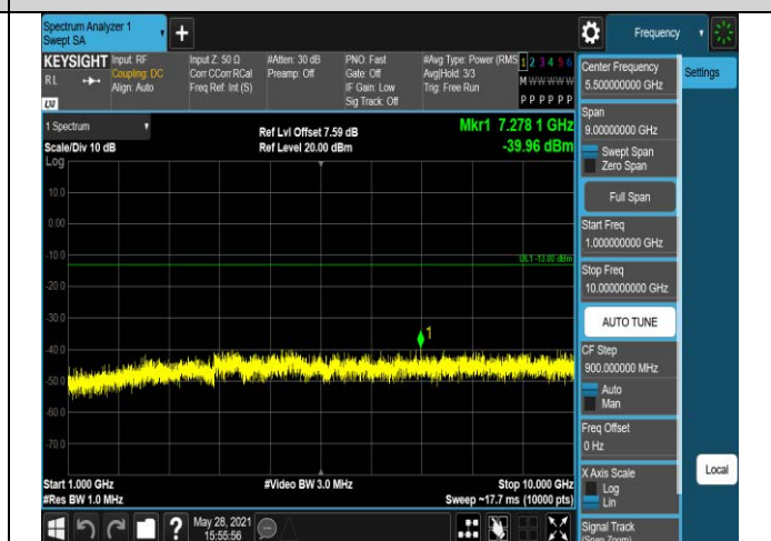
Band12-1.4MHz-QPSK-23095-1RB#0-Range2:1000~1
