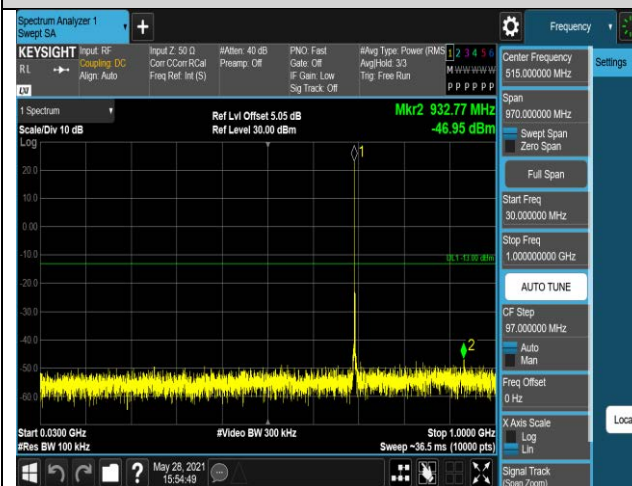
Band12-1.4MHz-QPSK-23095-1RB#0-Range1:30~1
