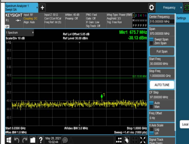
Band2-1.4MHz-16QAM-18607-1RB#0-Range1:30~1
