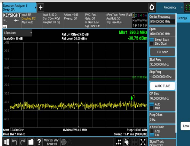
Band4-1.4MHz-16QAM-20175-1RB#0-Range1:30~1
