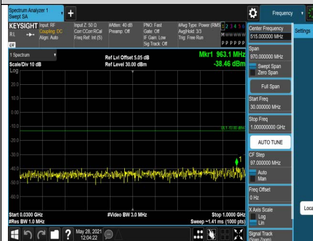
Band4-1.4MHz-QPSK-20175-1RB#0-Range1:30~10
