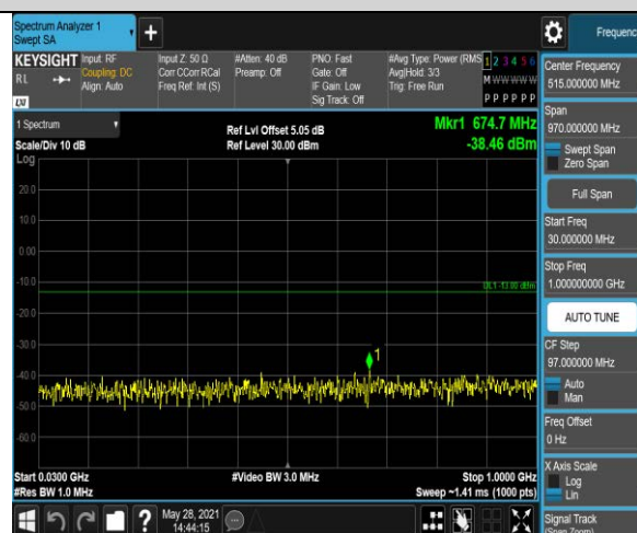
Band4-20MHz-16QAM-20175-1RB#0-Range1:30~1
