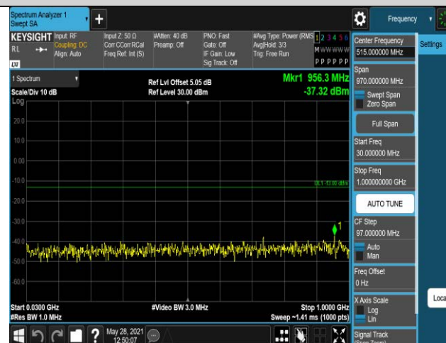
Band4-20MHz-QPSK-20175-1RB#0-Range1:30~10
