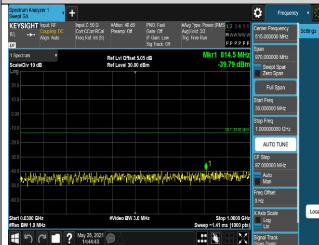
Band12-1.4MHz-QPSK-23017-1RB#0-Range1:30~1
