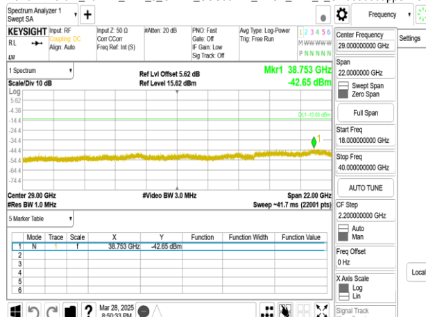
Band77-Part27_10MHz_DFT_s_OFDM_SCS30kHz_BPSK_RB1_1_CH656000upper 18G
