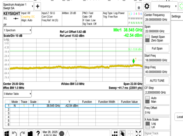
Band77-Part27_20MHz_DFT_s_OFDM_SCS30kHz_BPSK_RB1_1_CH664666upper 18G
