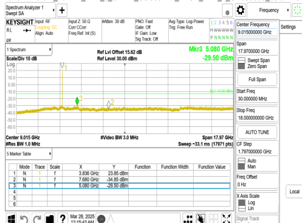
Band77-Part27_10MHz_DFT_s_OFDM_SCS30kHz_BPSK_RB1_1_CH656000_below 18G
