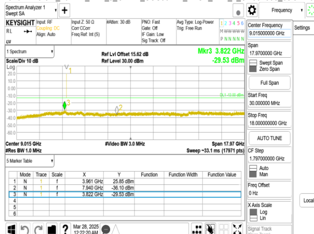
Band77-Part27_20MHz_DFT_s_OFDM_SCS30kHz_BPSK_RB1_1_CH664666upper 18G
