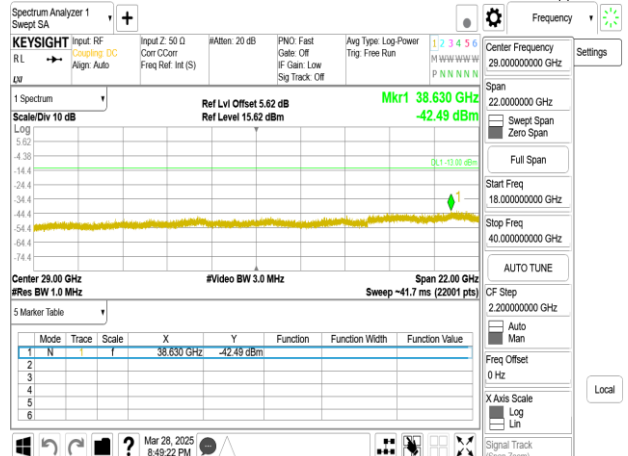
Band77-Part27_10MHz_DFT_s_OFDM_SCS30kHz_BPSK_RB1_1_CH636332upper 18G
