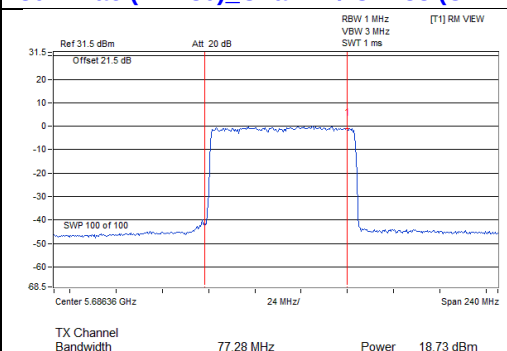
802.11ac (VHT80)_Chain 1 / CH138 (U-NII-2C Band)
