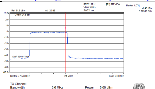
802.11ac (VHT80)_Chain 0 / CH138 (U-NII-3 Band)
