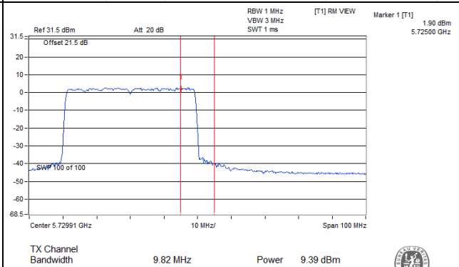
802.11ac (VHT40)_Chain 0 / CH142 (U-NII-3 Band)
