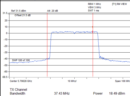
802.11ac (VHT40)_Chain 0 / CH142 (U-NII-2C Band)
