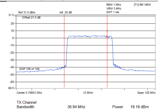
802.11ax (HE40)_Chain 1 / CH142 (U-NII-2C Band)
