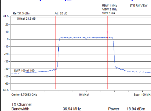
802.11ac (VHT40)_Chain 1 / CH142 (U-NII-2C Band)
