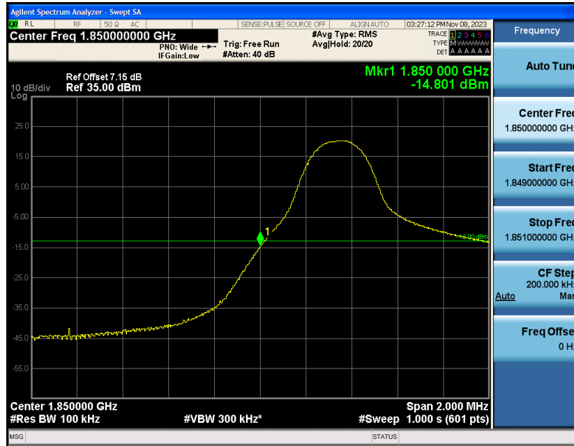
Band2-5MHz-16QAM-18625-1RB#24
