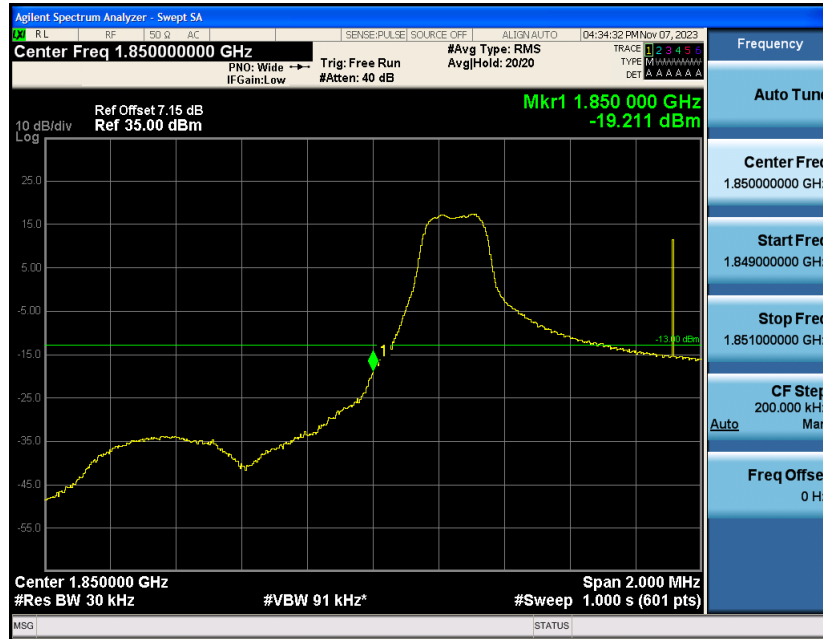
Band2-1.4MHz-16QAM-18607-1RB#5
