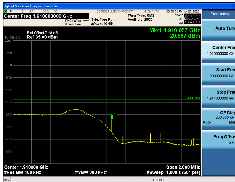
Band2-5MHz-16QAM-19175-1RB#24
