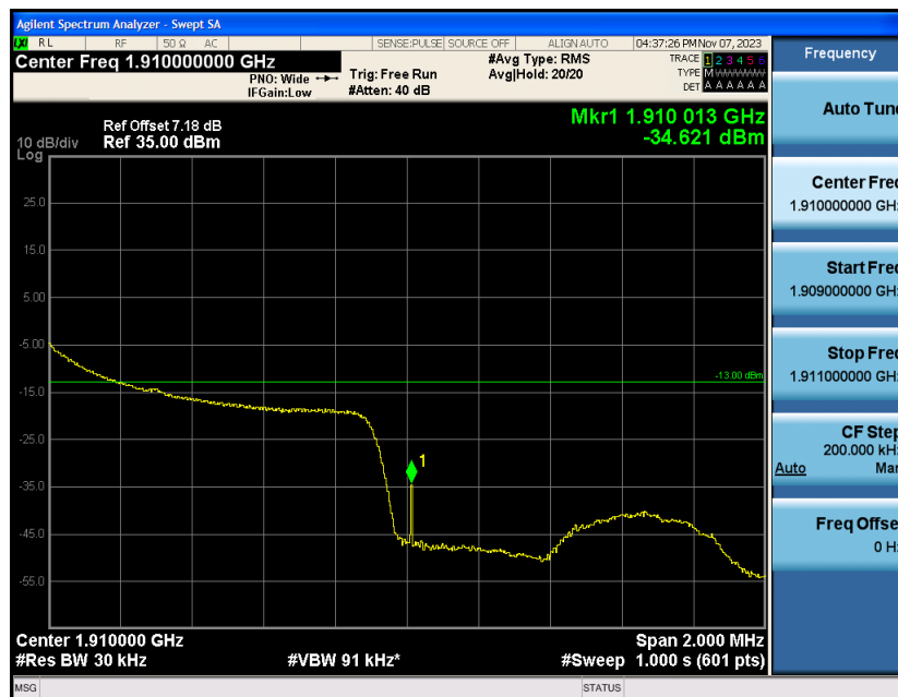
Band2-1.4MHz-16QAM-19193-1RB#5
