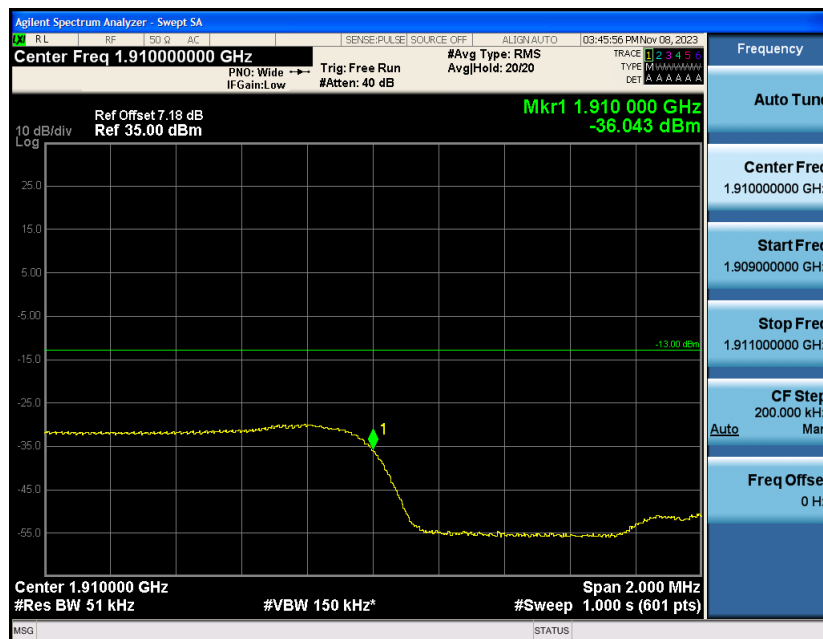
Band2-3MHz-16QAM-19185-1RB#14
