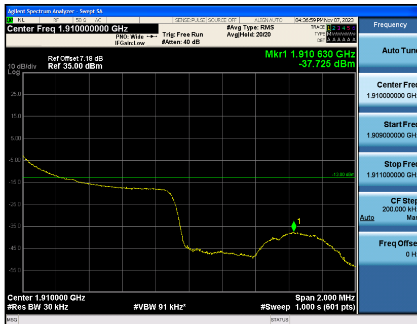
Band2-1.4MHz-QPSK-19193-1RB#5
