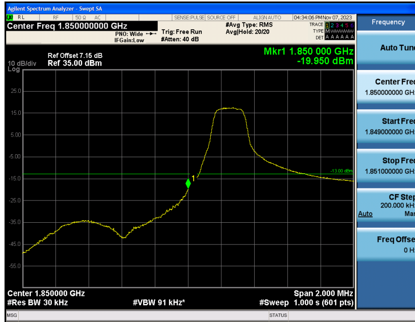
Band2-1.4MHz-QPSK-18607-1RB#5
