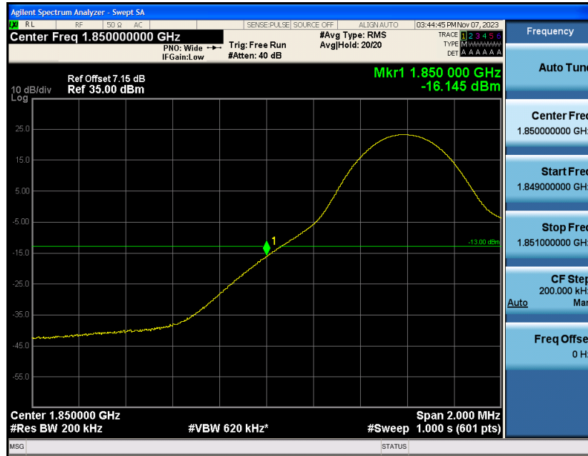
Band2-10MHz-QPSK-18650-1RB#49
