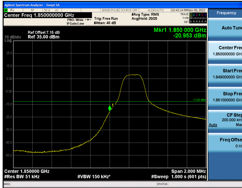
Band2-3MHz-16QAM-18615-1RB#14
