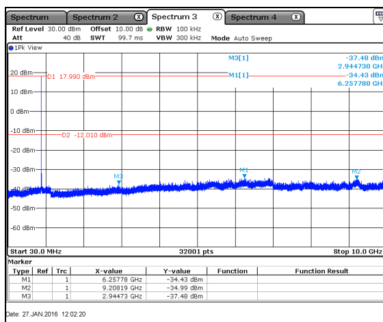
Figure 7.5.1.2-1: 30 MHz – 10 GHz – LCH – Port 0
