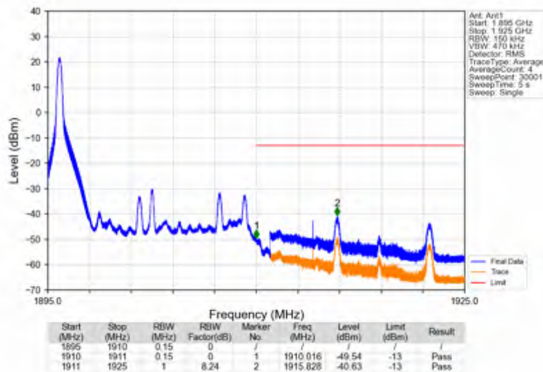
Band2_15MHz_64QAM_HCH_1902.5MHz_RB_75_0_NTNV
