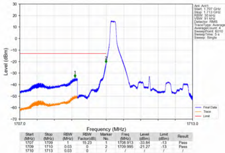
Band4_3MHz_64QAM_LCH_1711.5MHz_RB_1_0_NTNV
