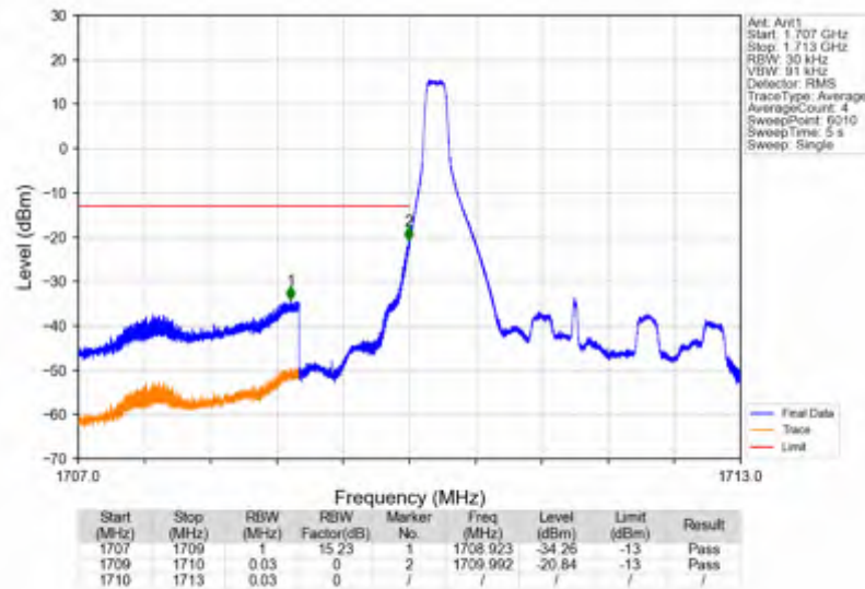
Band4_3MHz_QPSK_LCH_1711.5MHz_RB_15_0_NTNV
