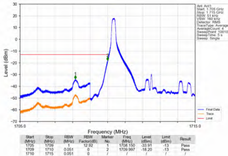
Band4_5MHz_16QAM_LCH_1712.5MHz_RB_1_0_NTNV
