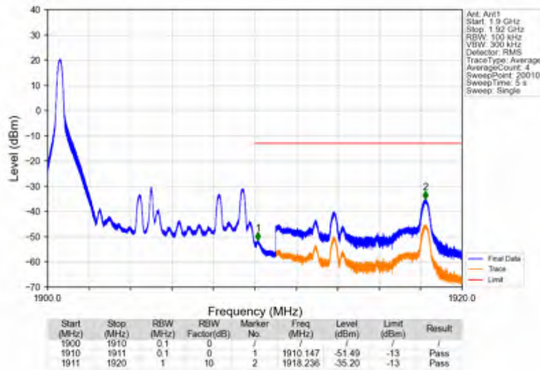
Band2_10MHz_64QAM_HCH_1905MHz_RB_50_0_NTNV
