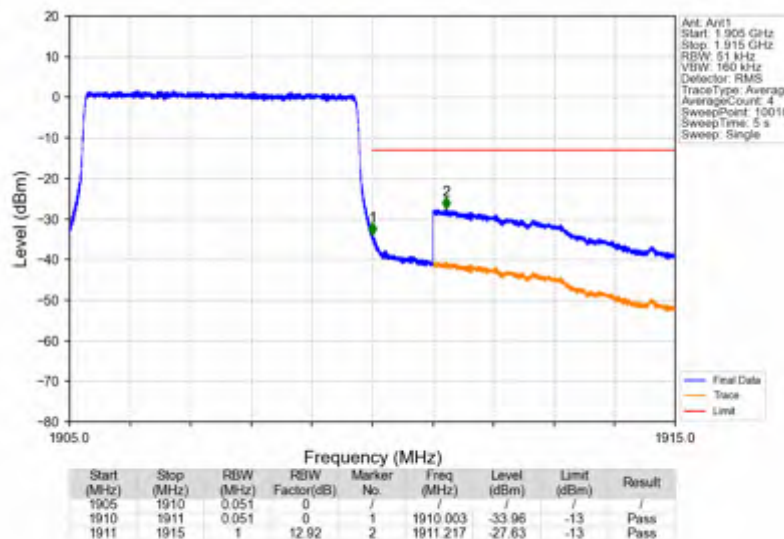
Band2_5MHz_256QAM_HCH_1907.5MHz_RB_25_0_NTNV
