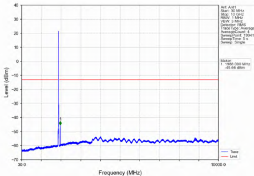
Band2_15MHz_64QAM_HCH_1902.5MHz_RB_1_0_NTNV
