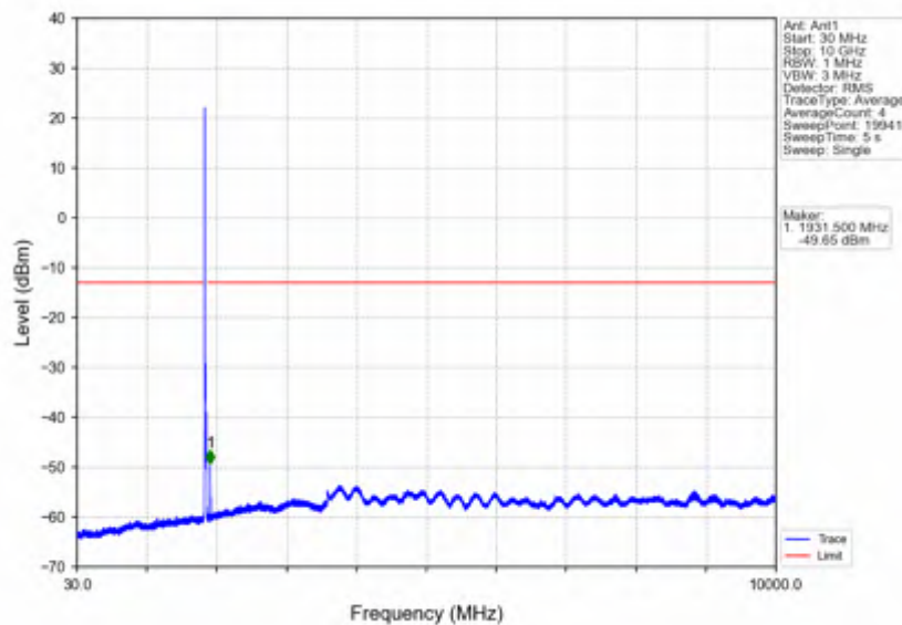
Band2_15MHz_64QAM_LCH_1857.5MHz_RB_1_0_NTNV
