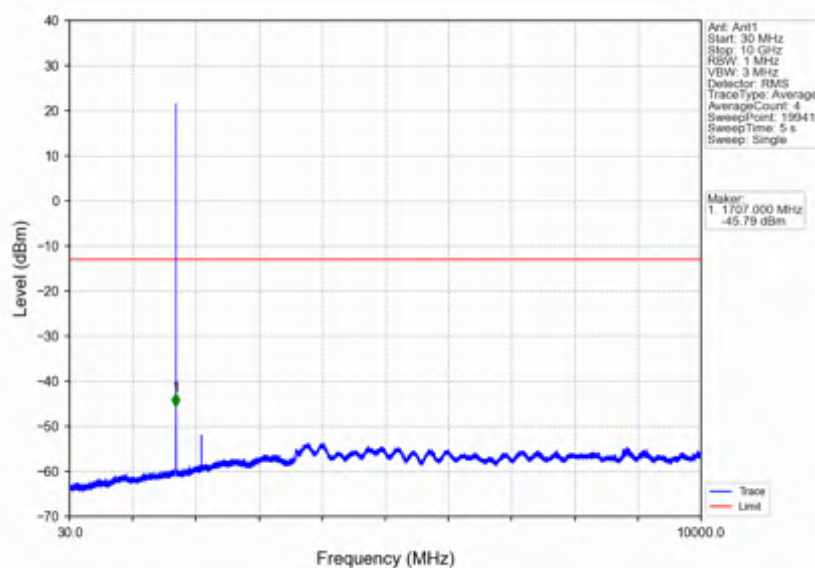
Band4_1.4MHz_QPSK_LCH_1710.7MHz_RB_1_0_NTNV
