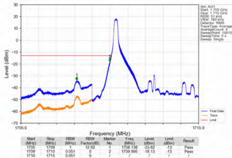
Band4_5MHz_64QAM_LCH_1712.5MHz_RB_25_0_NTNV
