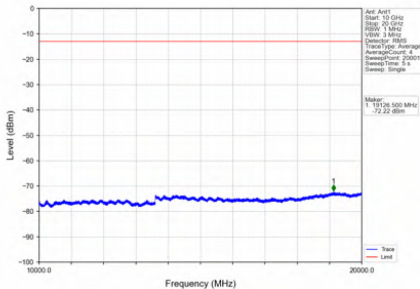
Band4_1.4MHz_16QAM_HCH_1754.3MHz_RB_1_0_NTNV
