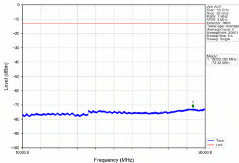
Band2_15MHz_QPSK_LCH_1857.5MHz_RB_75_0_NTNV
