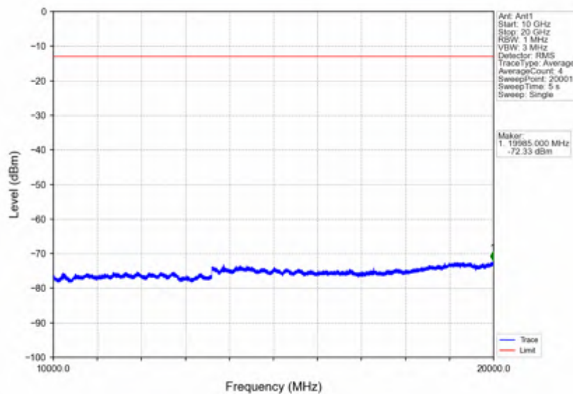
Band2_15MHz_16QAM_HCH_1902.5MHz_RB_1_0_NTNV
