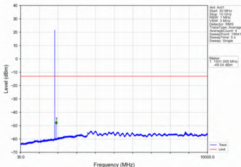
Band2_3MHz_64QAM_LCH_1851.5MHz_RB_1_0_NTNV
