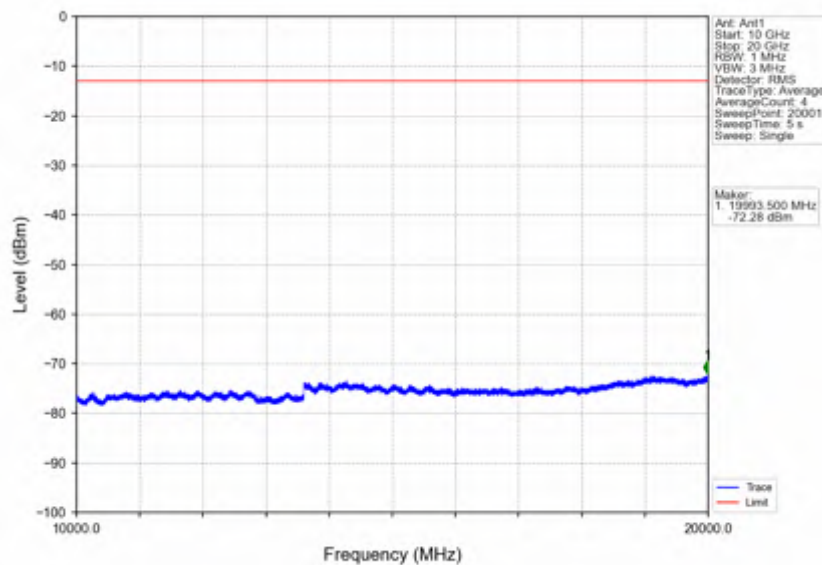
Band2_5MHz_QPSK_HCH_1907.5MHz_RB_1_0_NTNV
