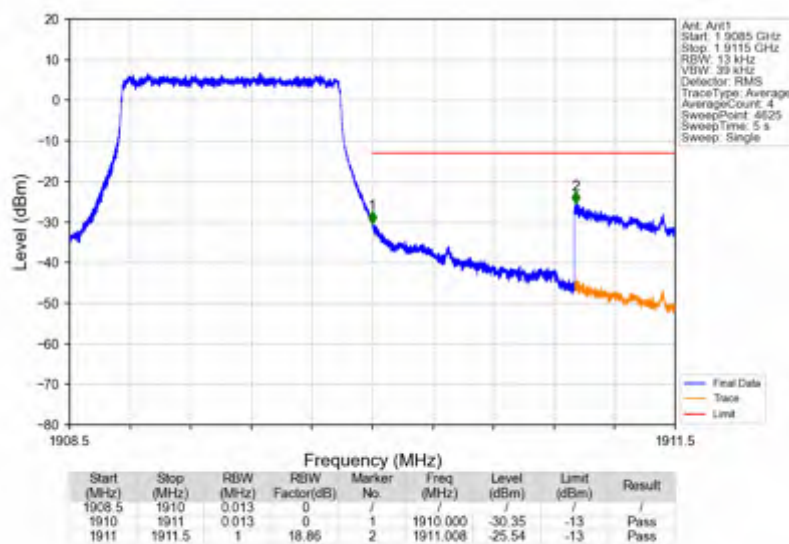
Band2_1.4MHz_QPSK_HCH_1909.3MHz_RB_6_0_NTNV
