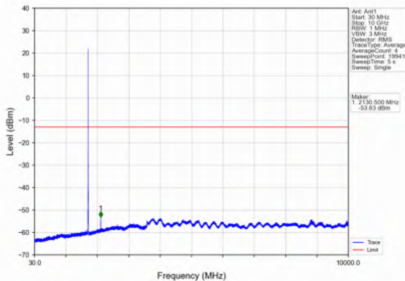
Band4 5MHz 64QAM MCH 1732.5MHz RB 1 0 NTNV
