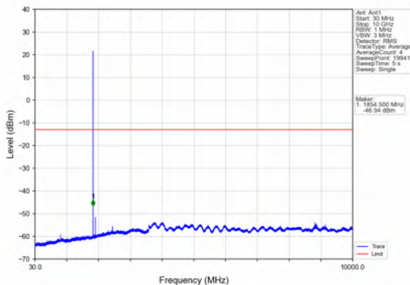
Band2_1.4MHz_QPSK_LCH_1850.7MHz_RB_1_0_NTNV
