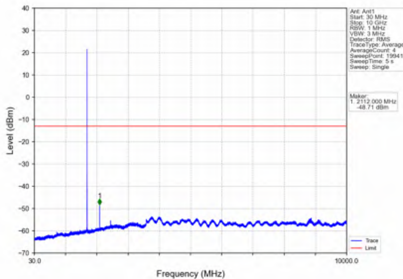
Band4_3MHz_64QAM_LCH_1711.5MHz_RB_1_0_NTNV
