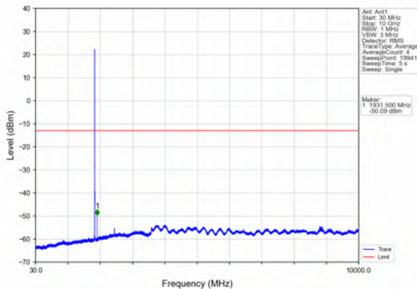
Band2_5MHz_16QAM_LCH_1852.5MHz_RB_1_0_NTNV
