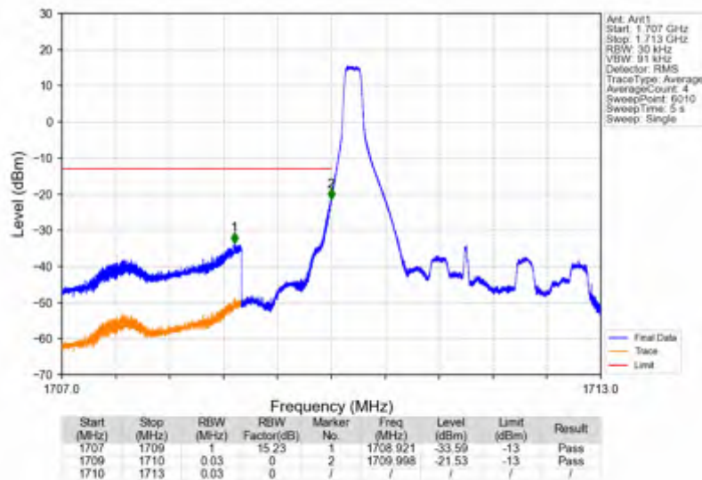
Band4_3MHz_QPSK_LCH_1711.5MHz_RB_1_0_NTNV
