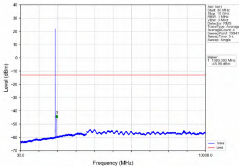
Band2_5MHz_16QAM_HCH_1907.5MHz_RB_1_0_NTNV
