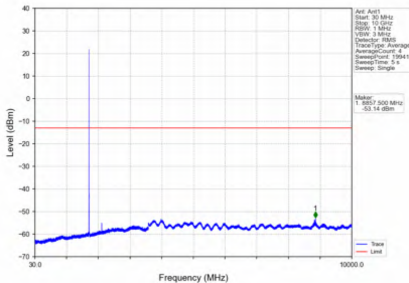
Band4_3MHz_QPSK_MCH_1732.5MHz_RB_1_0_NTNV
