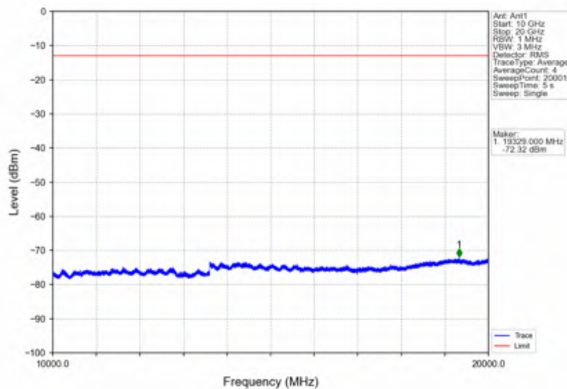
Band4_5MHz_256QAM_MCH_1732.5MHz_RB_1_0_NTNV
