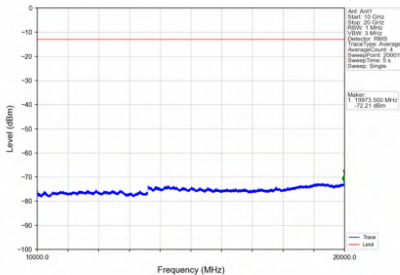
Band2_1.4MHz_256QAM_MCH_1880MHz_RB_1_0_NTNV
