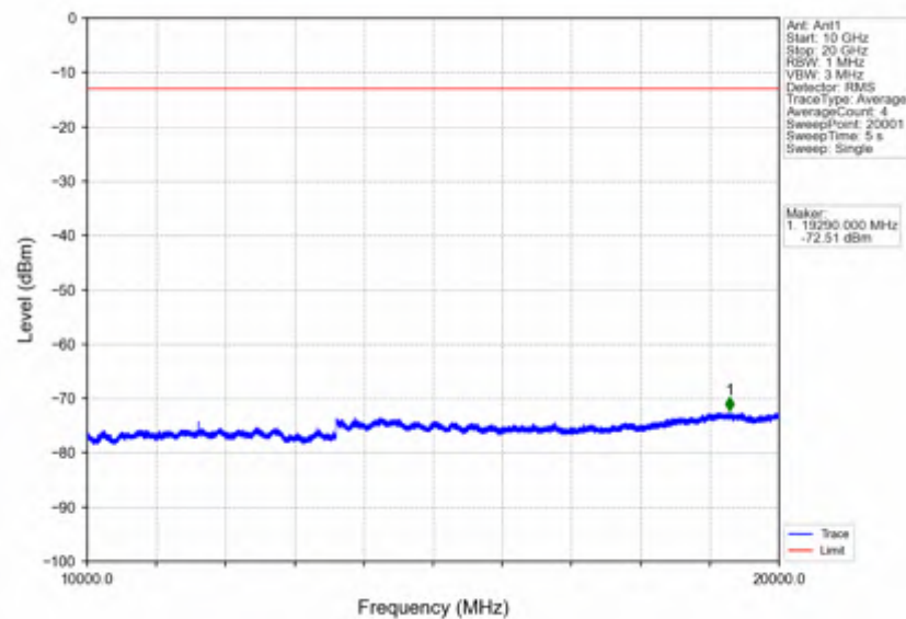
Band2_3MHz_QPSK_LCH_1851.5MHz_RB_15_0_NTNV
