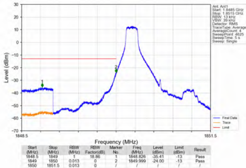
Band2_1.4MHz_64QAM_LCH_1850.7MHz_RB_1_0_NTNV
