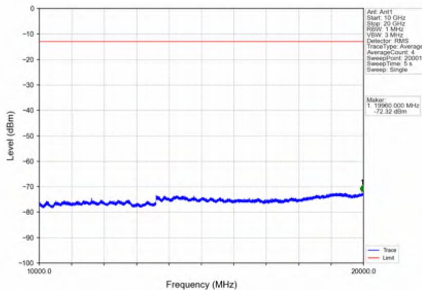
Band4_1.4MHz_QPSK_MCH_1732.5MHz_RB_1_0_NTNV
