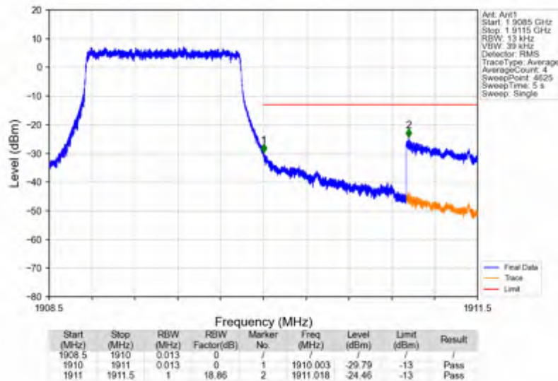
Band2_1.4MHz_64QAM_HCH_1909.3MHz_RB_1_5_NTNV
