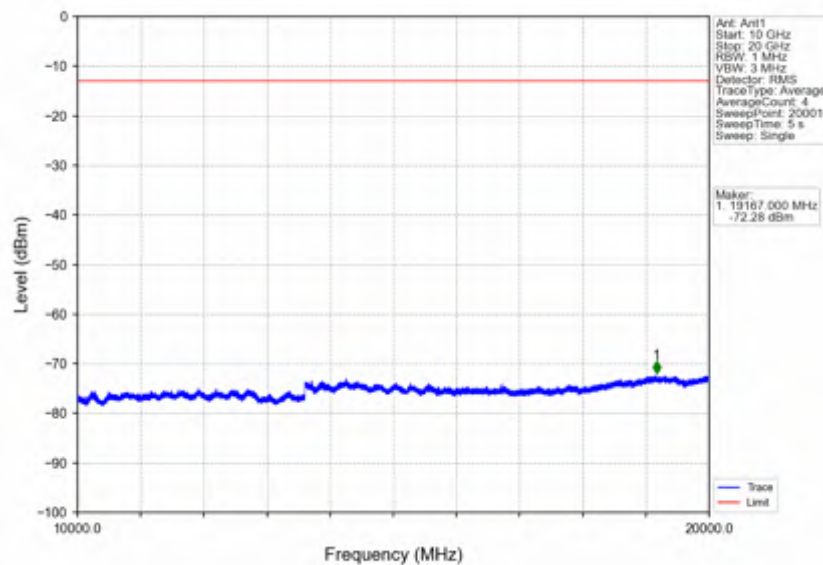
Band4_3MHz_256QAM_HCH_1753.5MHz_RB_1_0_NTNV
