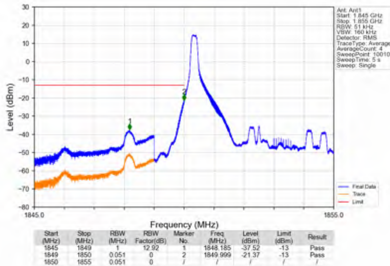
Band2 5MHz 256QAM LCH 1852.5MHz RB 1 0 NTN
