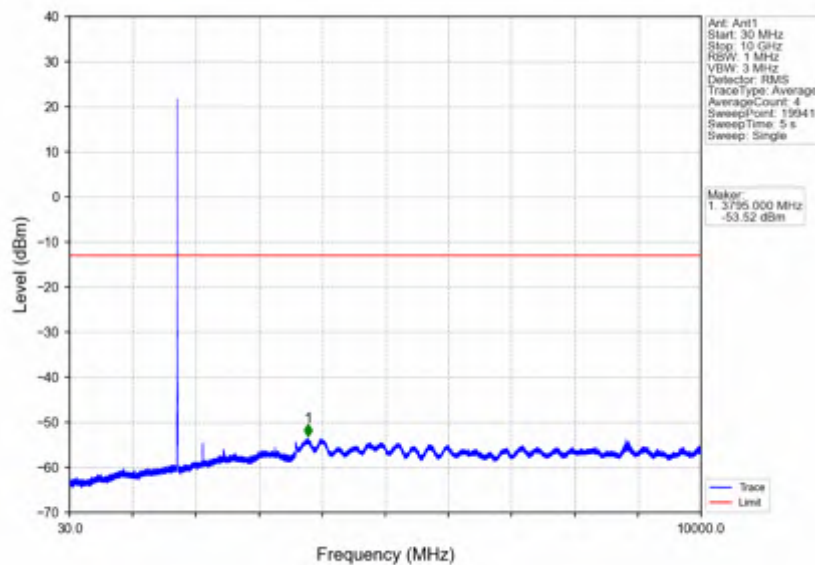
Band4_5MHz_QPSK_MCH_1732.5MHz_RB_1_0_NTNV
