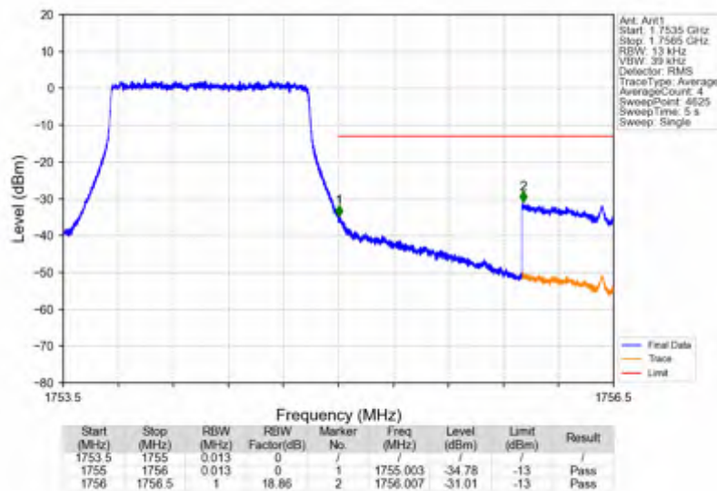
Band4 1.4MHz 256QAM HCH 1754.3MHz RB 6 0 NTNV
