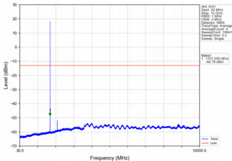
Band4 1.4MHz 256QAM LCH 1710.7MHz RB 1 0 NTN
