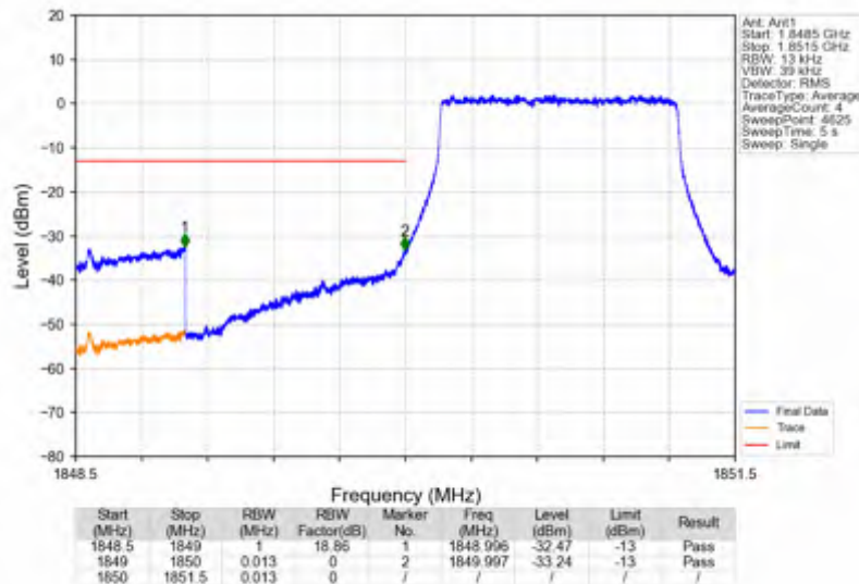
Band2_1.4MHz_256QAM_LCH_1850.7MHz_RB_6_0_NTNV
