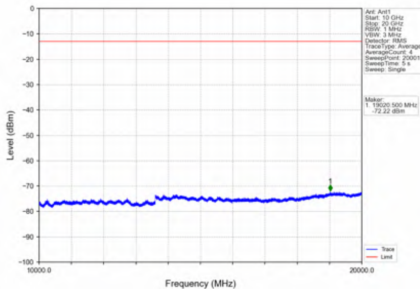
Band4_1.4MHz_16QAM_MCH_1732.5MHz_RB_1_0_NTNV
