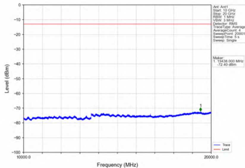
Band4_3MHz_QPSK_LCH_1711.5MHz_RB_15_0_NTNV
