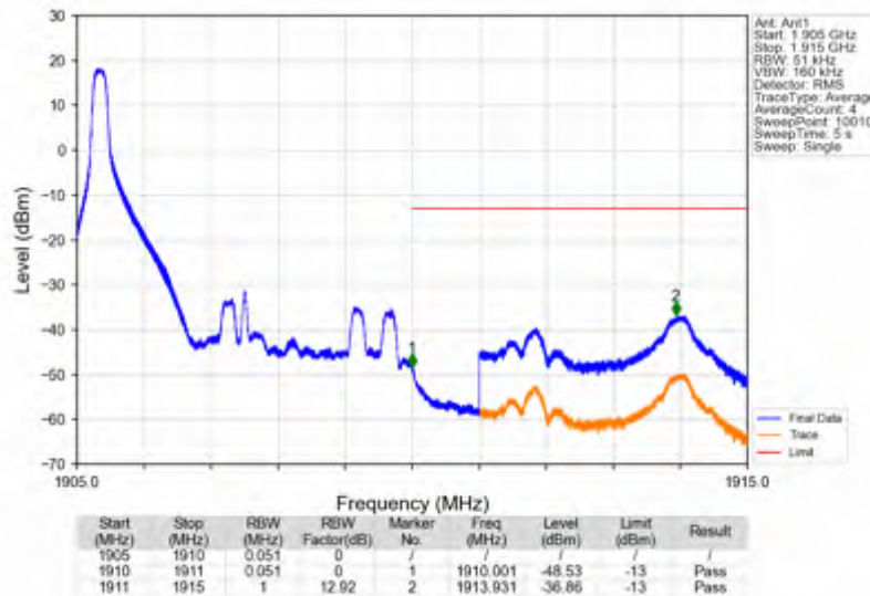
Band2_5MHz_64QAM_HCH_1907.5MHz_RB_1_24_NTNV
