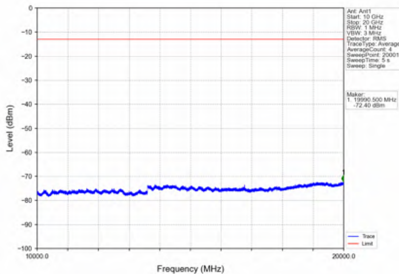
Band4_5MHz_64QAM_HCH_1752.5MHz_RB_1_0_NTNV
