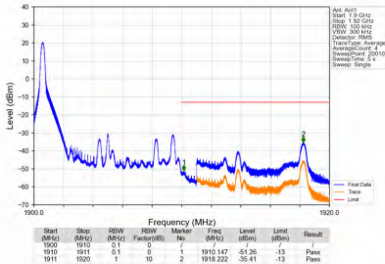
Band2_10MHz_64QAM_HCH_1905MHz_RB_1_49_NTNV
