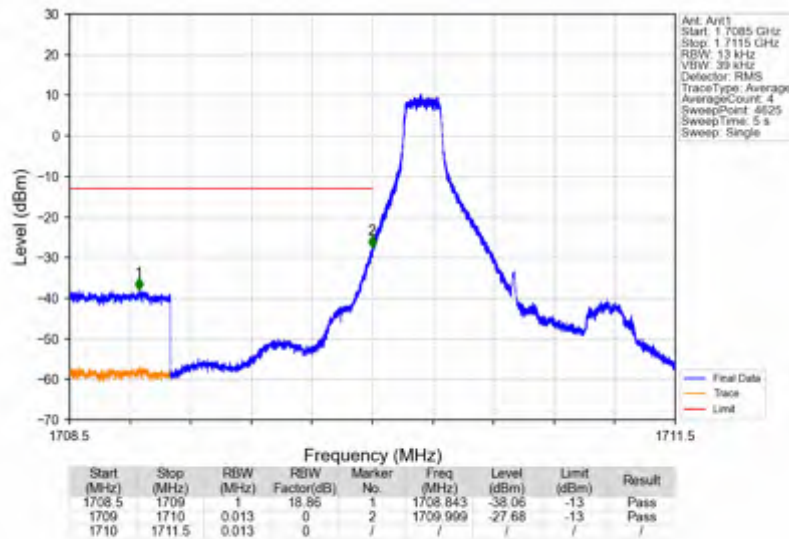
Band4 1.4MHz 256QAM LCH 1710.7MHz RB 1 0 NTN
