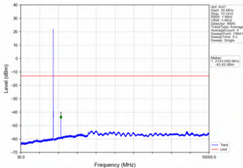
Band4_5MHz_16QAM_HCH_1752.5MHz_RB_1_0_NTNV
