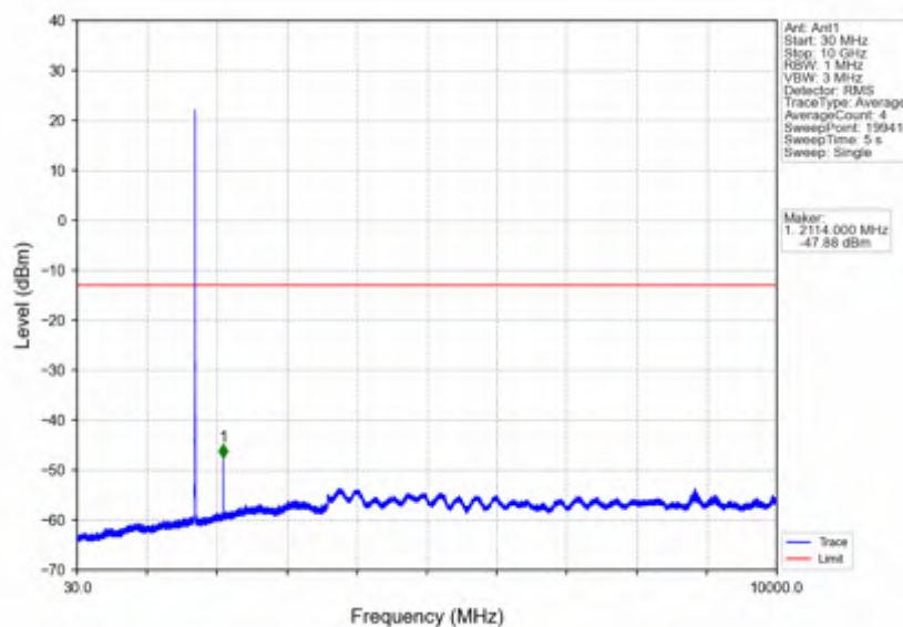
Band4_5MHz_QPSK_LCH_1712.5MHz_RB_1_0_NTNV
