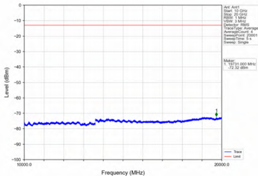
Band4_3MHz_256QAM_LCH_1711.5MHz_RB_15_0_NTNV
