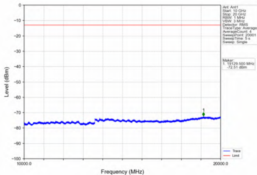
Band2_5MHz_64QAM_LCH_1852.5MHz_RB_25_0_NTNV
