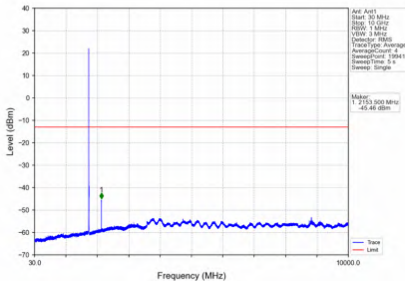
Band4_5MHz_64QAM_HCH_1752.5MHz_RB_1_0_NTNV
