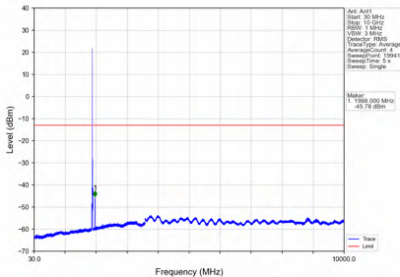
Band2_10MHz_64QAM_HCH_1905MHz_RB_1_0_NTNV
