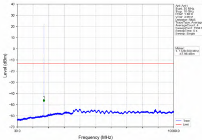
Band4_1.4MHz_QPSK_MCH_1732.5MHz_RB_1_0_NTNV
