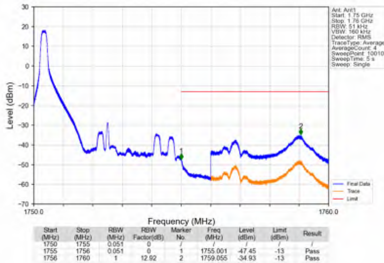
Band4_5MHz_16QAM_HCH_1752.5MHz_RB_1_24_NTNV
