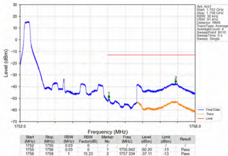
Band4_3MHz_64QAM_HCH_1753.5MHz_RB_15_0_NTNV
