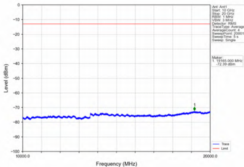
Band2_1.4MHz_16QAM_MCH_1880MHz_RB_1_0_NTNV
