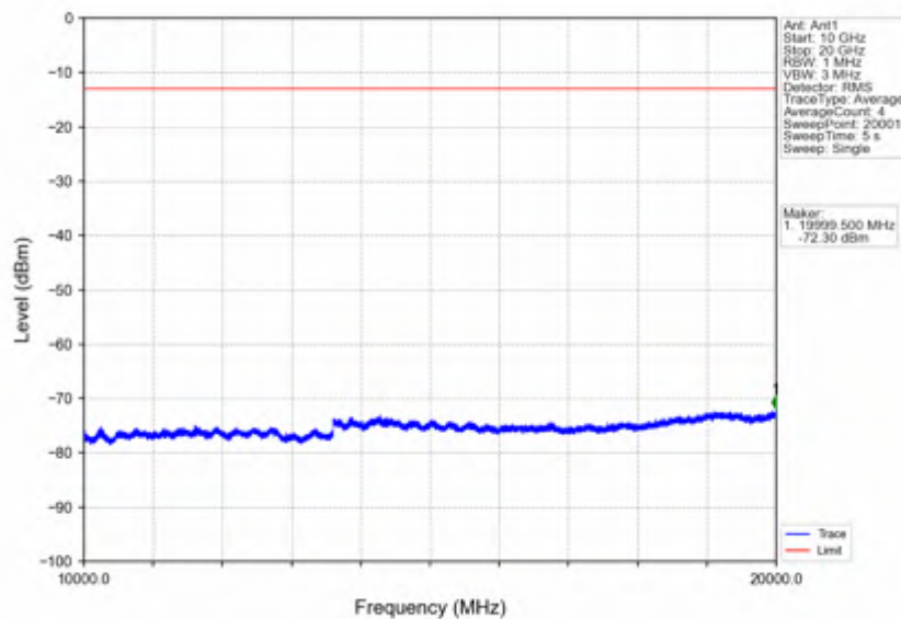
Band4_3MHz_64QAM_MCH_1732.5MHz_RB_1_0_NTNV
