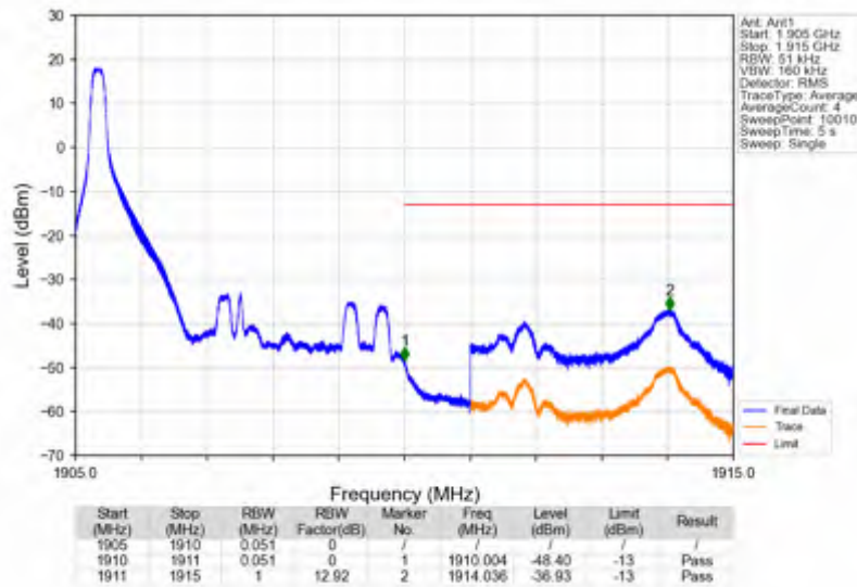
Band2_5MHz_16QAM_HCH_1907.5MHz_RB_1_24_NTNV
