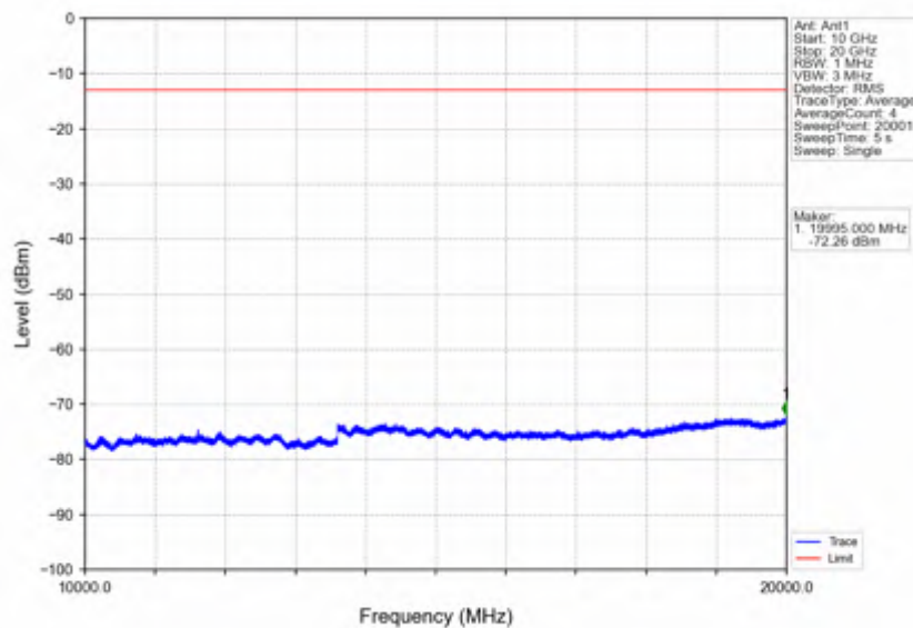
Band2_15MHz_16QAM_MCH_1880MHz_RB_1_0_NTNV
