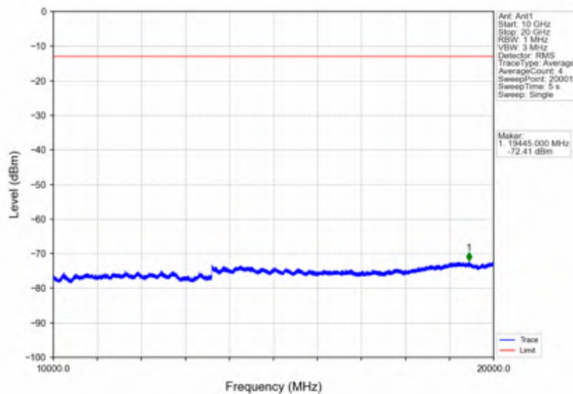
Band4_1.4MHz_QPSK_HCH_1754.3MHz_RB_1_0_NTNV
