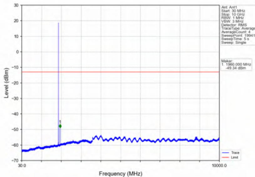
Band2_1.4MHz_256QAM_MCH_1880MHz_RB_1_0_NTNV
