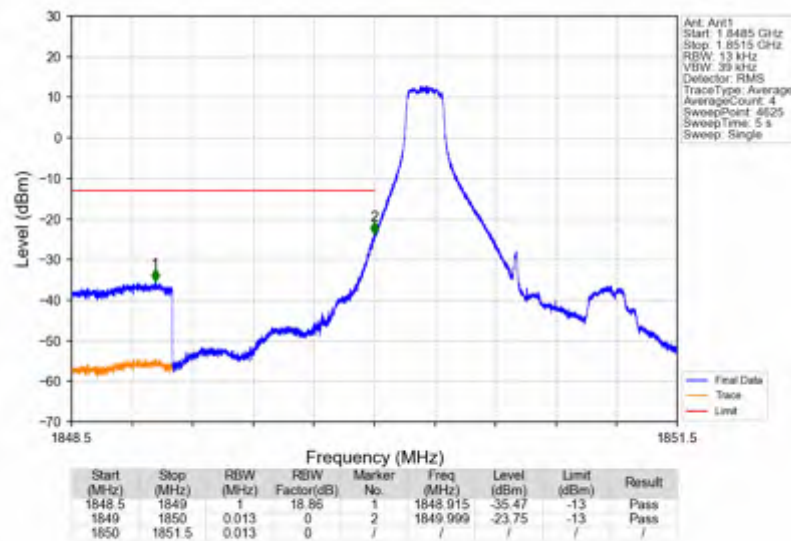
Band2_1.4MHz_QPSK_LCH_1850.7MHz_RB_6_0_NTV
