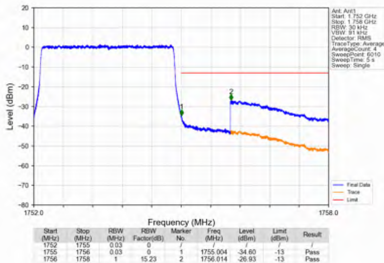
Band4_3MHz_256QAM_HCH_1753.5MHz_RB_15_0_NTNV
