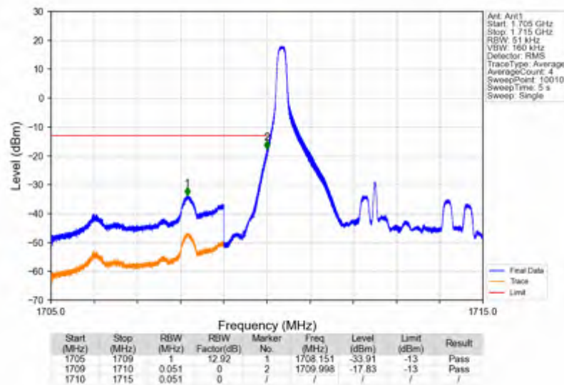
Band4_5MHz_QPSK_LCH_1712.5MHz_RB_25_0_NTNV
