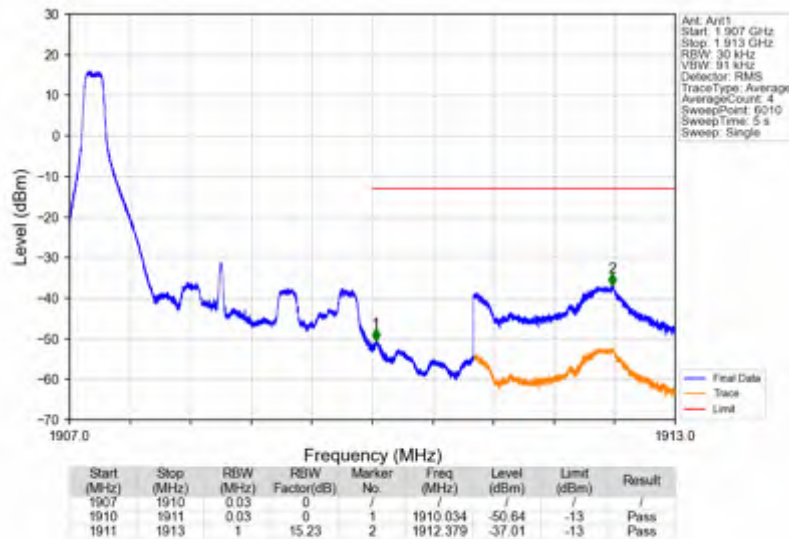
Band2_3MHz_64QAM_HCH_1908.5MHz_RB_1_14_NTNV
