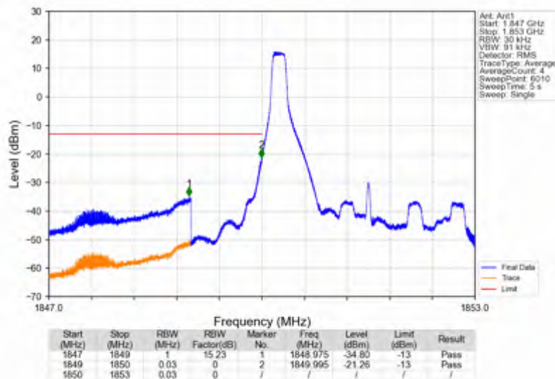
Band2_3MHz_64QAM_LCH_1851.5MHz_RB_15_0_NTNV
