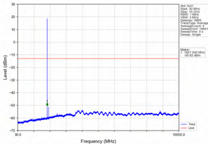
Band2_1.4MHz_256QAM_LCH_1850.7MHz_RB_1_0_NTNV
