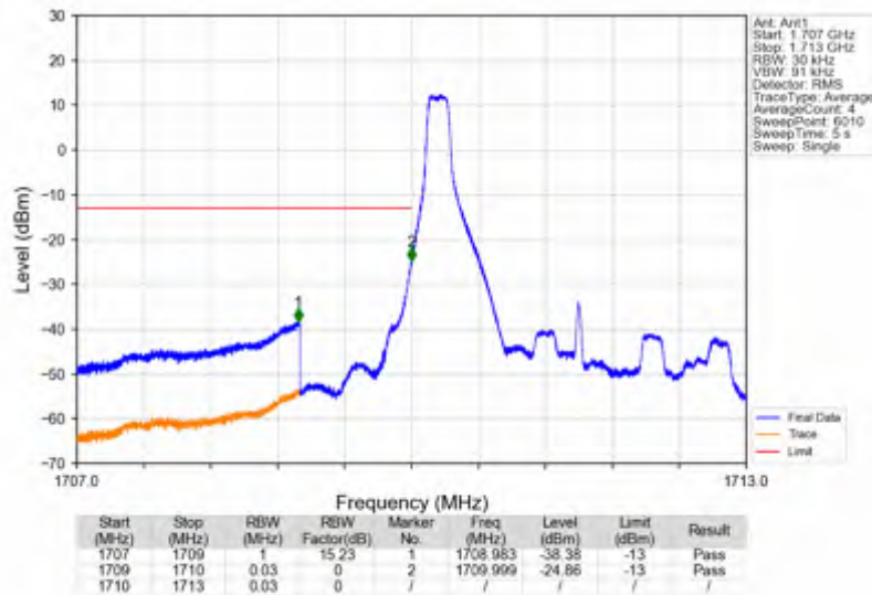
Band4_3MHz_256QAM_LCH_1711.5MHz_RB_1_0_NTNV
