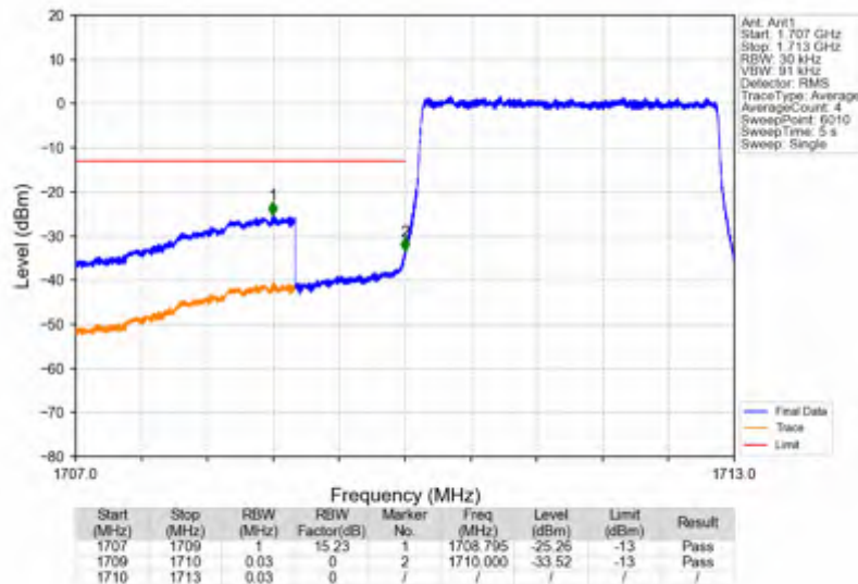
Band4_3MHz_256QAM_LCH_1711.5MHz_RB_15_0_NTNV
