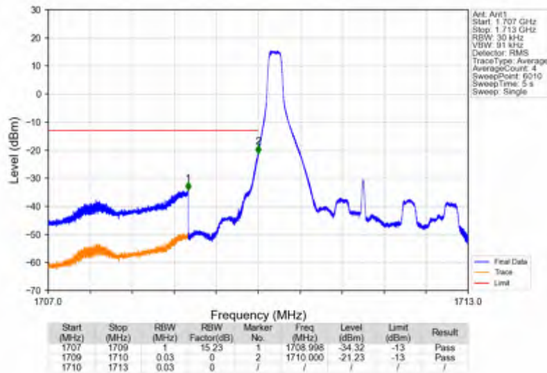
Band4_3MHz_64QAM_LCH_1711.5MHz_RB_15_0_NTNV
