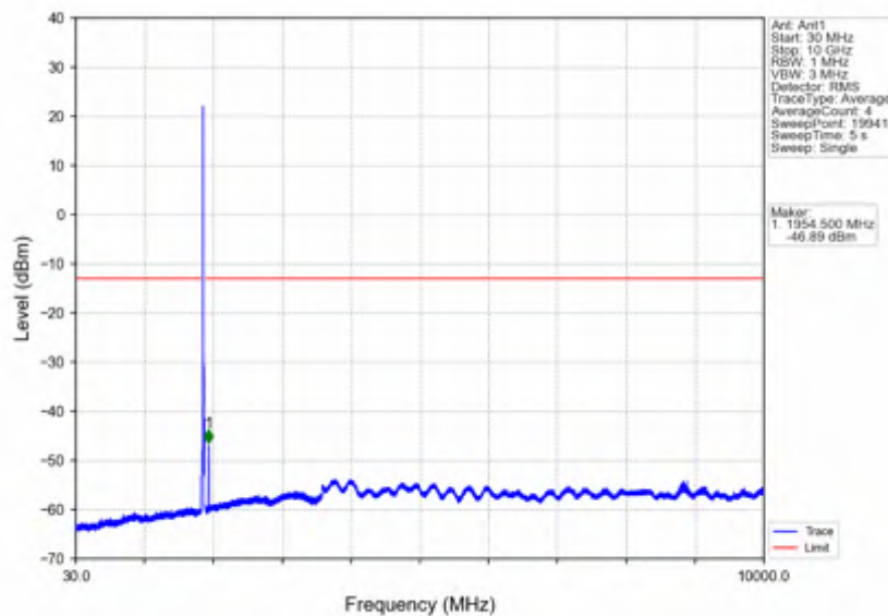
Band2_15MHz_16QAM_MCH_1880MHz_RB_1_0_NTNV
