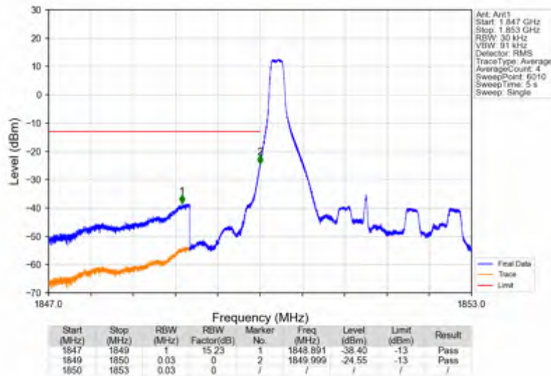
Band2_3MHz_256QAM_LCH_1851.5MHz_RB_1_0_NTNV
