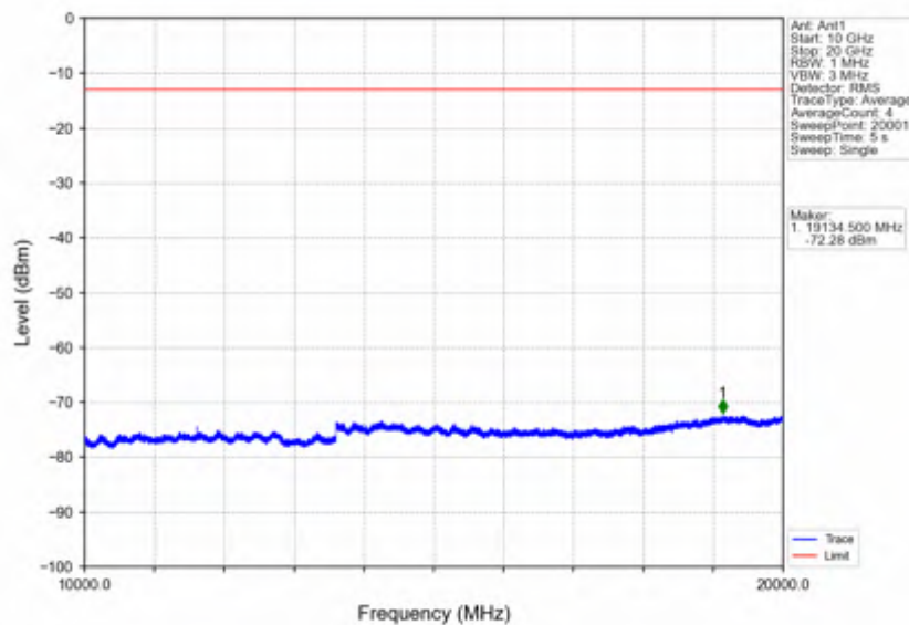
Band4_1.4MHz_256QAM_MCH_1732.5MHz_RB_1_0_NTNV
