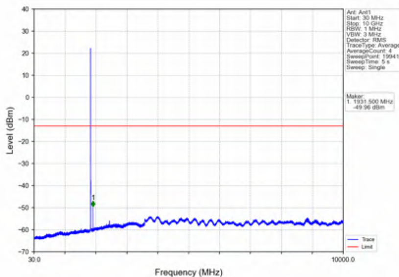
Band2_5MHz_QPSK_LCH_1852.5MHz_RB_1_0_NTNV
