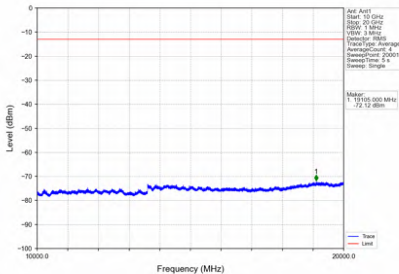
Band4_5MHz_QPSK_MCH_1732.5MHz_RB_1_0_NTNV
