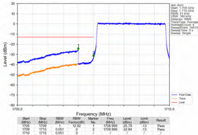
Band4_5MHz_256QAM_LCH_1712.5MHz_RB_25_0_NTNV
