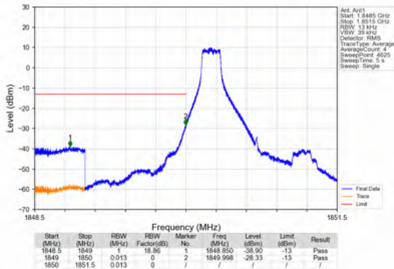
Band2_1.4MHz_256QAM_LCH_1850.7MHz_RB_1_0_NTNV
