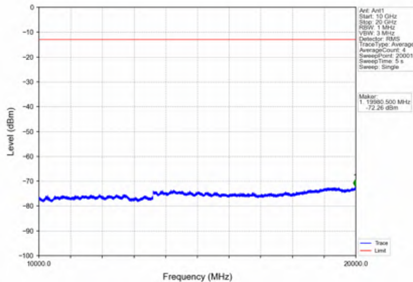
Band2_1.4MHz_16QAM_LCH_1850.7MHz_RB_6_0_NTNV
