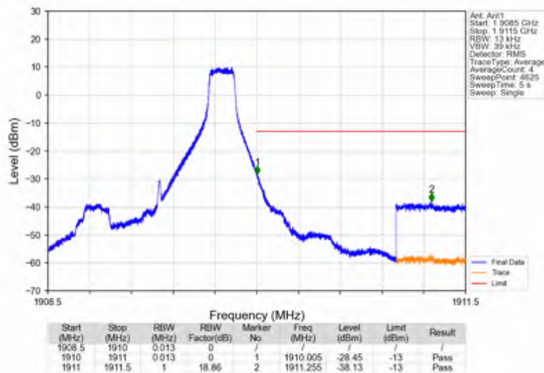
Band2_1.4MHz_256QAM_HCH_1909.3MHz_RB_6_0_NTNV
