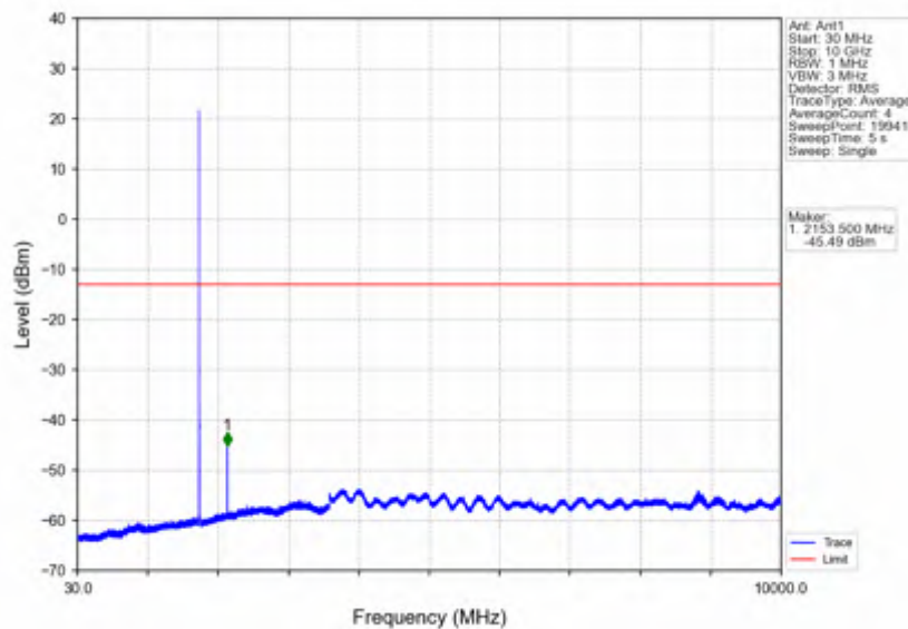
Band4 3MHz 16QAM HCH 1753.5MHz RB 1 0 NTNV
