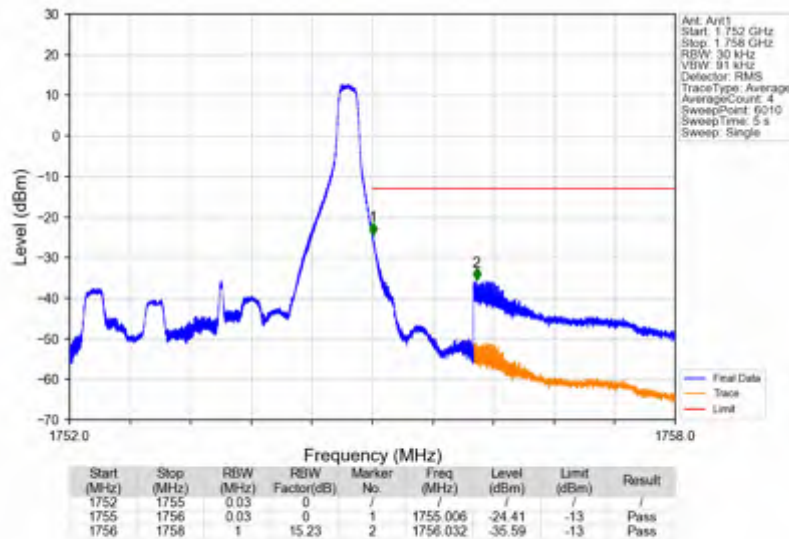
Band4_3MHz_256QAM_HCH_1753.5MHz_RB_1_14_NTNV
