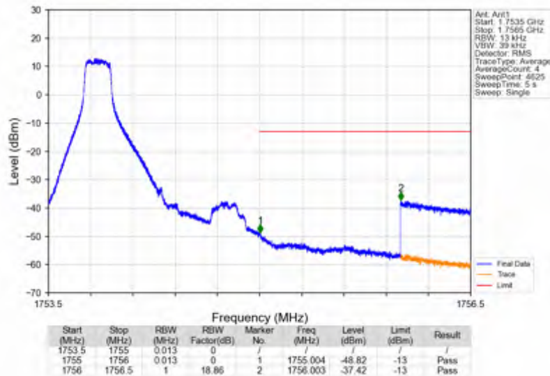
Band4_1.4MHz_16QAM_HCH_1754.3MHz_RB_1_5_NTNV
