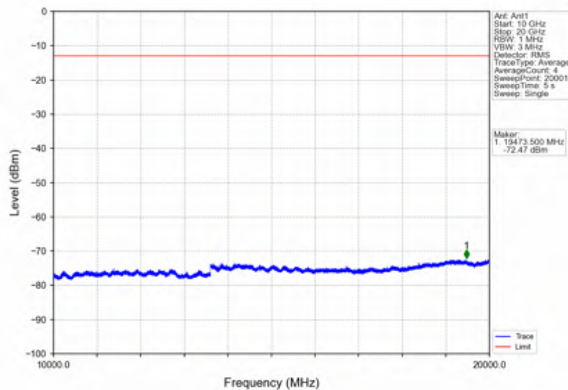
Band2_1.4MHz_256QAM_LCH_1850.7MHz_RB_6_0_NTNV
