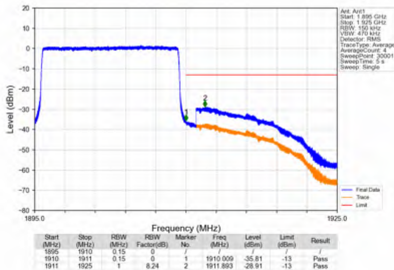
Band2_15MHz_256QAM_HCH_1902.5MHz_RB_75_0_NTNV
