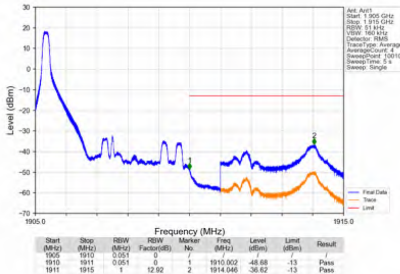
Band2_5MHz_64QAM_HCH_1907.5MHz_RB_25_0_NTNV
