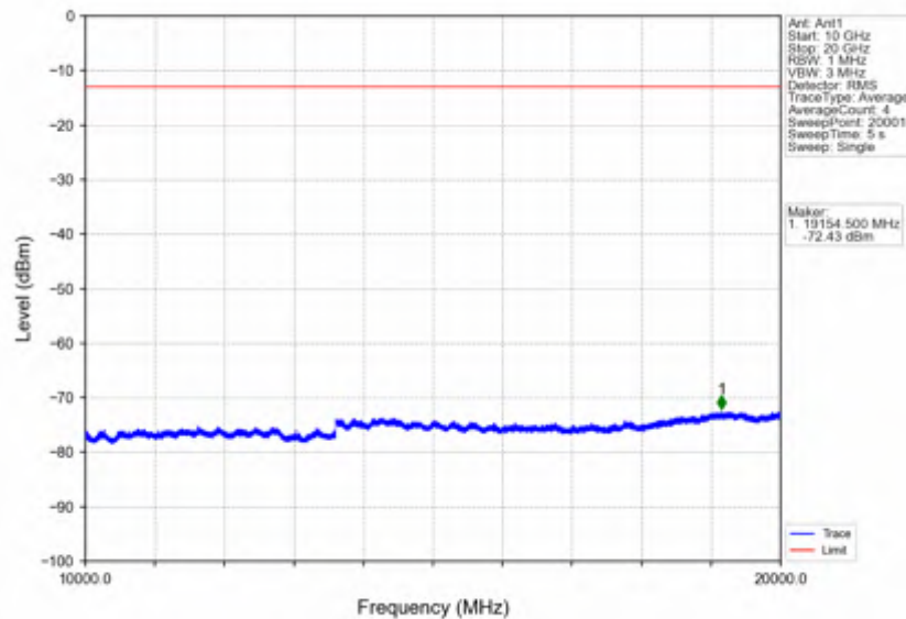
Band2_3MHz_256QAM_LCH_1851.5MHz_RB_15_0_NTNV
