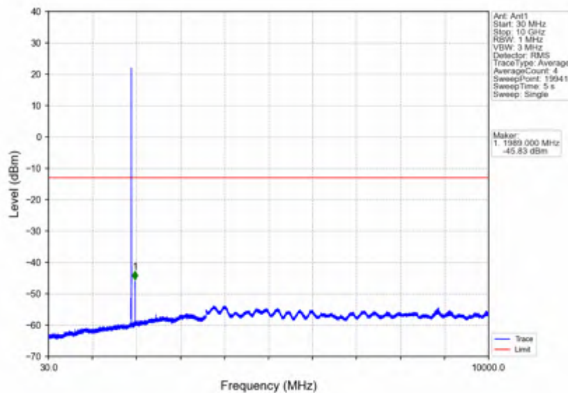
Band2_5MHz_64QAM_HCH_1907.5MHz_RB_1_0_NTNV
