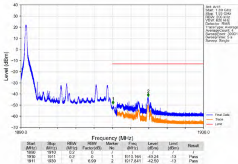
Band2_20MHz_64QAM_HCH_1900MHz_RB_100_0_NTNV
