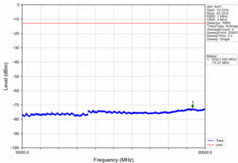
Band4_1.4MHz_64QAM_HCH_1754.3MHz_RB_1_0_NTNV
