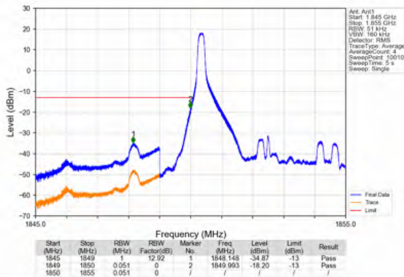
Band2_5MHz_64QAM_LCH_1852.5MHz_RB_25_0_NTNV
