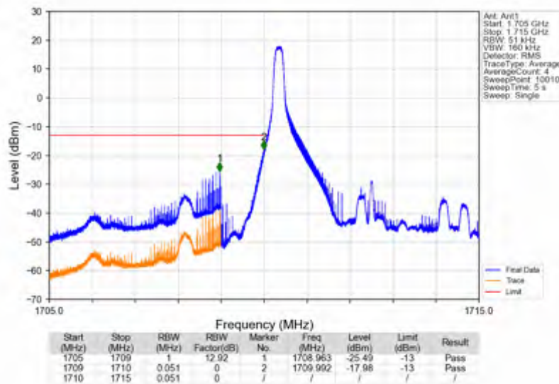
Band4_5MHz_16QAM_LCH_1712.5MHz_RB_25_0_NTNV
