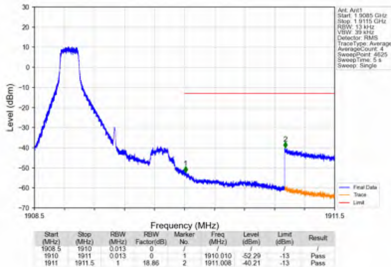
Band2_1.4MHz_256QAM_HCH_1909.3MHz_RB_1_5_NTNV
