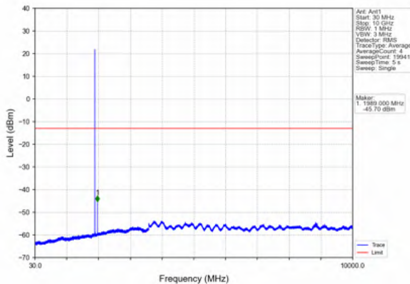
Band2_3MHz_64QAM_HCH_1908.5MHz_RB_1_0_NTNV
