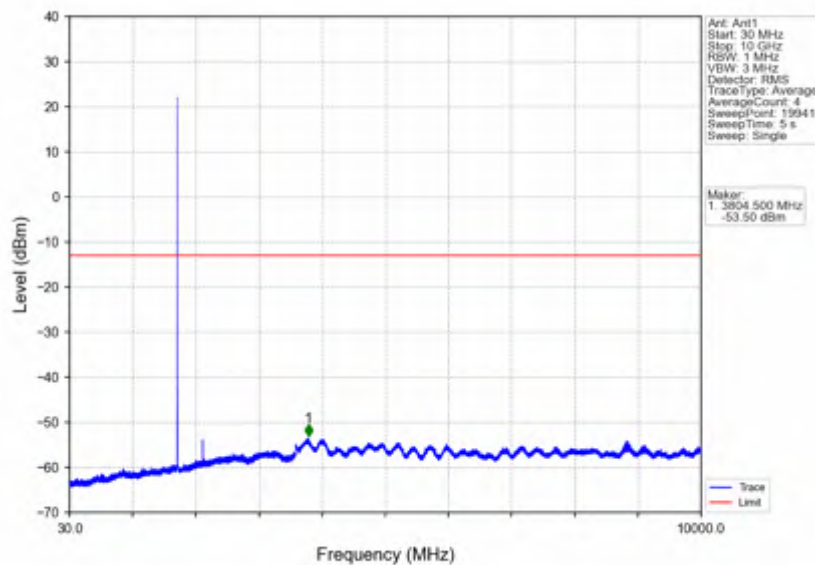
Band4_3MHz_16QAM_MCH_1732.5MHz_RB_1_0_NTNV
