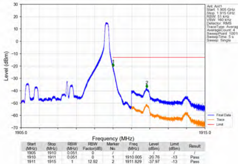
Band2_5MHz_256QAM_HCH_1907.5MHz_RB_1_24_NTNV
