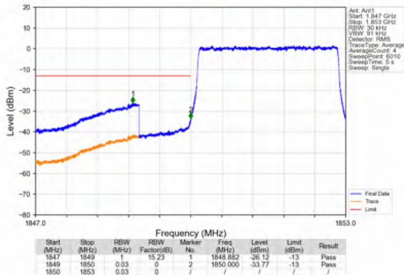
Band2_3MHz_256QAM_LCH_1851.5MHz_RB_15_0_NTNV
