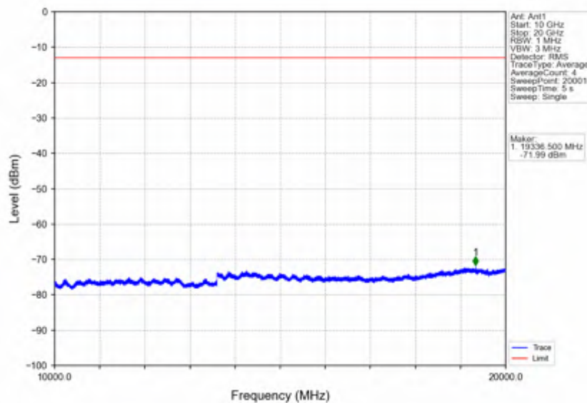
Band4_3MHz_QPSK_HCH_1753.5MHz_RB_1_0_NTNV
