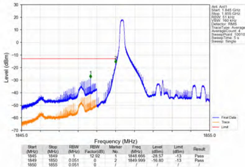
Band2_5MHz_QPSK_LCH_1852.5MHz_RB_1_0_NTNV
