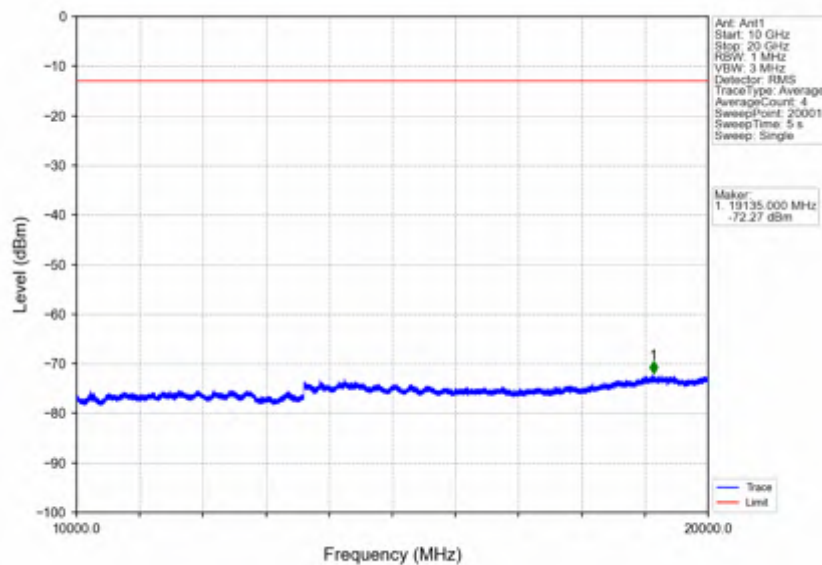
Band2_10MHz_256QAM_HCH_1905MHz_RB_1_0_NTV
