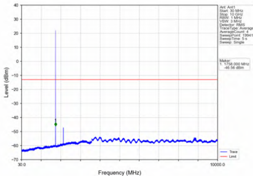
Band4_1.4MHz_16QAM_HCH_1754.3MHz_RB_1_0_NTNV
