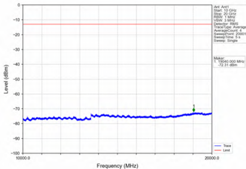
Band4_3MHz_256QAM_MCH_1732.5MHz_RB_1_0_NTNV
