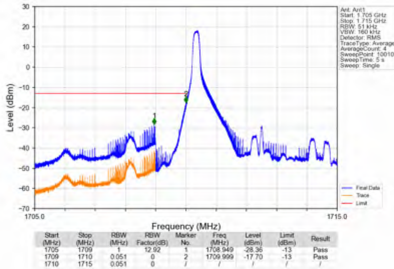
Band4_5MHz_QPSK_LCH_1712.5MHz_RB_1_0_NTNV
