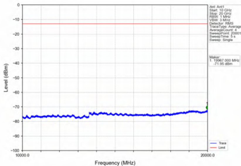
Band2_20MHz_64QAM_HCH_1900MHz_RB_1_0_NTNV
