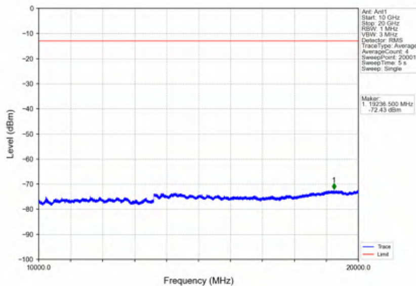
Band2_15MHz_64QAM_MCH_1880MHz_RB_1_0_NTNV
