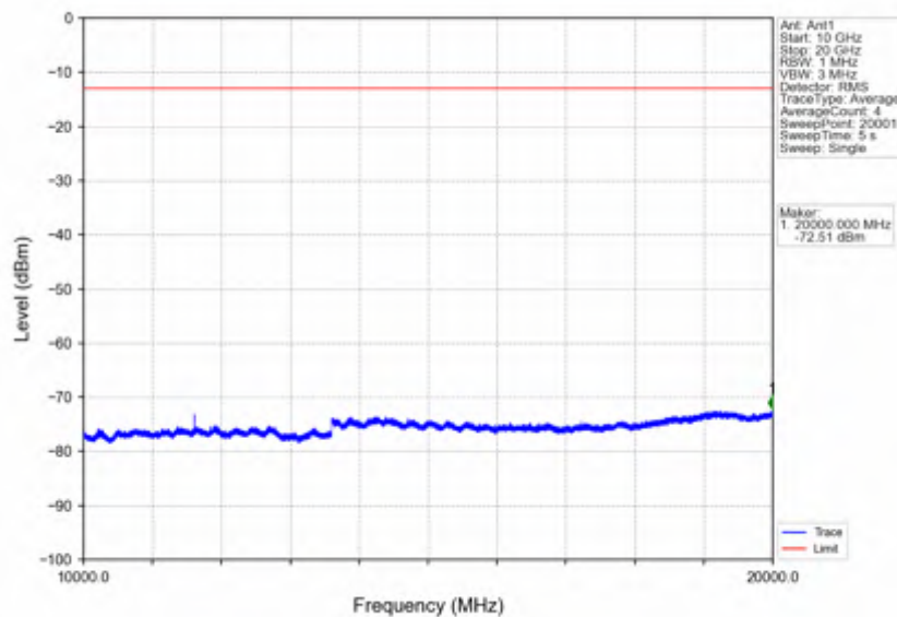
Band2_3MHz_64QAM_MCH_1880MHz_RB_1_0_NTNV
