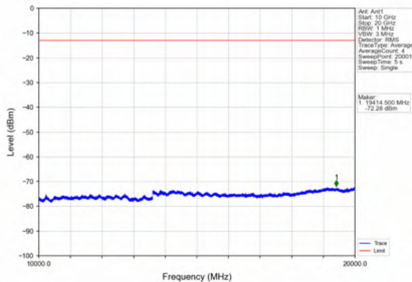
Band4_1.4MHz_64QAM_LCH_1710.7MHz_RB_6_0_NTNV
