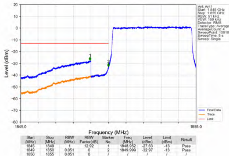
Band2_5MHz_256QAM_LCH_1852.5MHz_RB_25_0_NTNV
