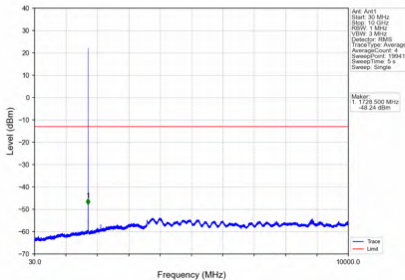
Band4 1.4MHz 64QAM MCH 1732.5MHz RB 1 0 NTNV
