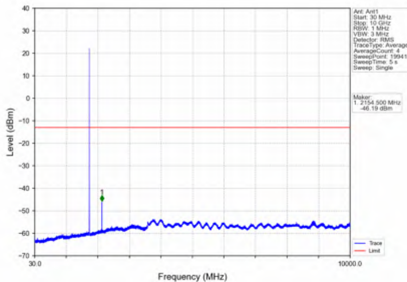
Band4_1.4MHz_QPSK_HCH_1754.3MHz_RB_1_0_NTNV
