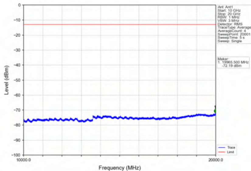
Band4_5MHz_256QAM_LCH_1712.5MHz_RB_25_0_NTNV
