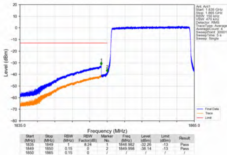
Band2_15MHz_256QAM_LCH_1857.5MHz_RB_75_0_NTNV
