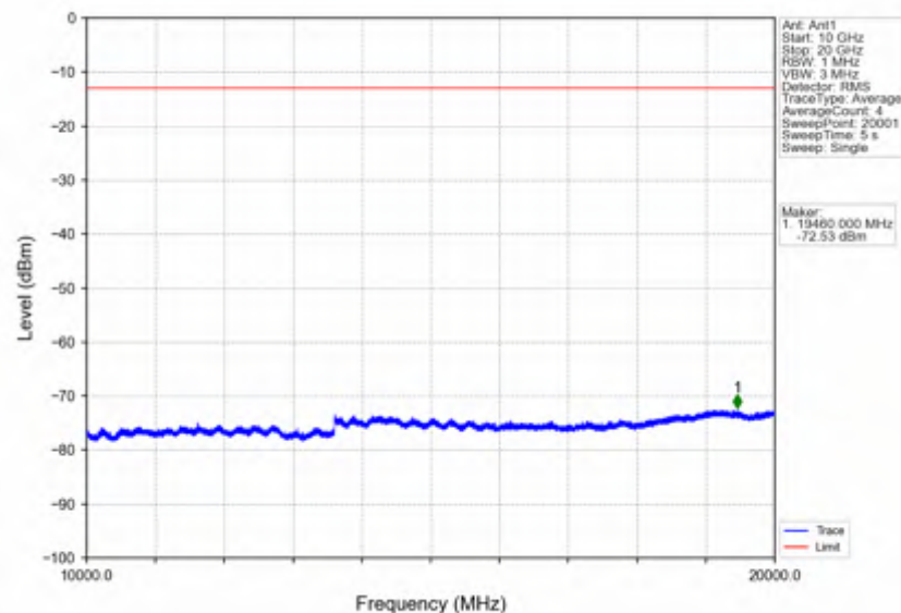
Band2_5MHz_256QAM_LCH_1852.5MHz_RB_25_0_NTNV
