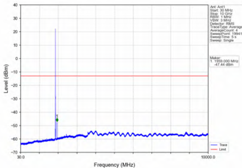
Band2_5MHz_16QAM_MCH_1880MHz_RB_1_0_NTNV
