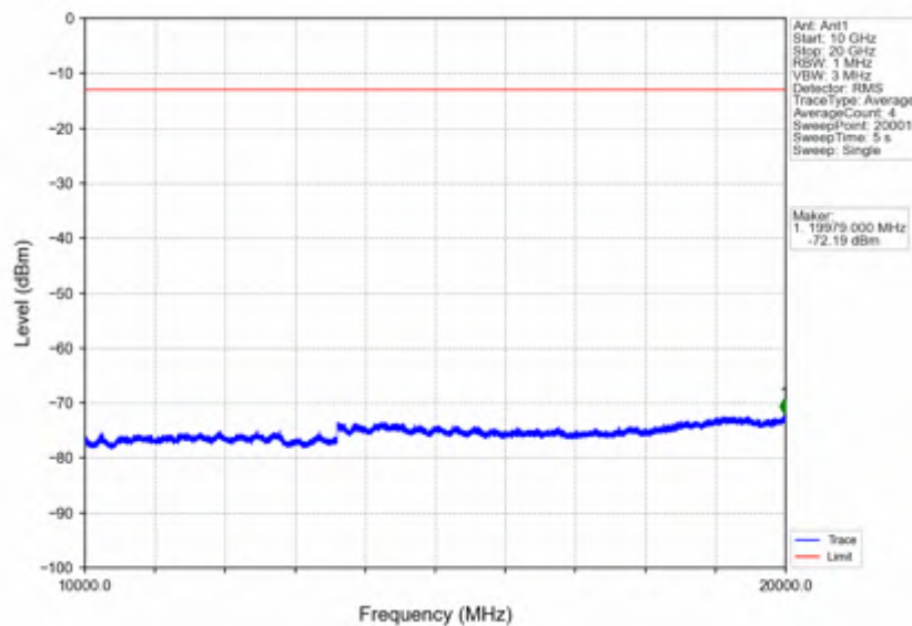
Band4_3MHz_16QAM_MCH_1732.5MHz_RB_1_0_NTNV
