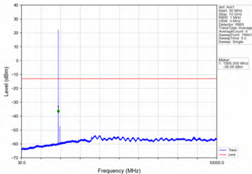
Band2_1.4MHz_16QAM_HCH_1909.3MHz_RB_1_0_NTNV
