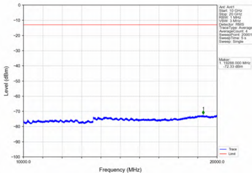
Band2_15MHz_256QAM_HCH_1902.5MHz_RB_1_0_NTNV
