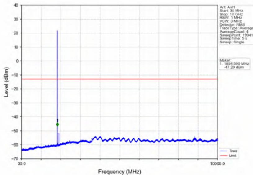
Band2_1.4MHz_64QAM_LCH_1850.7MHz_RB_1_0_NTNV
