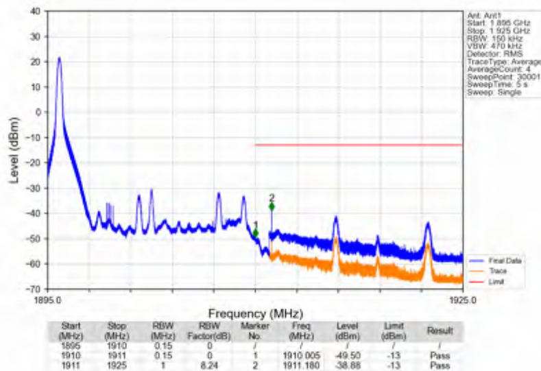
Band2_15MHz_QPSK_HCH_1902.5MHz_RB_75_0_NTNV
