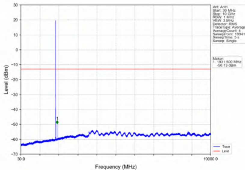
Band2_5MHz_256QAM_LCH_1852.5MHz_RB_1_0_NTNV
