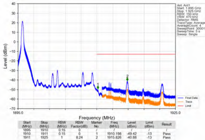
Band2_15MHz_64QAM_HCH_1902.5MHz_RB_1_74_NTNV
