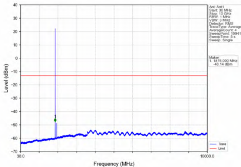
Band2_1.4MHz_16QAM_MCH_1880MHz_RB_1_0_NTNV
