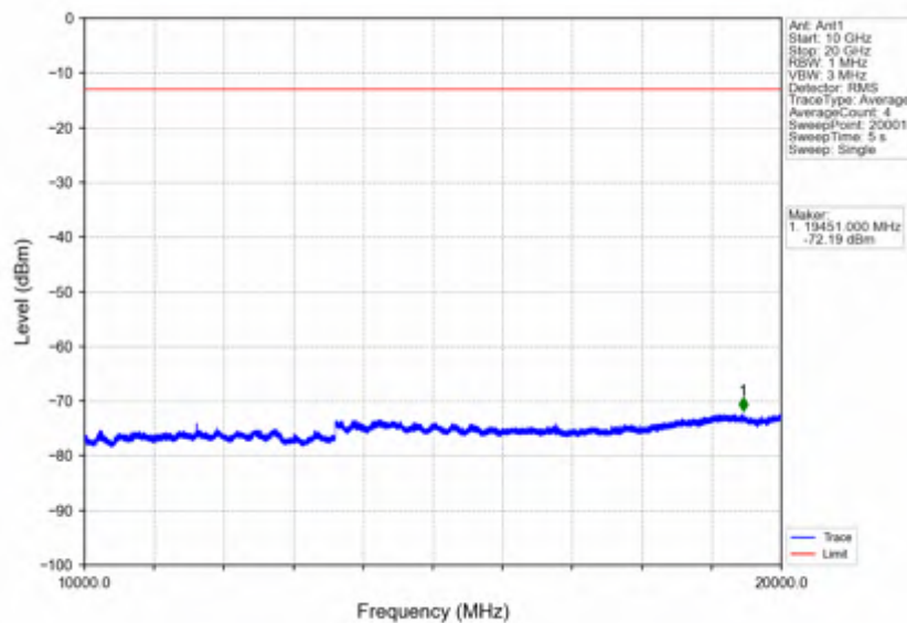
Band4_5MHz_16QAM_HCH_1752.5MHz_RB_1_0_NTNV
