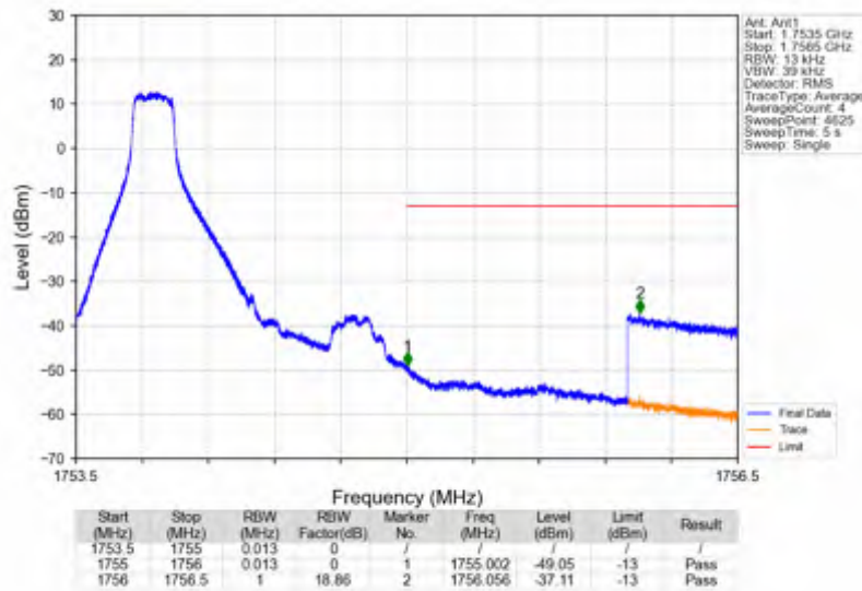
Band4_1.4MHz_64QAM_HCH_1754.3MHz_RB_1_5_NTNV
