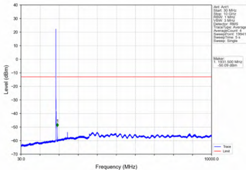
Band2_15MHz_16QAM_LCH_1857.5MHz_RB_1_0_NTNV
