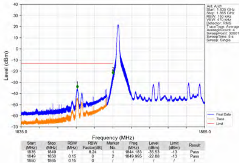
Band2_15MHz_64QAM_LCH_1857.5MHz_RB_75_0_NTNV
