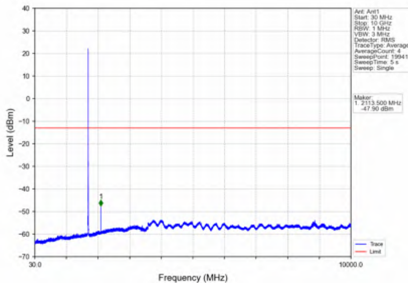
Band4 5MHz 64QAM LCH 1712.5MHz RB 1 0 NTNV
