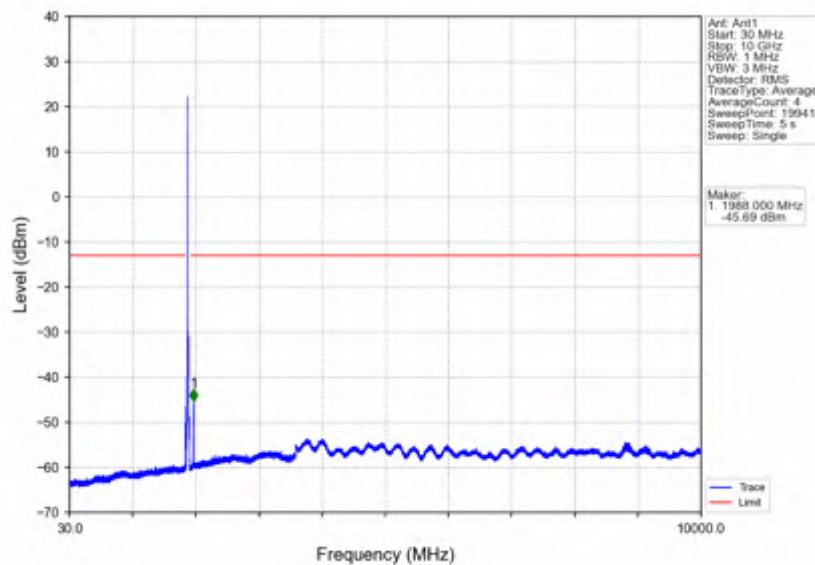
Band2_20MHz_64QAM_HCH_1900MHz_RB_1_0_NTNV
