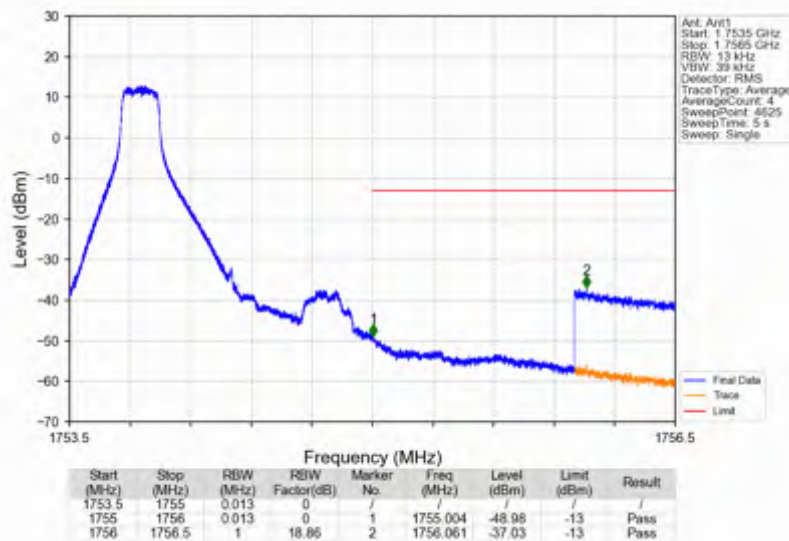
Band4_1.4MHz_16QAM_HCH_1754.3MHz_RB_6_0_NTNV
