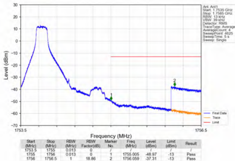
Band4_1.4MHz_QPSK_HCH_1754.3MHz_RB_6_0_NTNV
