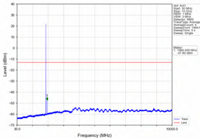
Band2_3MHz_64QAM_MCH_1880MHz_RB_1_0_NTNV
