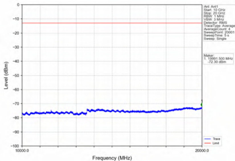
Band2_15MHz_256QAM_LCH_1857.5MHz_RB_75_0_NTNV
