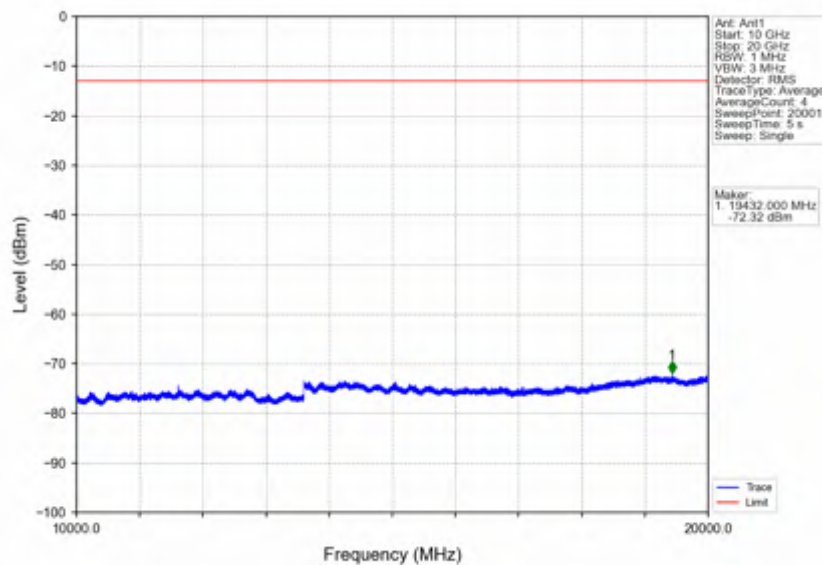
Band2_15MHz_64QAM_HCH_1902.5MHz_RB_1_0_NTNV
