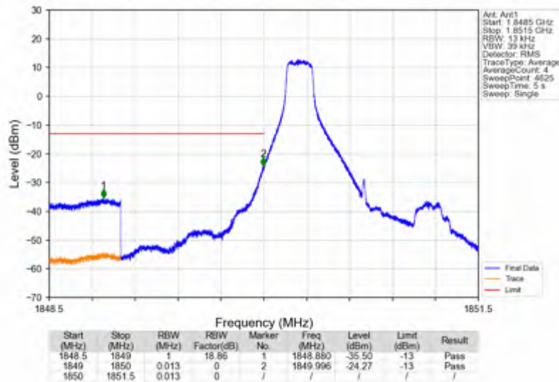
Band2_1.4MHz_16QAM_LCH_1850.7MHz_RB_1_0_NTNV
