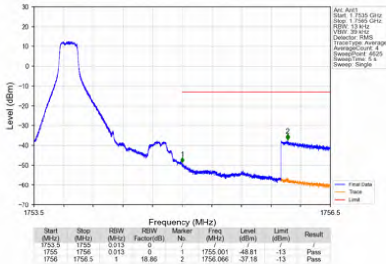
Band4_1.4MHz_QPSK_HCH_1754.3MHz_RB_1_5_NTNV
