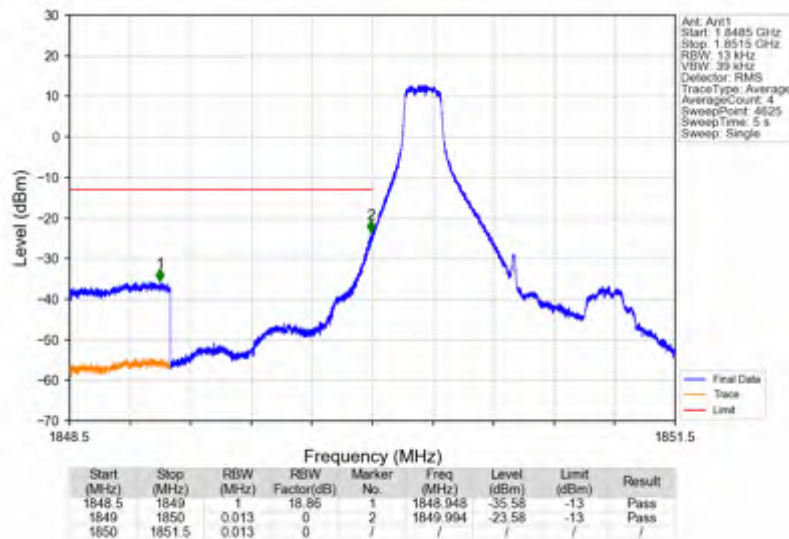
Band2_1.4MHz_QPSK_LCH_1850.7MHz_RB_1_0_NTNV
