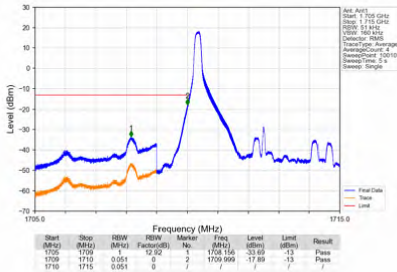
Band4 5MHz 64QAM LCH 1712.5MHz RB 1 0 NTNV
