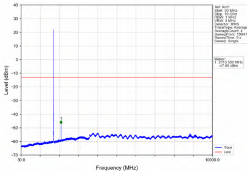
Band4_5MHz_16QAM_LCH_1712.5MHz_RB_1_0_NTNV
