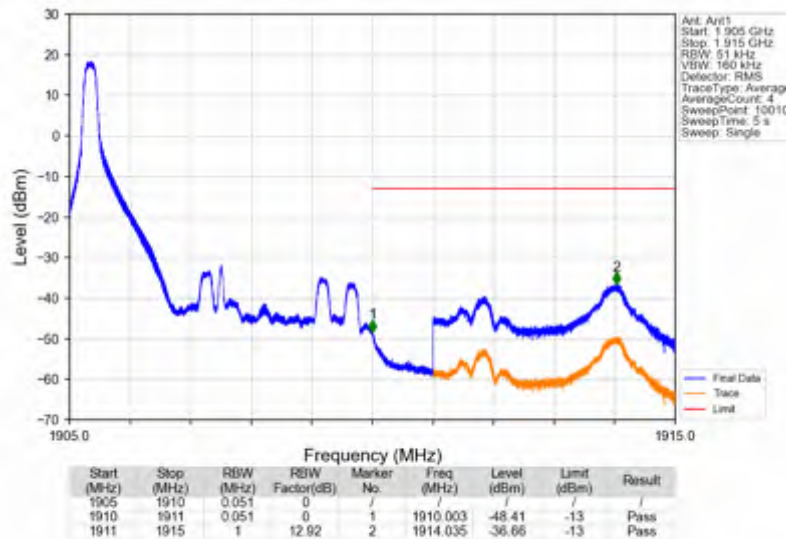
Band2_5MHz_QPSK_HCH_1907.5MHz_RB_1_24_NTNV
