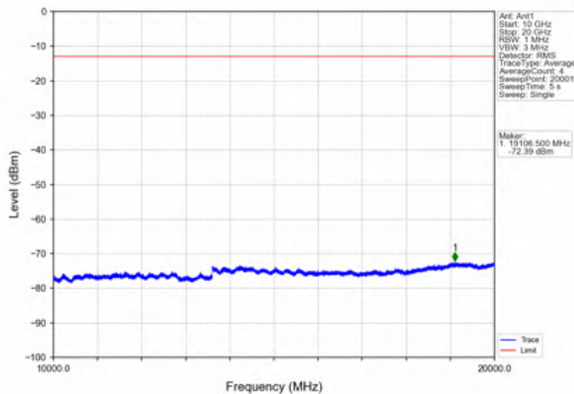
Band2_5MHz_64QAM_HCH_1907.5MHz_RB_1_0_NTNV
