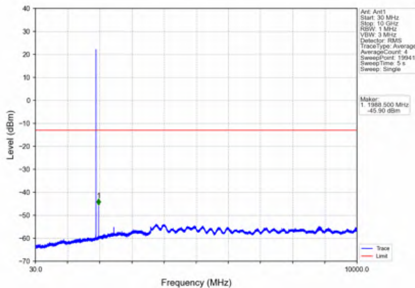
Band2_3MHz_16QAM_HCH_1908.5MHz_RB_1_0_NTNV
