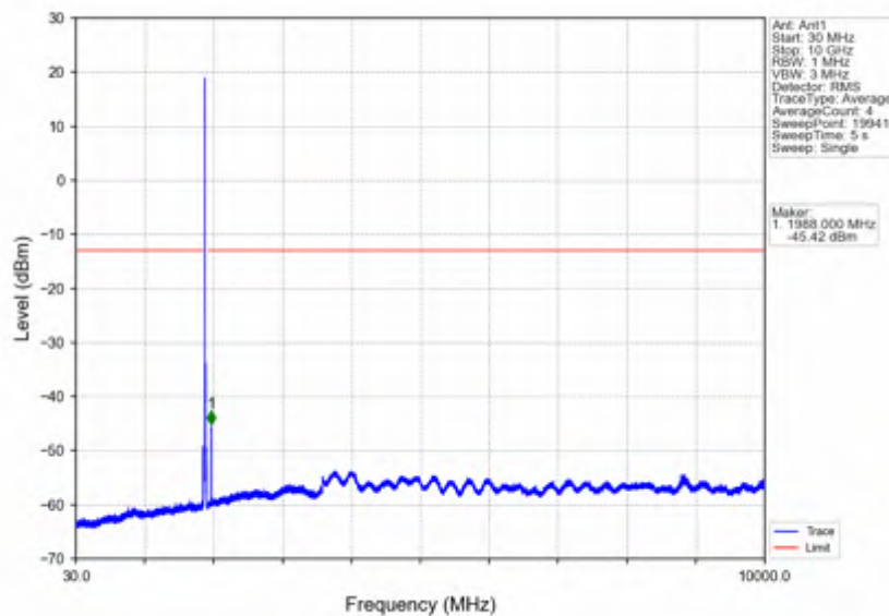
Band2_15MHz_256QAM_HCH_1902.5MHz_RB_1_0_NTNV
