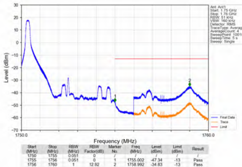
Band4_5MHz_QPSK_HCH_1752.5MHz_RB_25_0_NTNV
