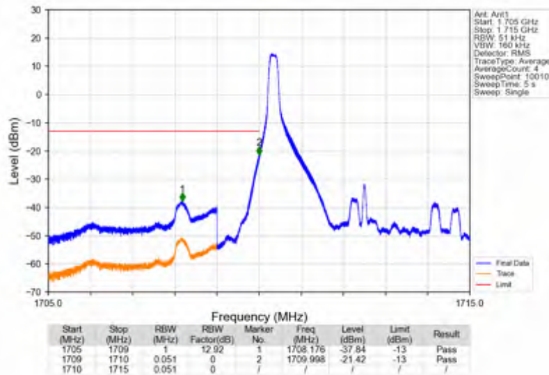
Band4 5MHz 256QAM LCH 1712.5MHz RB 1 0 NTN
