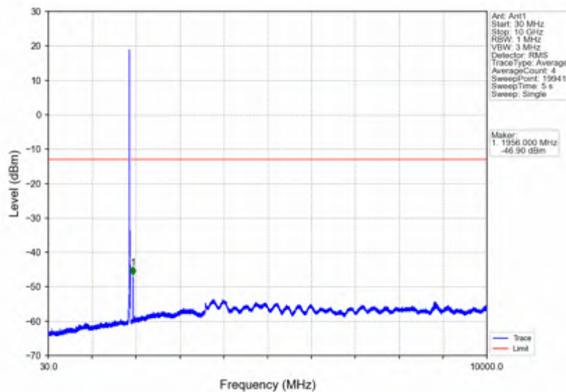
Band2_15MHz_256QAM_MCH_1880MHz_RB_1_0_NTNV
