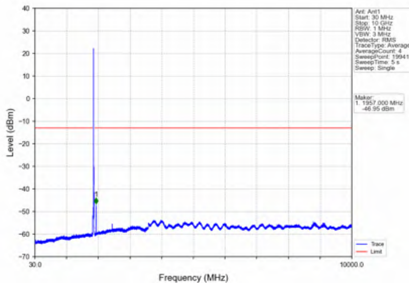
Band2_15MHz_64QAM_MCH_1880MHz_RB_1_0_NTNV
