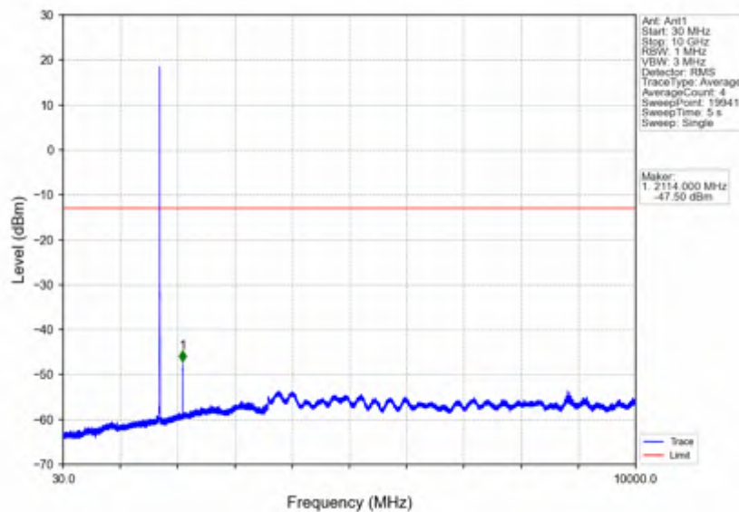
Band4 5MHz 256QAM LCH 1712.5MHz RB 1 0 NTNV
