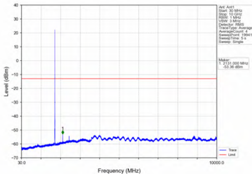
Band4_5MHz_16QAM_MCH_1732.5MHz_RB_1_0_NTNV
