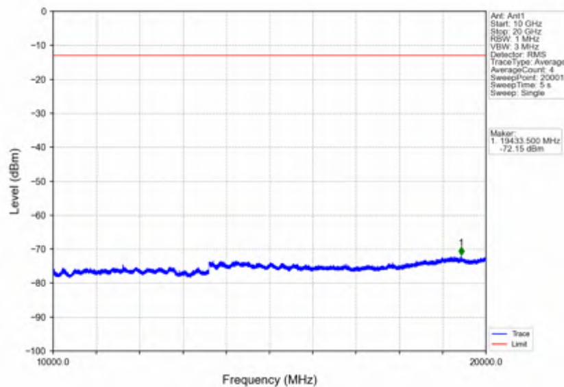
Band4_3MHz_16QAM_LCH_1711.5MHz_RB_15_0_NTNV
