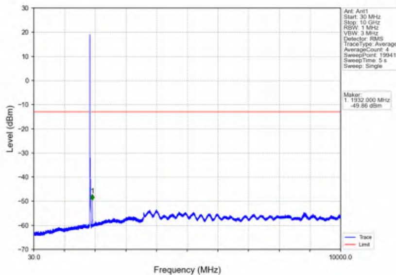
Band2_15MHz_256QAM_LCH_1857.5MHz_RB_1_0_NTNV
