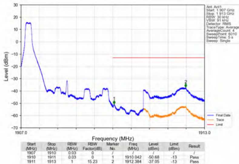
Band2_3MHz_64QAM_HCH_1908.5MHz_RB_15_0_NTNV
