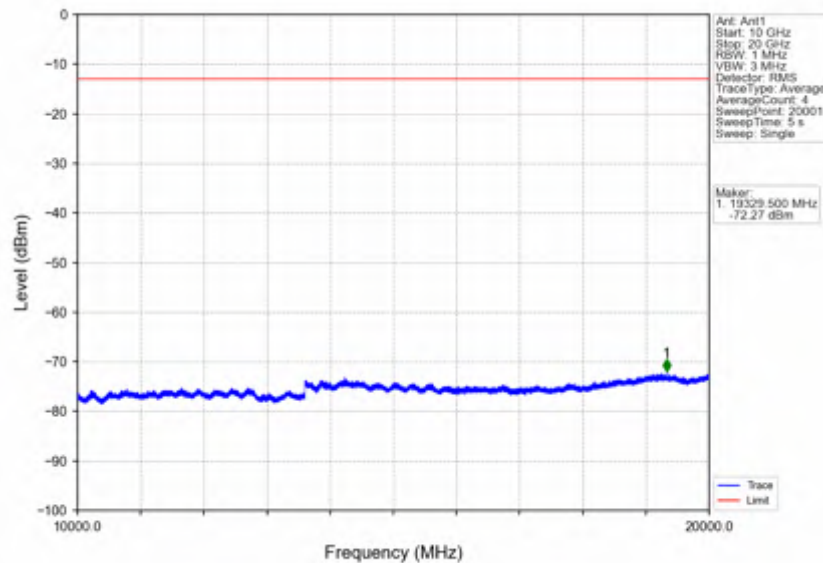
Band2_3MHz_16QAM_LCH_1851.5MHz_RB_15_0_NTNV
