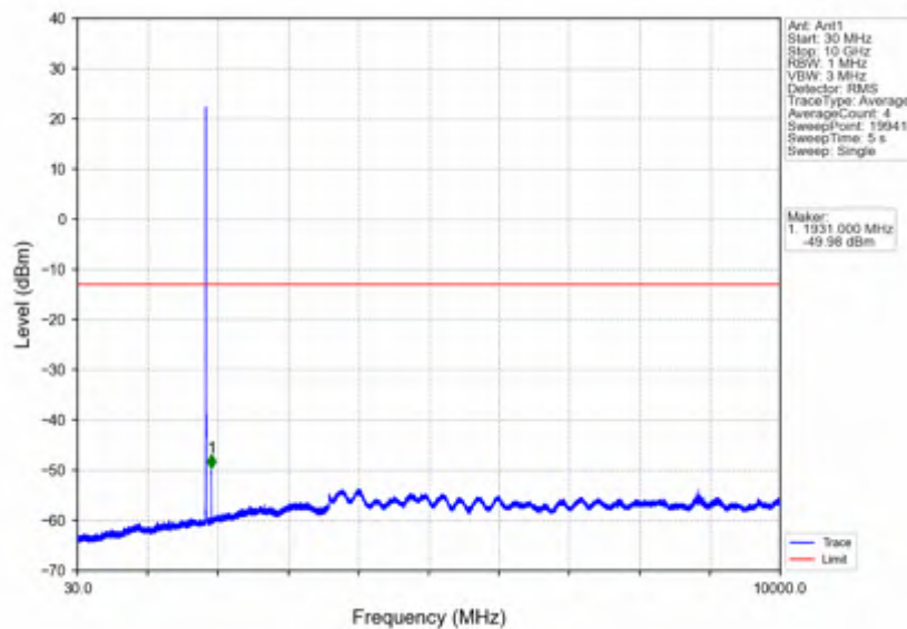
Band2_5MHz_64QAM_LCH_1852.5MHz_RB_1_0_NTNV
