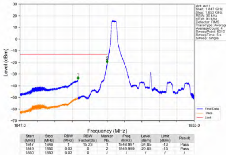
Band2_3MHz_64QAM_LCH_1851.5MHz_RB_1_0_NTNV
