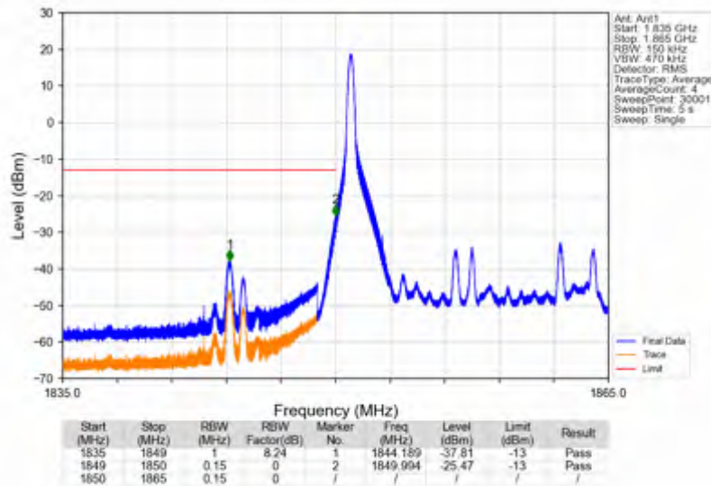
Band2_15MHz_256QAM_LCH_1857.5MHz_RB_1_0_NTNV
