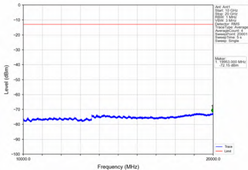
Band4_1.4MHz_256QAM_LCH_1710.7MHz_RB_6_0_NTNV
