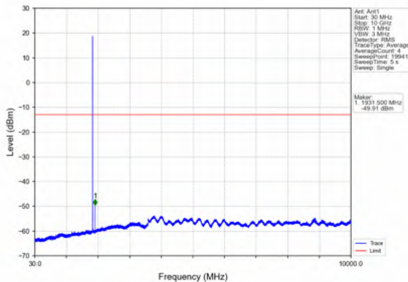
Band2_3MHz_256QAM_LCH_1851.5MHz_RB_1_0_NTNV
