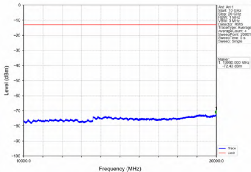
Band2_15MHz_64QAM_LCH_1857.5MHz_RB_75_0_NTNV
