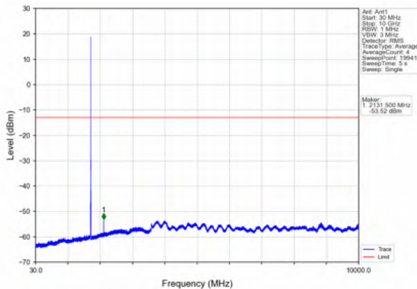
Band4_5MHz_256QAM_MCH_1732.5MHz_RB_1_0_NTNV
