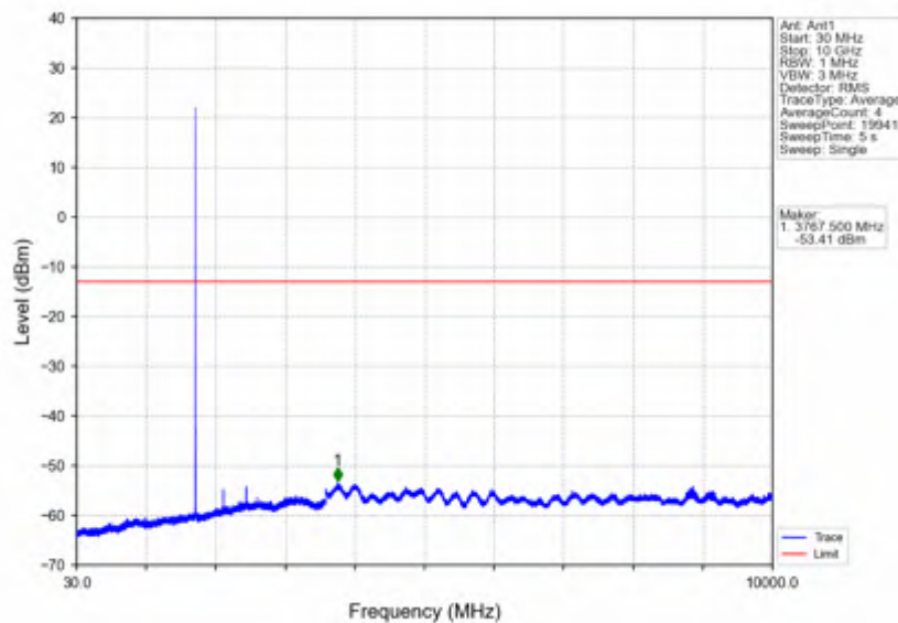
Band4_3MHz_64QAM_MCH_1732.5MHz_RB_1_0_NTNV
