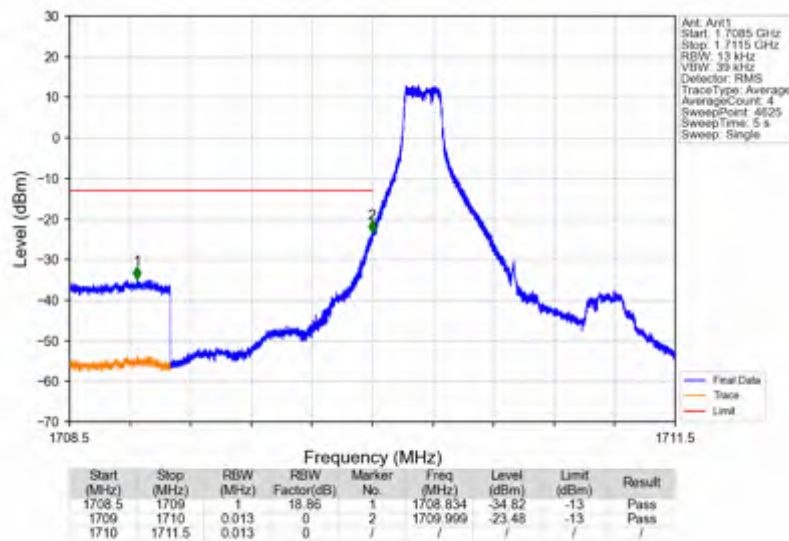
Band4_1.4MHz_64QAM_LCH_1710.7MHz_RB_6_0_NTNV
