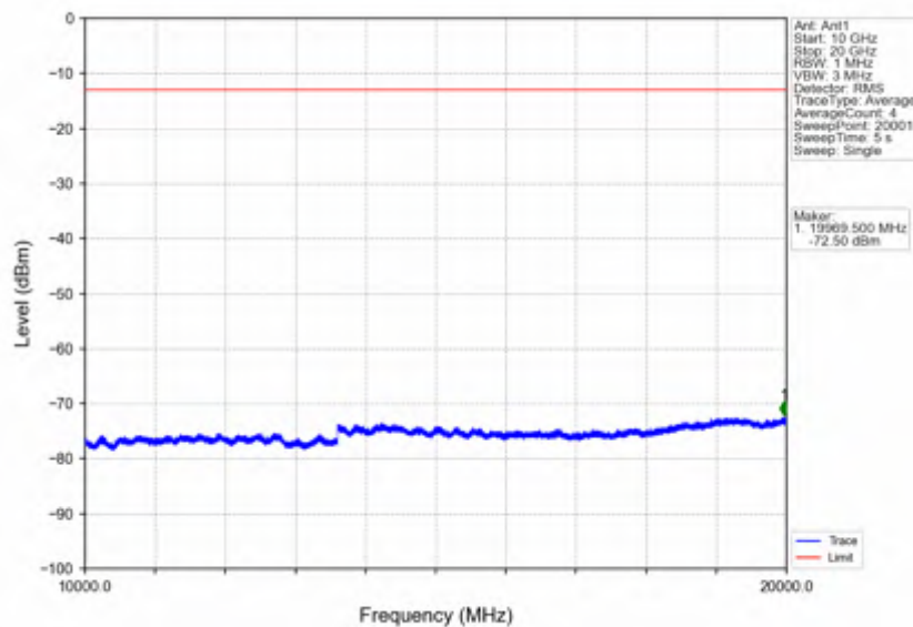
Band2_5MHz_256QAM_HCH_1907.5MHz_RB_1_0_NTNV
