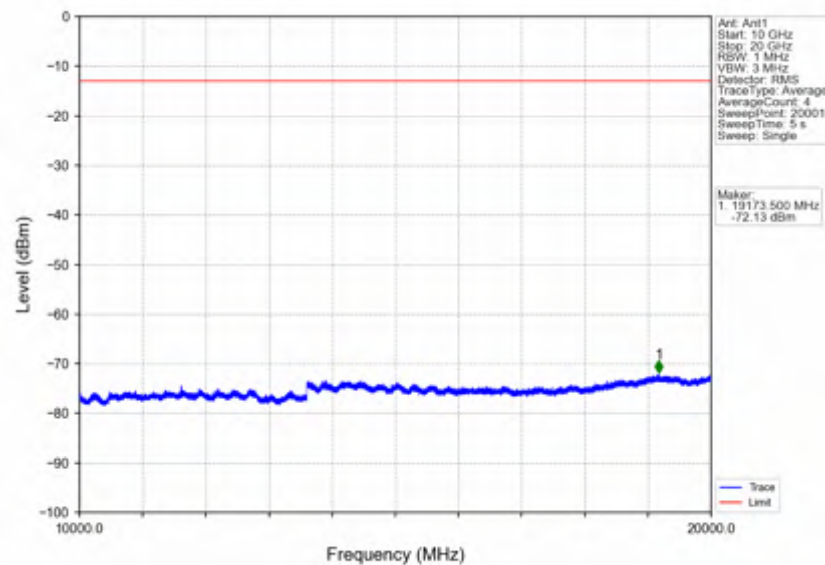
Band4_5MHz_64QAM_LCH_1712.5MHz_RB_25_0_NTNV
