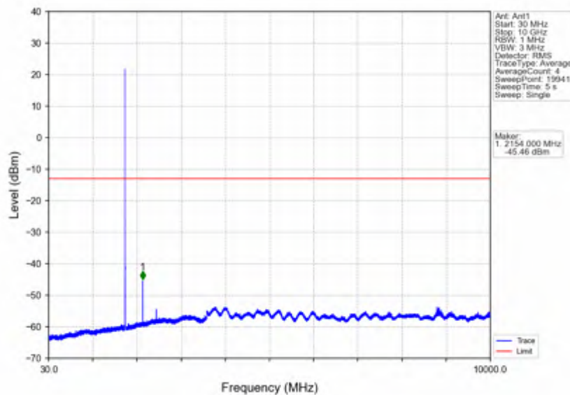
Band4_3MHz_QPSK_HCH_1753.5MHz_RB_1_0_NTNV
