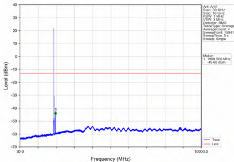
Band2_15MHz_16QAM_HCH_1902.5MHz_RB_1_0_NTNV
