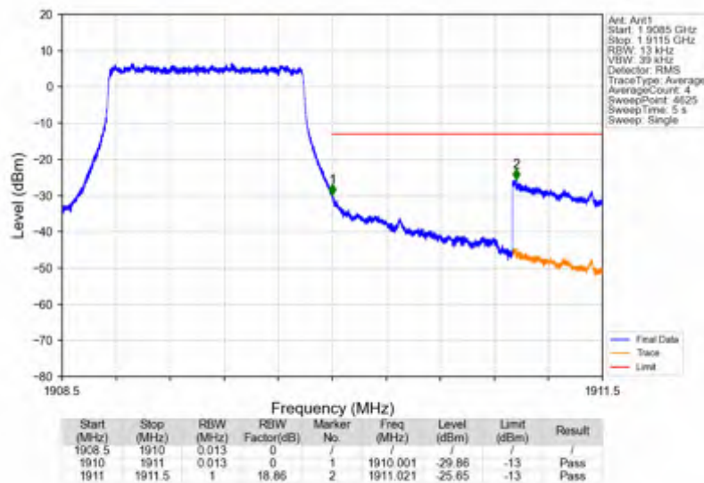
Band2_1.4MHz_64QAM_HCH_1909.3MHz_RB_6_0_NTNV
