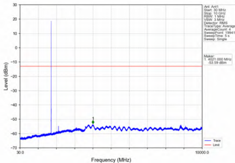
Band4_3MHz_256QAM_MCH_1732.5MHz_RB_1_0_NTNV
