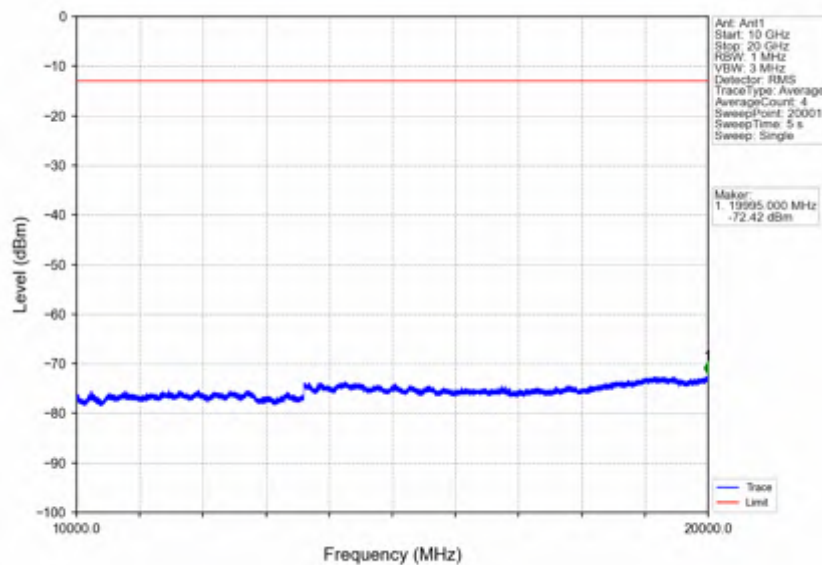
Band2_5MHz_256QAM_MCH_1880MHz_RB_1_0_NTNV
