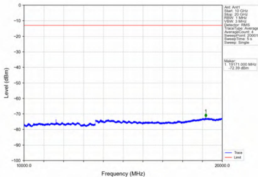
Band2_1.4MHz_256QAM_HCH_1909.3MHz_RB_1_0_NTNV
