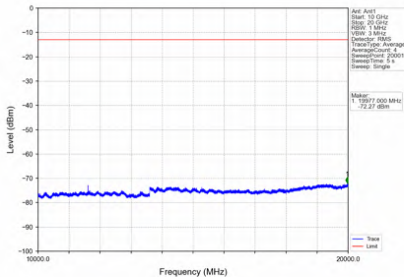
Band4_5MHz_16QAM_LCH_1712.5MHz_RB_25_0_NTNV
