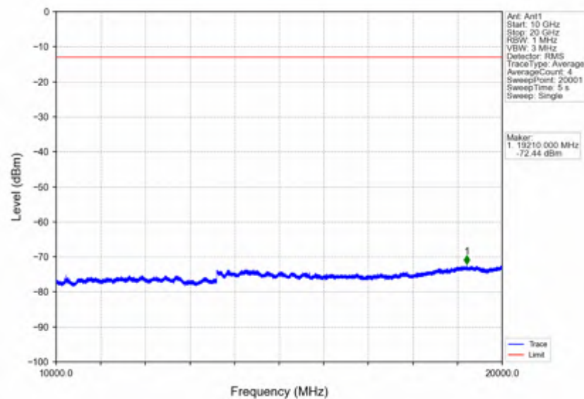
Band2_1.4MHz_64QAM_LCH_1850.7MHz_RB_6_0_NTNV
