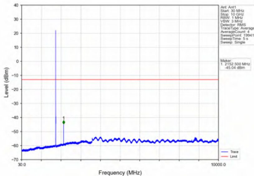
Band4_5MHz_QPSK_HCH_1752.5MHz_RB_1_0_NTNV
