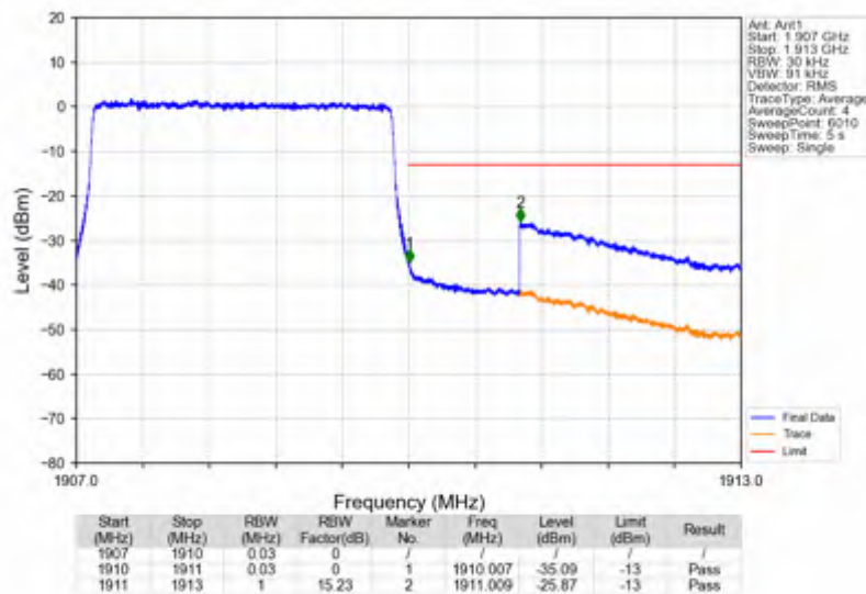
Band2_3MHz_256QAM_HCH_1908.5MHz_RB_15_0_NTNV
