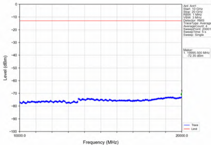
Band2_10MHz_64QAM_MCH_1880MHz_RB_1_0_NTNV
