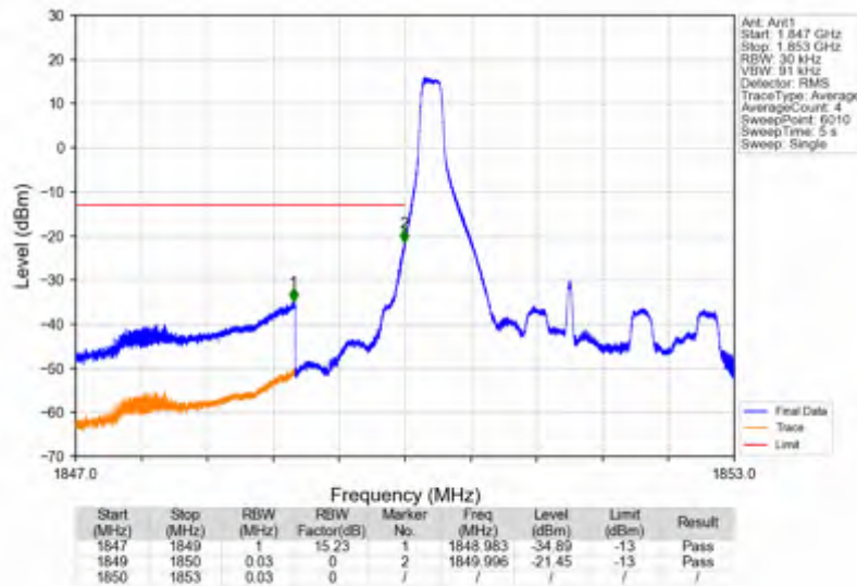
Band2_3MHz_16QAM_LCH_1851.5MHz_RB_15_0_NTNV
