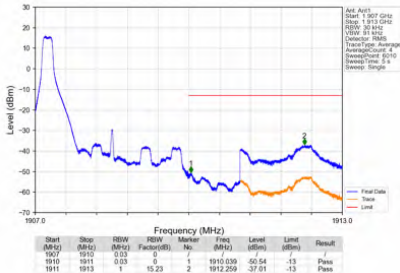
Band2_3MHz_16QAM_HCH_1908.5MHz_RB_1_14_NTNV
