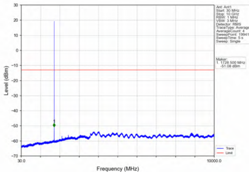
Band4_1.4MHz_256QAM_MCH_1732.5MHz_RB_1_0_NTNV
