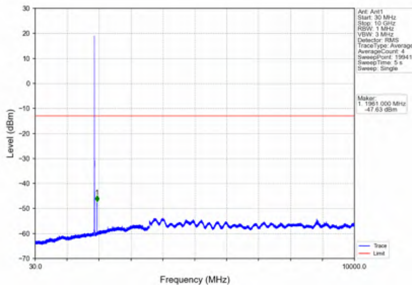
Band2_5MHz_256QAM_MCH_1880MHz_RB_1_0_NTNV
