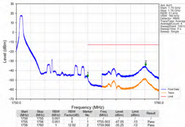
Band4_5MHz_64QAM_HCH_1752.5MHz_RB_25_0_NTNV
