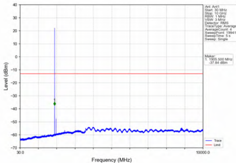
Band2_1.4MHz_64QAM_HCH_1909.3MHz_RB_1_0_NTNV
