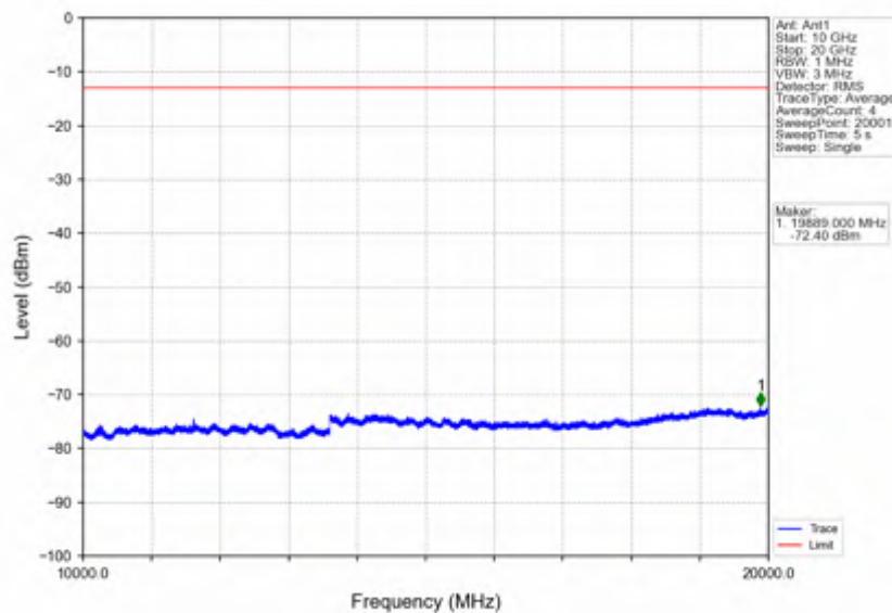
Band2_5MHz_16QAM_HCH_1907.5MHz_RB_1_0_NTNV
