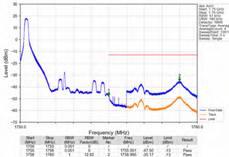
Band4_5MHz_QPSK_HCH_1752.5MHz_RB_1_24_NTNV
