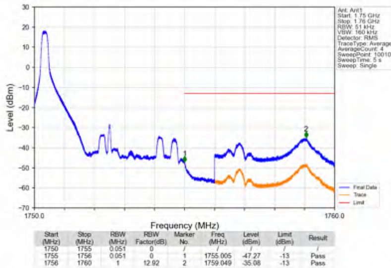
Band4_5MHz_16QAM_HCH_1752.5MHz_RB_25_0_NTNV
