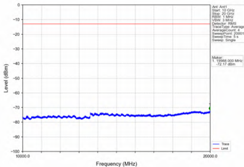
Band4_3MHz_64QAM_HCH_1753.5MHz_RB_1_0_NTNV
