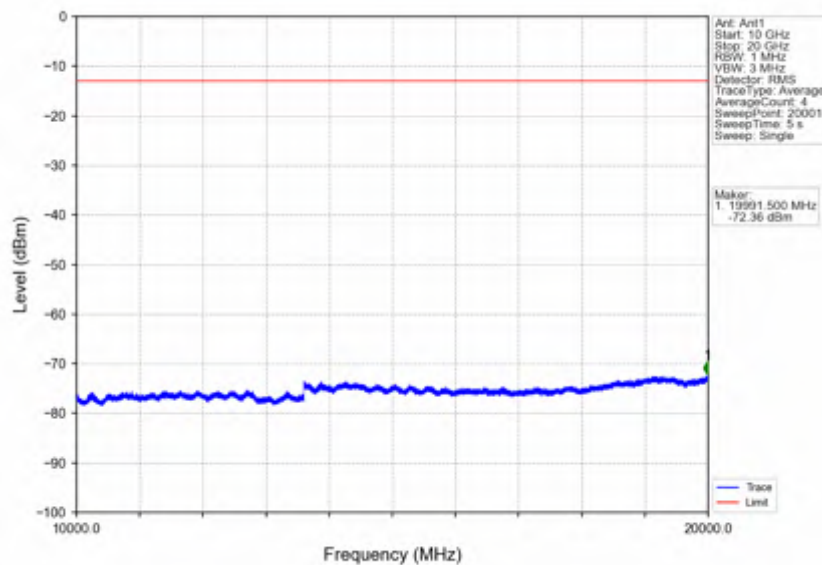
Band2_5MHz_64QAM_MCH_1880MHz_RB_1_0_NTNV
