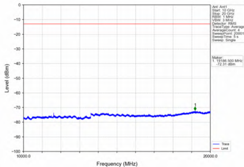
Band2_3MHz_64QAM_LCH_1851.5MHz_RB_15_0_NTNV
