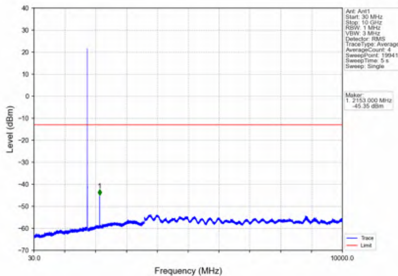
Band4_3MHz_64QAM_HCH_1753.5MHz_RB_1_0_NTNV
