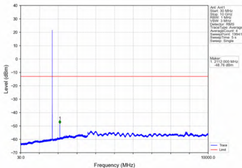
Band4_3MHz_QPSK_LCH_1711.5MHz_RB_1_0_NTNV
