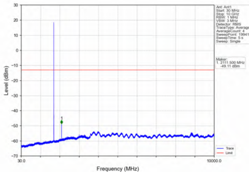
Band4_3MHz_256QAM_LCH_1711.5MHz_RB_1_0_NTNV
