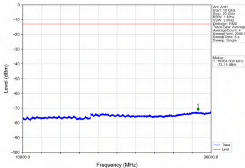
Band4_5MHz_16QAM_MCH_1732.5MHz_RB_1_0_NTNV
