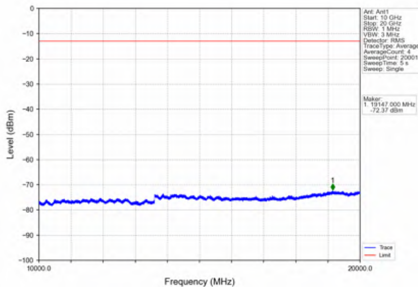
Band2_1.4MHz_64QAM_HCH_1909.3MHz_RB_1_0_NTNV
