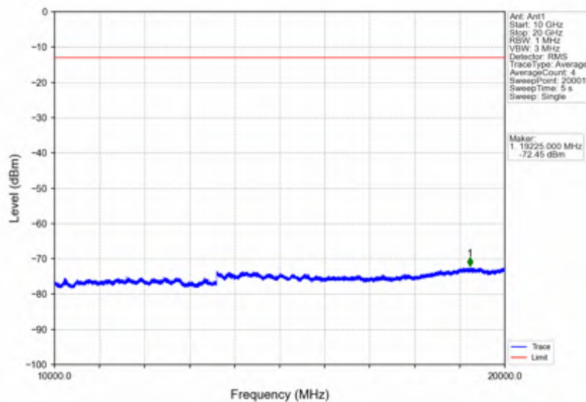
Band2_10MHz_64QAM_HCH_1905MHz_RB_1_0_NTNV
