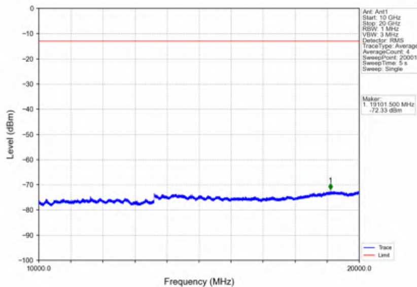
Band2_3MHz_64QAM_HCH_1908.5MHz_RB_1_0_NTNV
