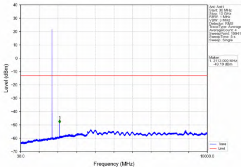
Band4 3MHz 16QAM LCH 1711.5MHz RB 1 0 NTNV
