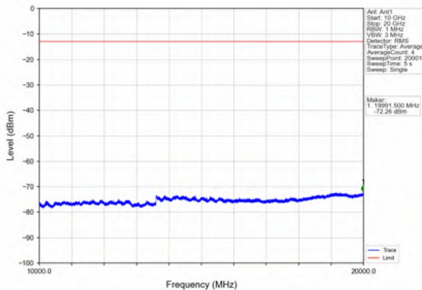
Band4_5MHz_QPSK_HCH_1752.5MHz_RB_1_0_NTNV
