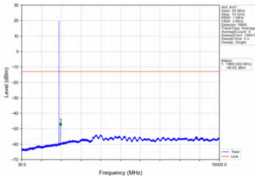
Band2_1.4MHz_256QAM_HCH_1909.3MHz_RB_1_0_NTNV
