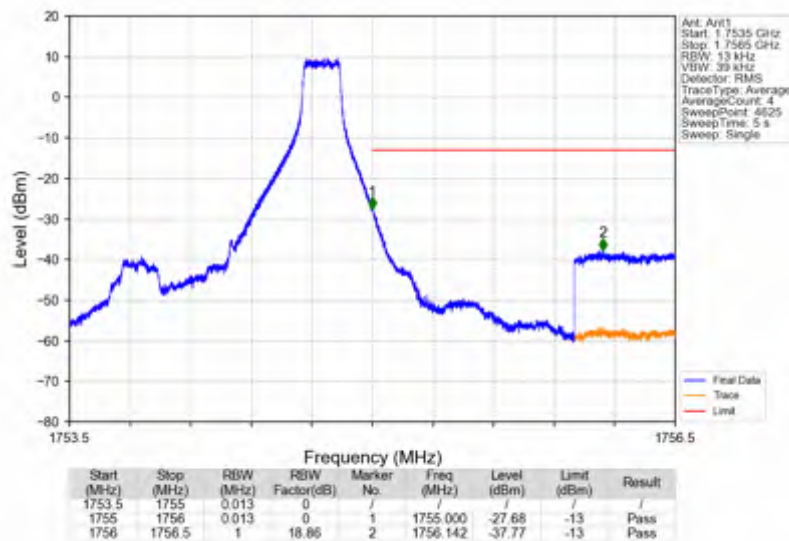
Band4 1.4MHz 256QAM HCH 1754.3MHz RB 1 5 NTNV
