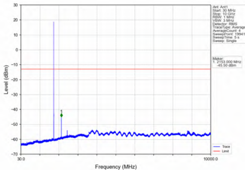
Band4_3MHz_256QAM_HCH_1753.5MHz_RB_1_0_NTNV
