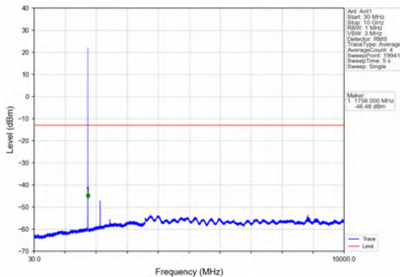
Band4_1.4MHz_64QAM_HCH_1754.3MHz_RB_1_0_NTNV
