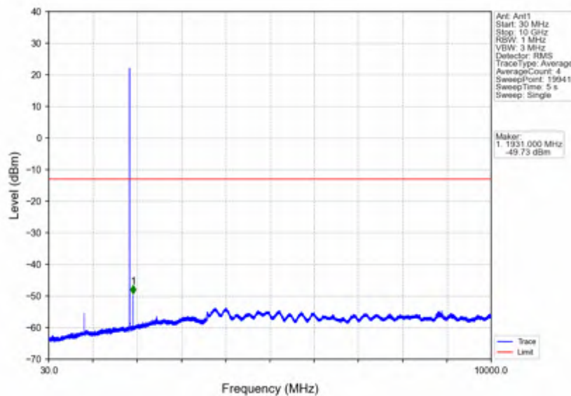
Band2_3MHz_16QAM_LCH_1851.5MHz_RB_1_0_NTNV
