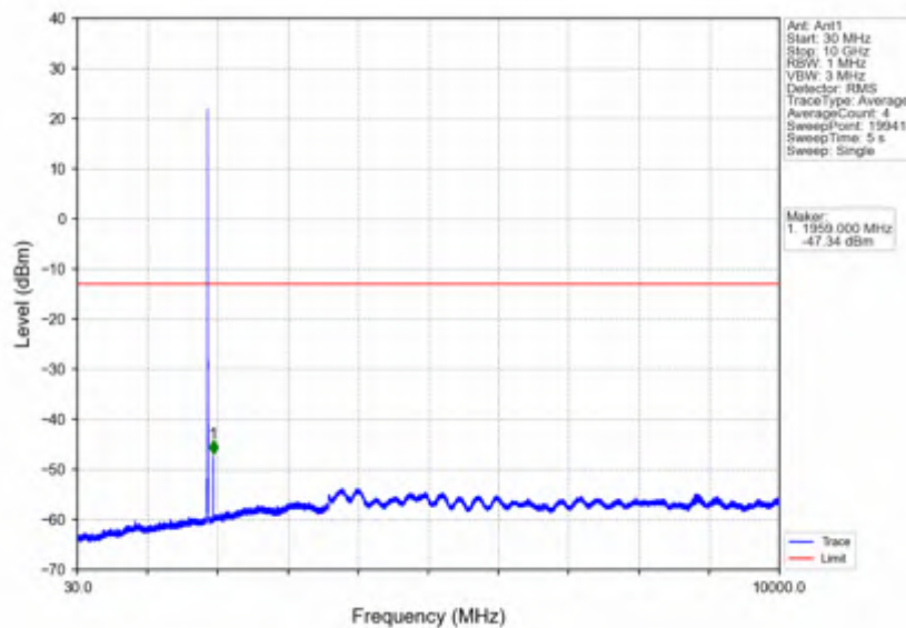
Band2_5MHz_64QAM_MCH_1880MHz_RB_1_0_NTNV
