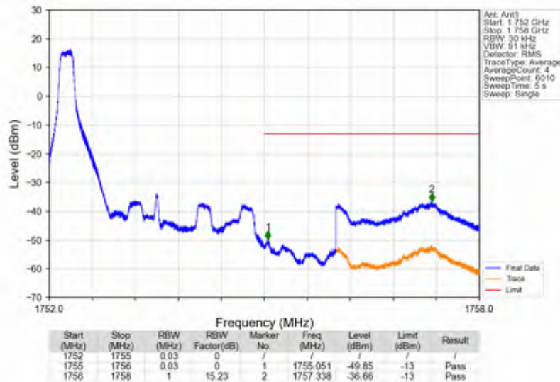
Band4_3MHz_64QAM_HCH_1753.5MHz_RB_1_14_NTNV
