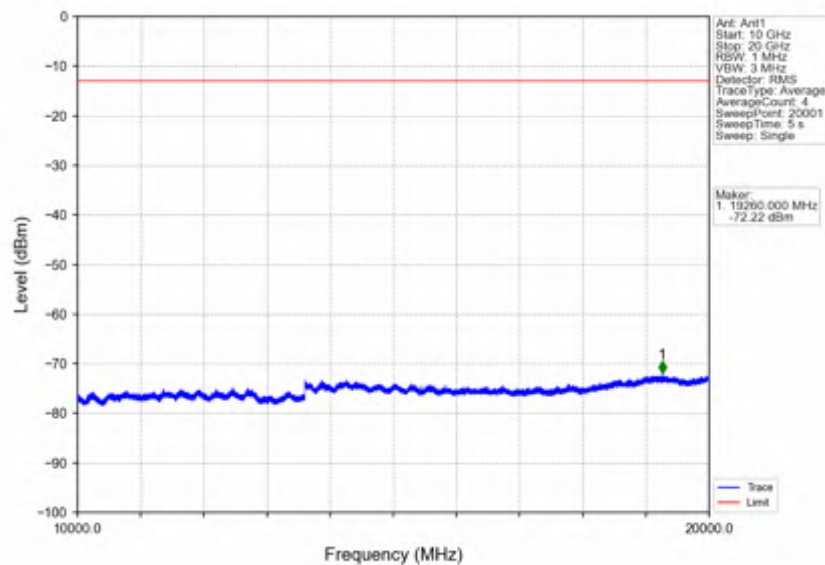
Band4_3MHz_64QAM_LCH_1711.5MHz_RB_15_0_NTNV
