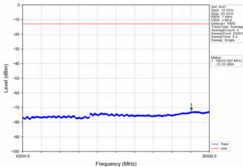
Band4_3MHz_QPSK_MCH_1732.5MHz_RB_1_0_NTNV
