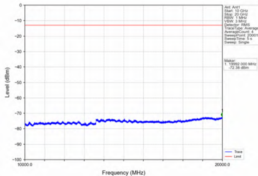
Band4_5MHz_QPSK_LCH_1712.5MHz_RB_25_0_NTNV
