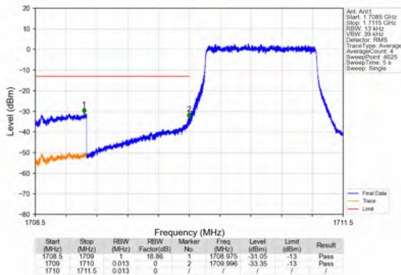
Band4_1.4MHz_256QAM_LCH_1710.7MHz_RB_6_0_NTNV
