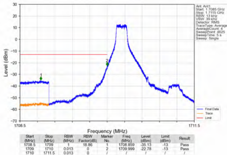
Band4_1.4MHz_QPSK_LCH_1710.7MHz_RB_1_0_NTNV
