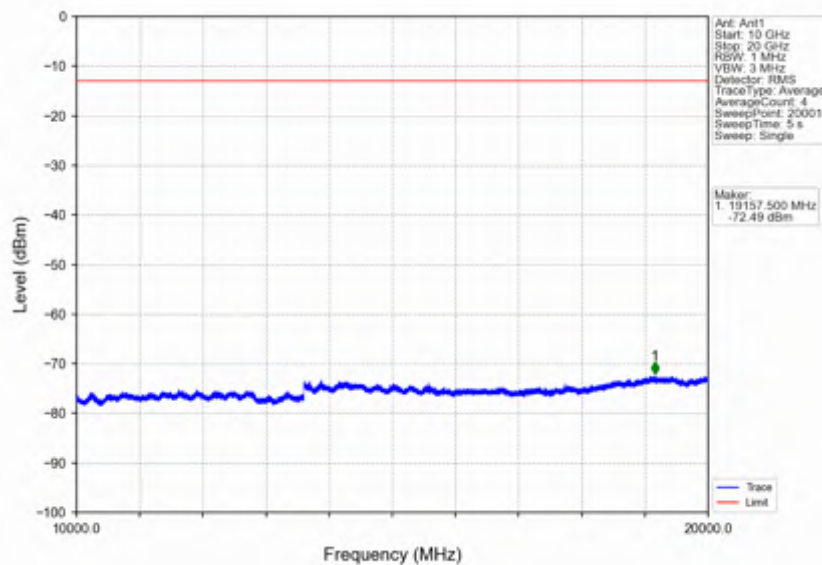
Band2_5MHz_16QAM_MCH_1880MHz_RB_1_0_NTNV
