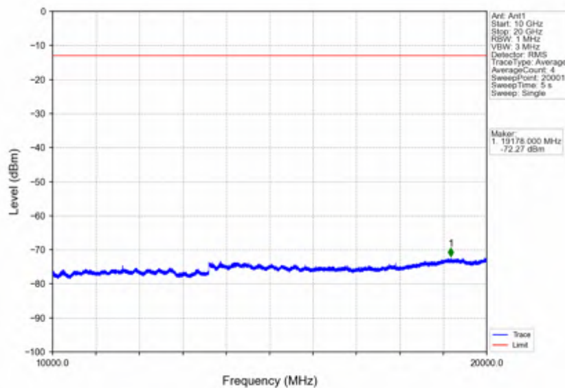
Band2_3MHz_16QAM_HCH_1908.5MHz_RB_1_0_NTNV
