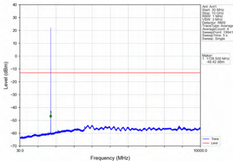
Band4_1.4MHz_16QAM_MCH_1732.5MHz_RB_1_0_NTNV
