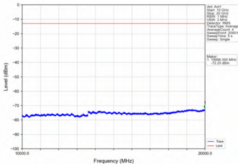
Band2_1.4MHz_64QAM_MCH_1880MHz_RB_1_0_NTNV
