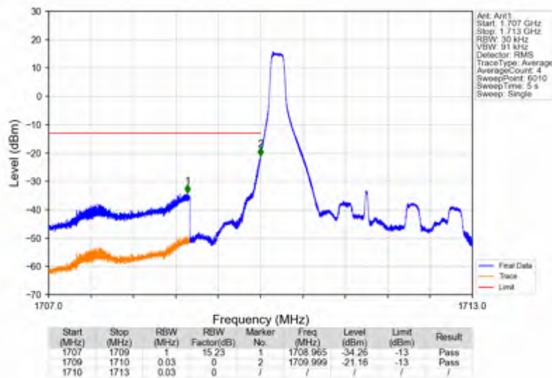
Band4_3MHz_16QAM_LCH_1711.5MHz_RB_15_0_NTNV
