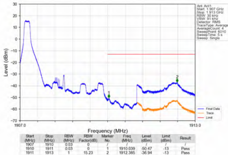
Band2_3MHz_16QAM_HCH_1908.5MHz_RB_15_0_NTNV
