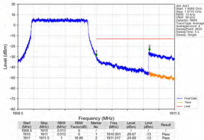
Band2_1.4MHz_16QAM_HCH_1909.3MHz_RB_6_0_NTNV
