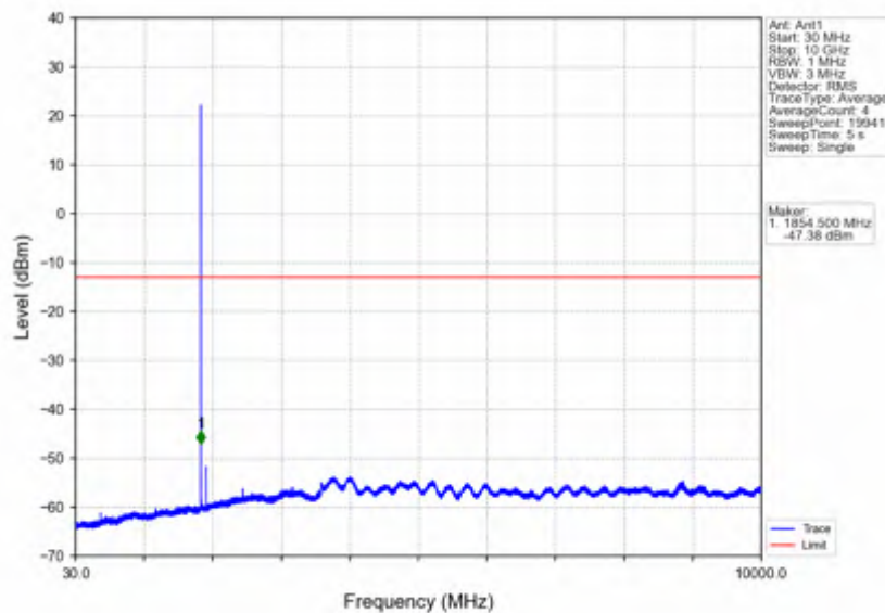
Band2_1.4MHz_16QAM_LCH_1850.7MHz_RB_1_0_NTNV
