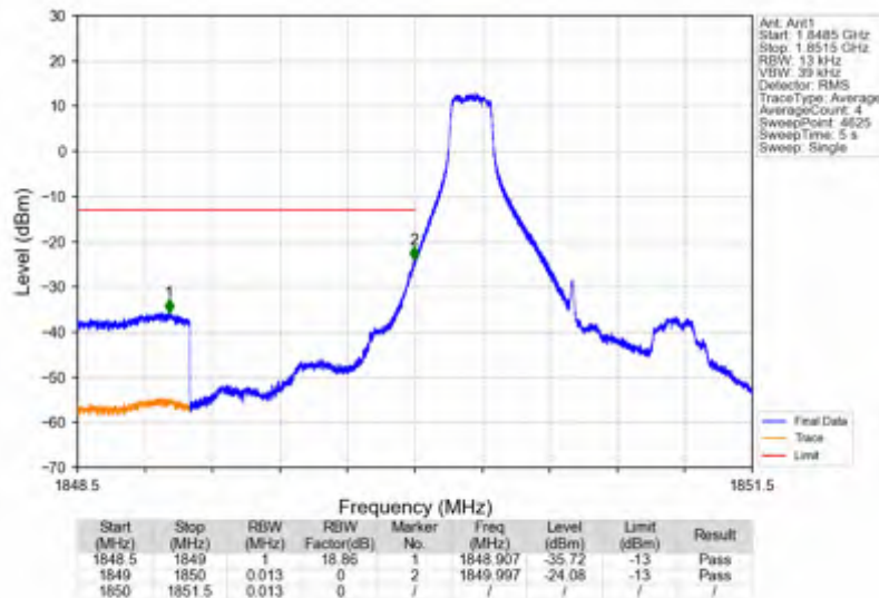
Band2_1.4MHz_16QAM_LCH_1850.7MHz_RB_6_0_NTNV
