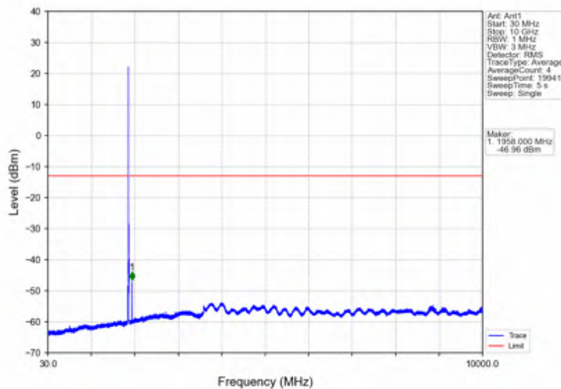
Band2_10MHz_64QAM_MCH_1880MHz_RB_1_0_NTNV
