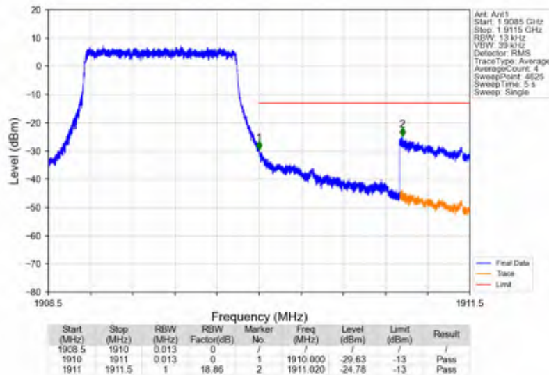
Band2_1.4MHz_16QAM_HCH_1909.3MHz_RB_1_5_NTNV
