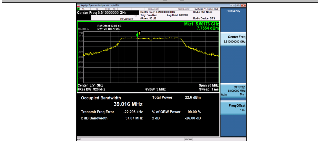
11AC40SISO_Ant1_5510
