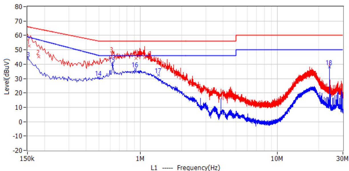
L Line
