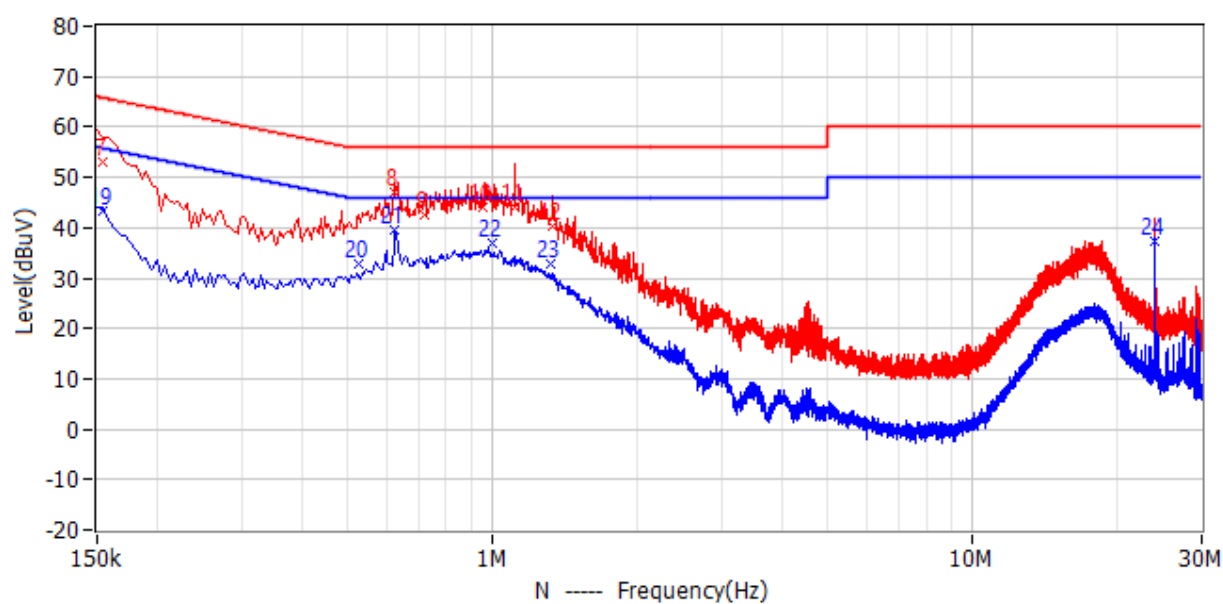
N Line
