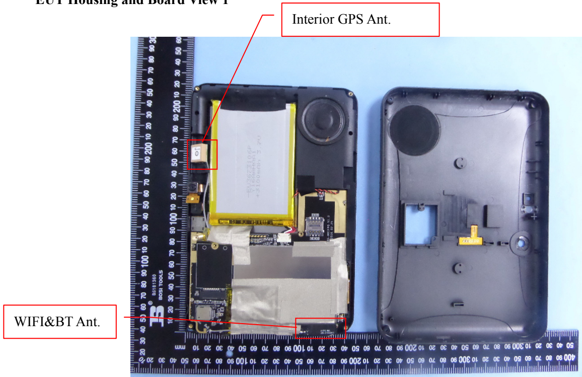
EUT Housing and Board View 1
