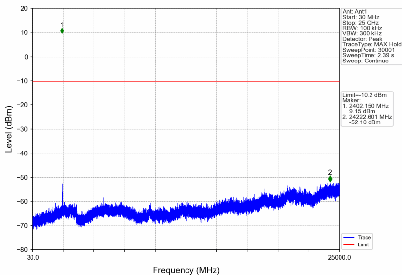
1M_LCH_2402MHz_Ant1_NTNV
