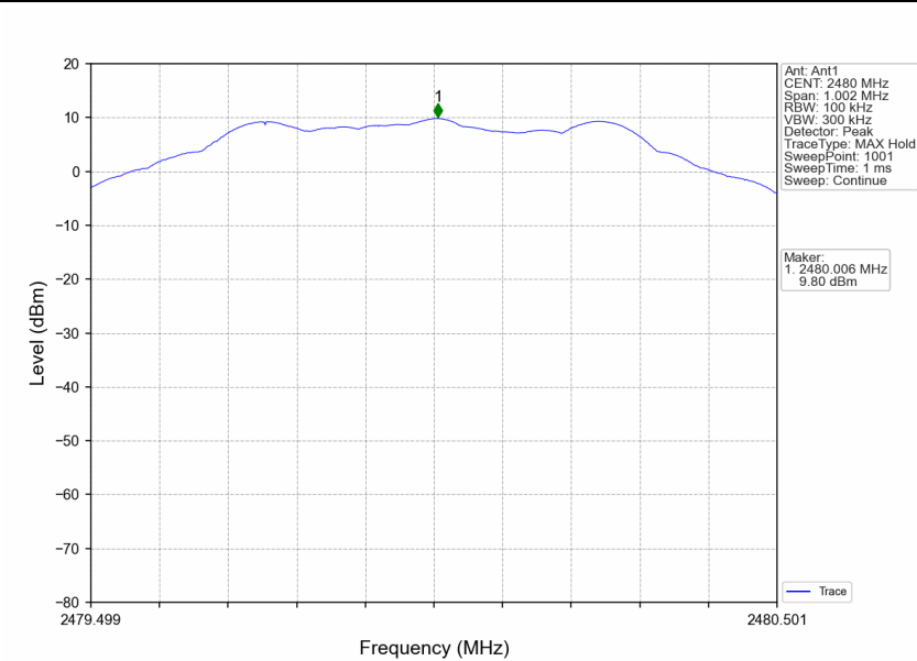
1M_HCH_2480MHz_Ant1_NTNV
