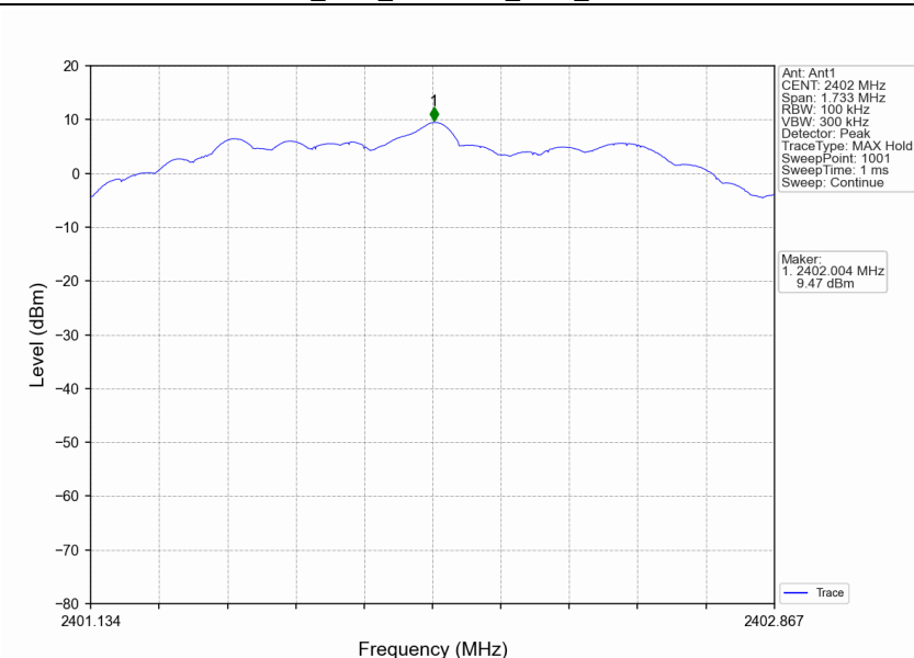
2M_LCH_2402MHz_Ant1_NTNV
