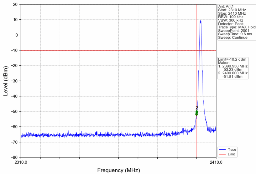
1M_LCH_2402MHz_Ant1_NTNV
