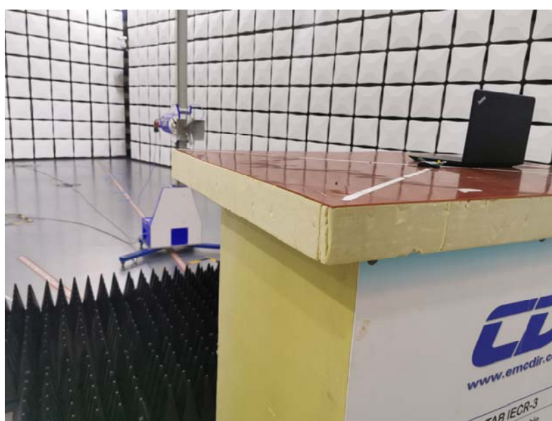
Spurious Radiated Emissions Test setup (1GHz~25GHz)
