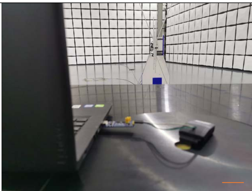
Spurious Radiated Emissions Test setup (below 1GHz)
