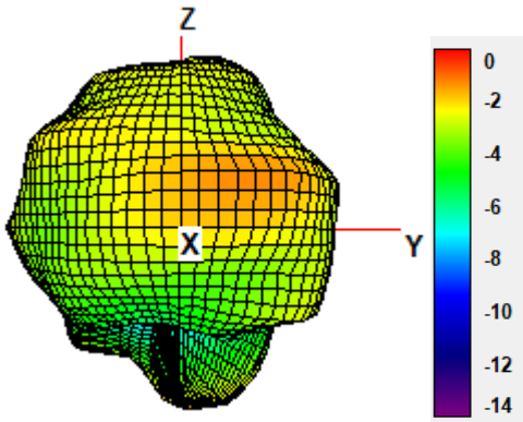
Max Antenna 3D Radiation Pattern 2400-2500 MHz
