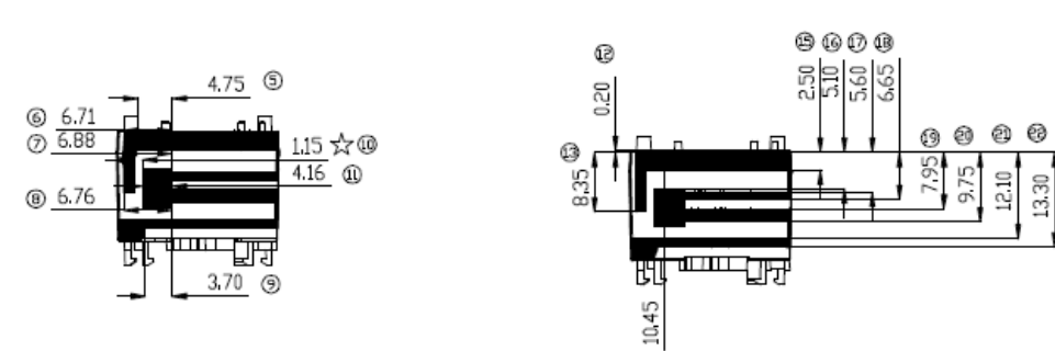
LoRa / BLE2 Antenna Drawing:
