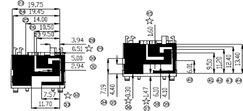
GPS / BLE1 Antenna Drawing:
