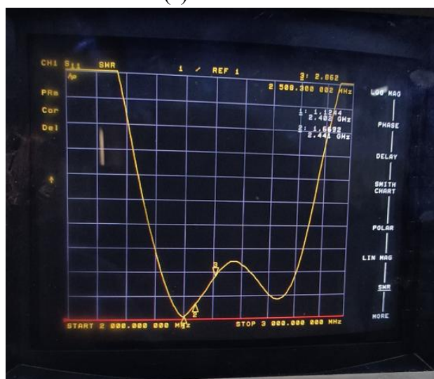
(c) VSWR
