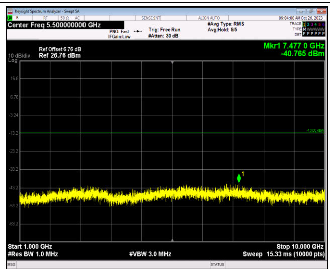
Band26-1.4MHz-QPSK-27033-1RB#0-Range2:1000~10000MHz
