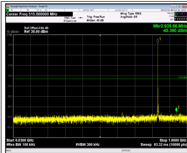
Band26-1.4MHz-QPSK-27033-1RB#0-Range1:30~1000MHz
