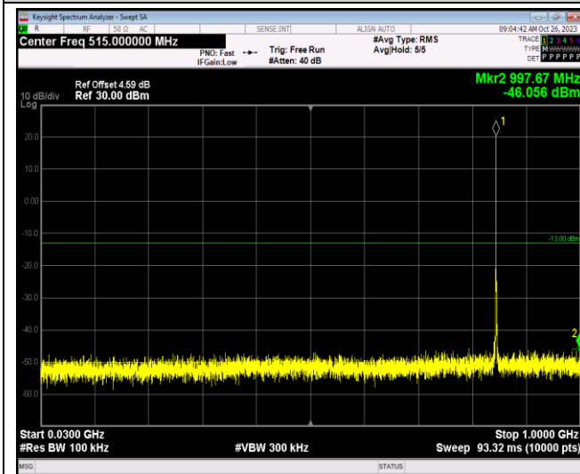
Band26-1.4MHz-16QAM-26697-1RB#0-Range1:30~1000MHz
