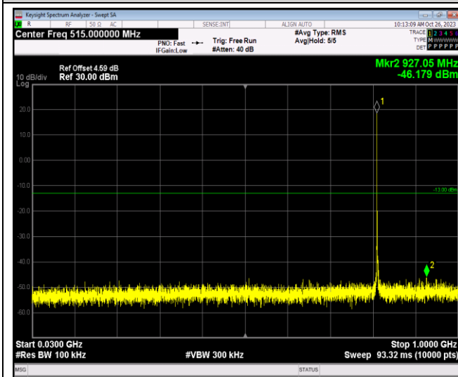
Band26-1.4MHz-16QAM-26697-1RB#0-Range1:30~1000MHz
