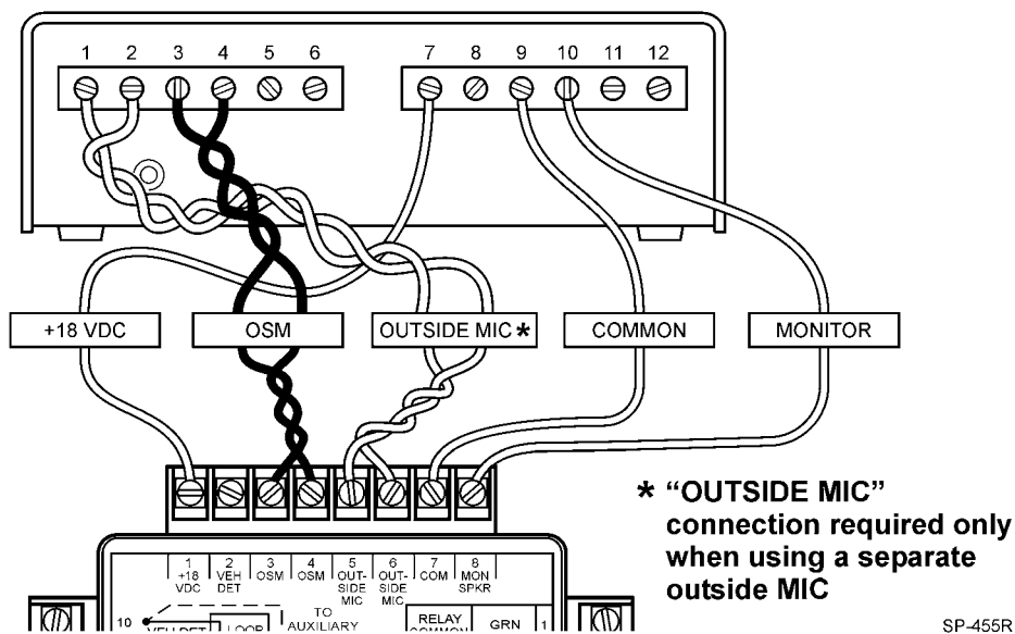
Figure 9. D-15B and D-15C (M478 BA and CA) Connections
