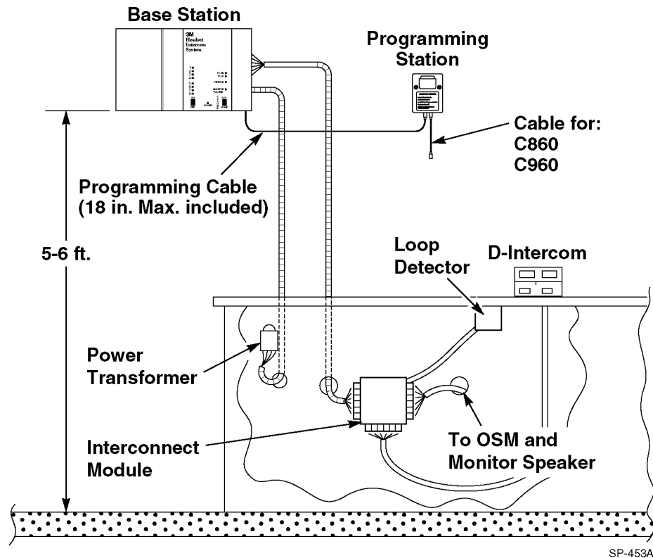
Figure 1. Typical Installation
