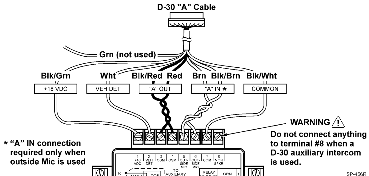
Figure 10. D-30 Connections
