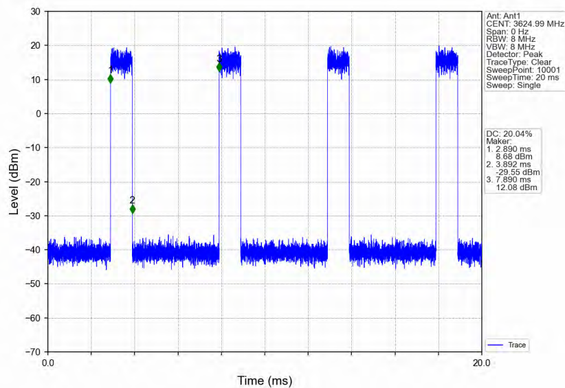
n48_30kHz_MIMO_NTNV_10MHz_CP-OFDM_256_QAM_3624.99MHz_Inner_Full
