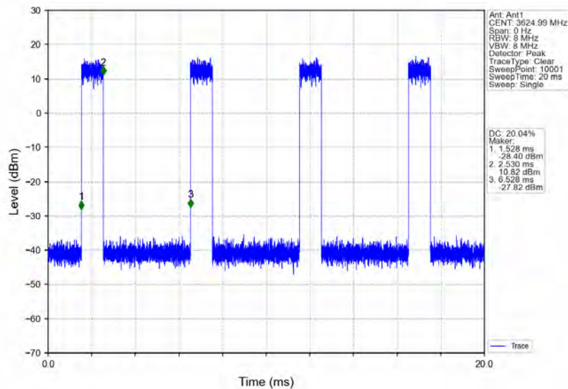
n48_30kHz_MIMO_NTNV_40MHz_CP-OFDM_64_QAM_3624.99MHz_Inner_Full
