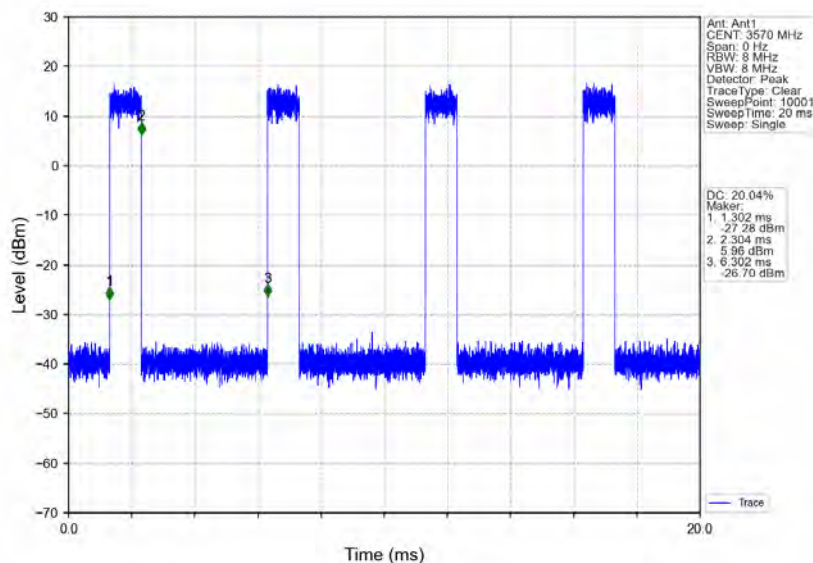
n48_30kHz_MIMO_NTNV_40MHz_CP-OFDM_64_QAM_3570MHz_Inner_Full
