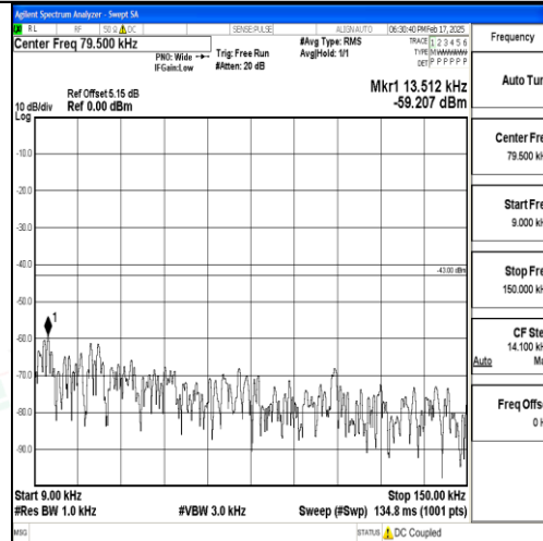
Band25_3MHz_QPSK_26365_1RB#0_0.009~0.15_0.009~0.15
