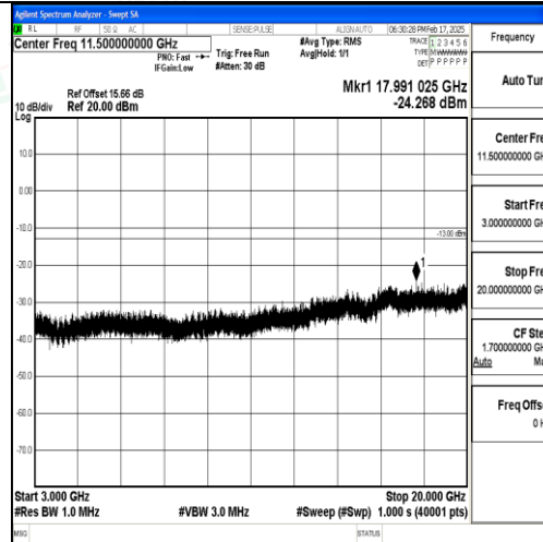
Band25_3MHz_16QAM_26055_1RB#0_3000~20000_3000~20000
