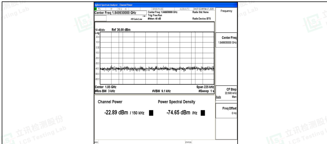
Band25_15MHz_QPSK_26115_75RB#0_Final1
