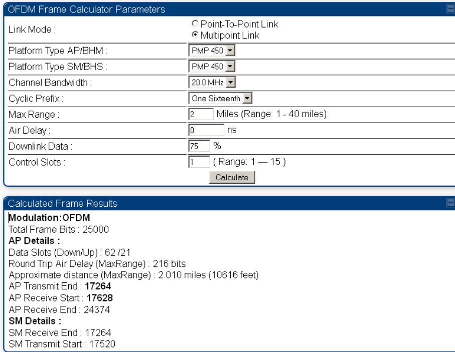
Figure 20 OFDM Frame Calculator tab
