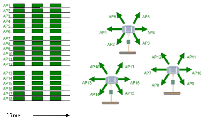
Figure 29 GPS timing throughout the network
