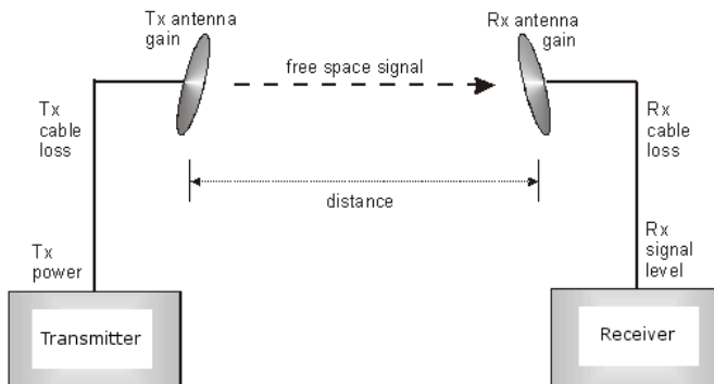
Figure 17 Determinants in Rx signal level
