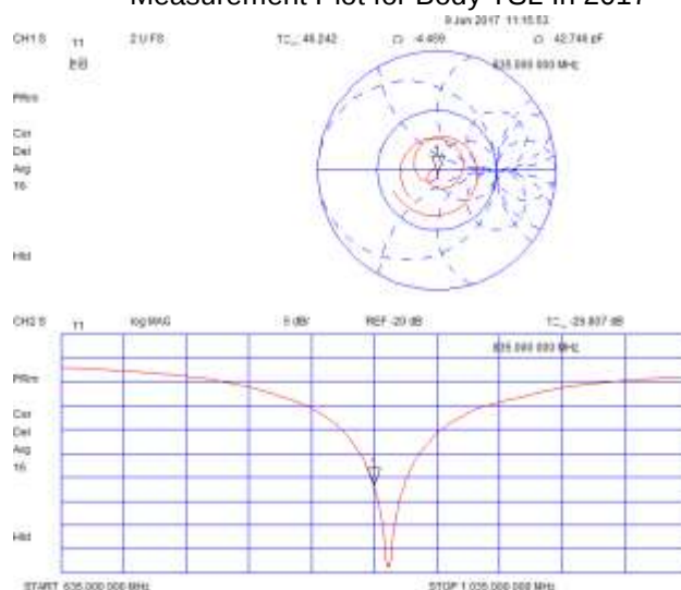
Measurement Plot for Body TSL In 2017
