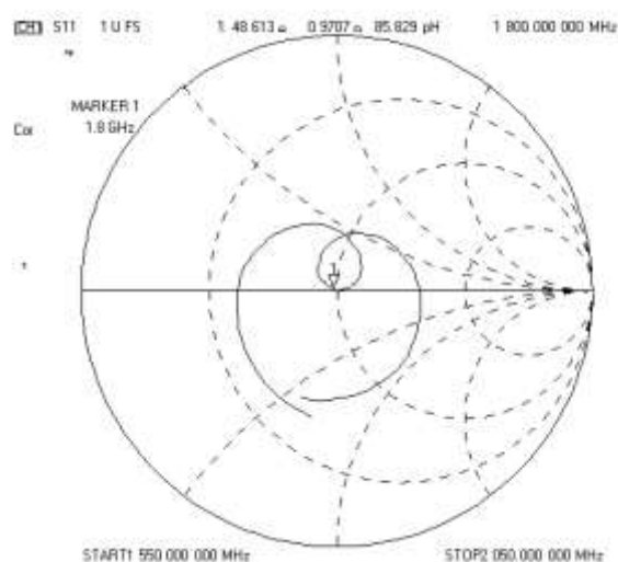
Measurement Plot for Body TSL In 2017 (Mar 15,2017)
