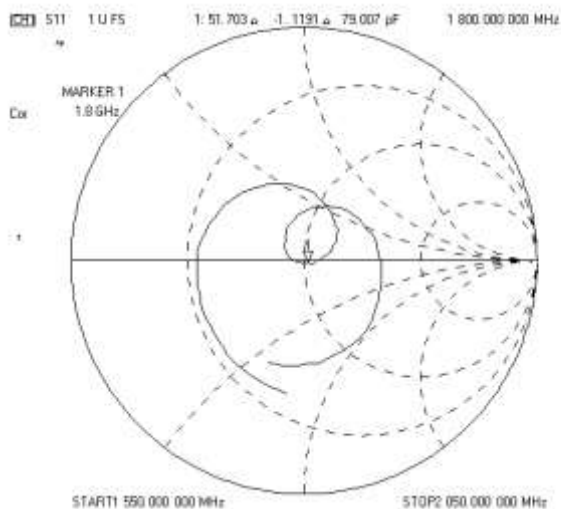
Measurement Plot for Head TSL In 2017 (Mar 15,2017)
