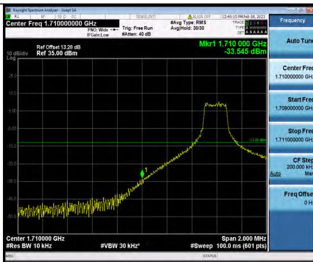
Band4-10MHz-64QAM-20000-50RB#0
