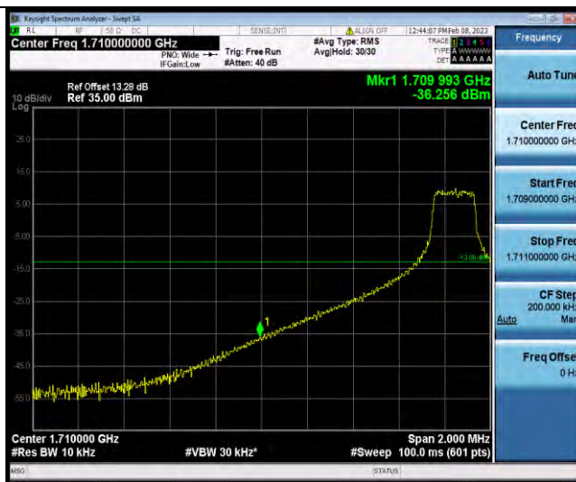
Band4-15MHz-64QAM-20025-75RB#0
