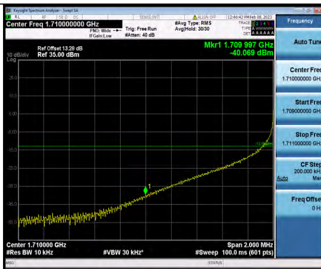
Band4-20MHz-64QAM-20050-100RB#0
