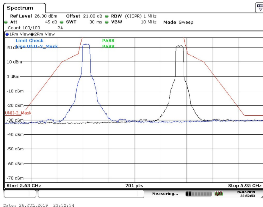
10MHz Channels_J2 Port
