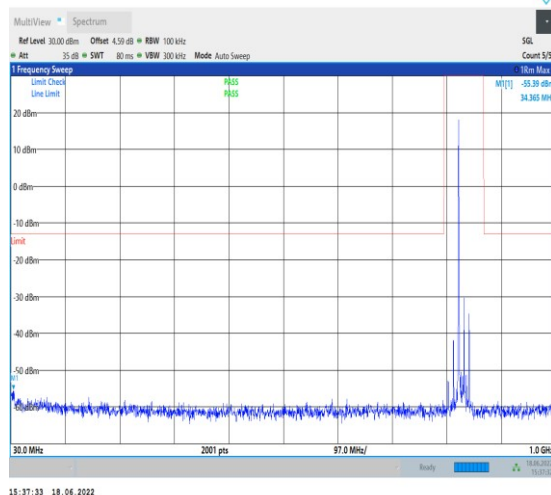
1-N5--15-20-M-1-DFT-PI2BPSK-Inner_1RB_Left-1@ 1-30-1000-Ant1--55.39--13-PASS
