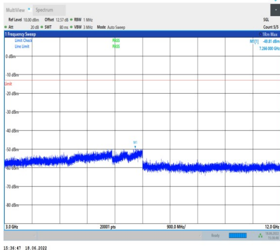
1-N5--15-20-L-1-DFT-PI2BPSK-Inner_1RB_Left-1@ 1-3000-12000-Ant1--49.81--13-PASS
