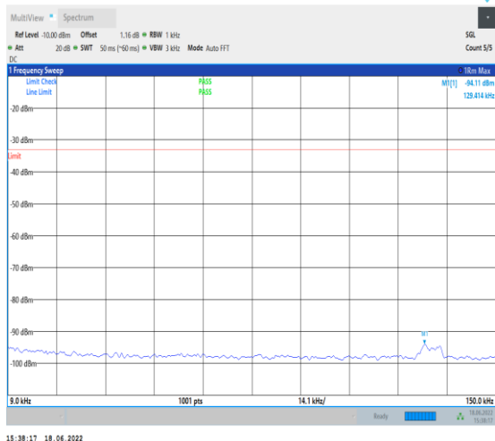
1-N5--15-20-H-1-DFT-PI2BPSK-Inner_1RB_Left-1@ 1-0.009-0.15-Ant1--94.11--33-PASS
