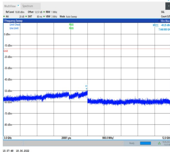
1-N5--15-20-M-1-DFT-PI2BPSK-Inner_1RB_Left-1@ 1-3000-12000-Ant1--49.25--13-PASS
