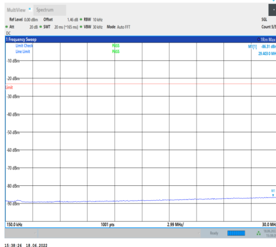
1-N5--15-20-H-1-DFT-PI2BPSK-Inner_1RB_Left-1@ 1-0.15-30-Ant1--86.31--23-PASS
