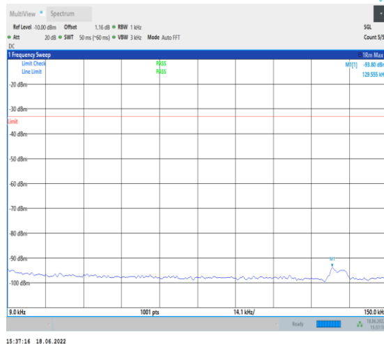
1-N5--15-20-M-1-DFT-PI2BPSK-Inner_1RB_Left-1@ 1-0.009-0.15-Ant1--93.80--33-PASS
