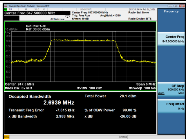
16QAM-20635
