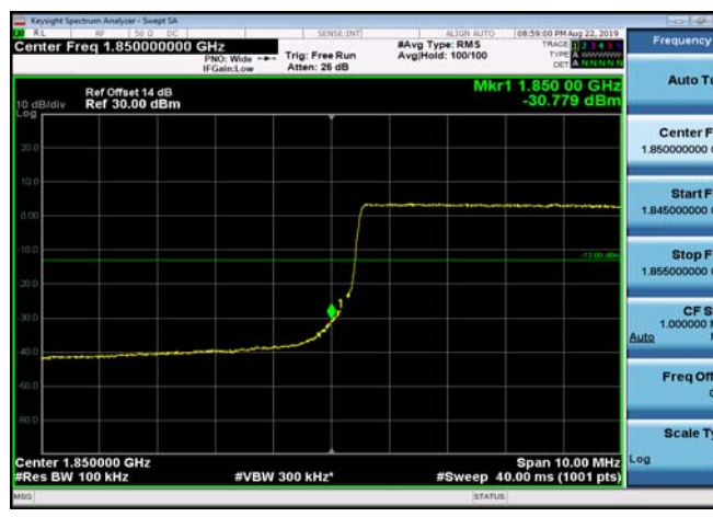
LowRange_FDD02_10MHz_1855_fullRB _Low_QPSK
