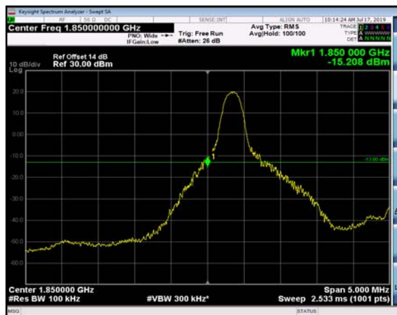
LowRange_FDD02_5MHz_1852.5_OneRB _low_QPSK
