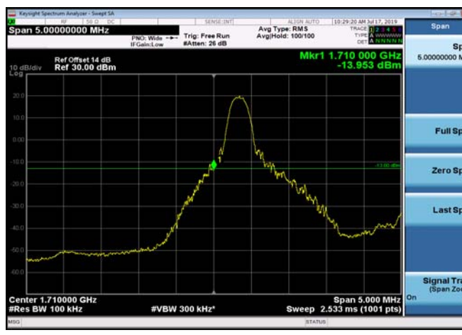
LowRange_FDD04_5MHz_1712.5_OneRB _low_QPSK
