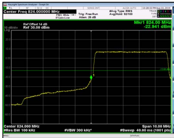
LowRange_FDD05_10MHz_829_OneRB _low_QPSK
