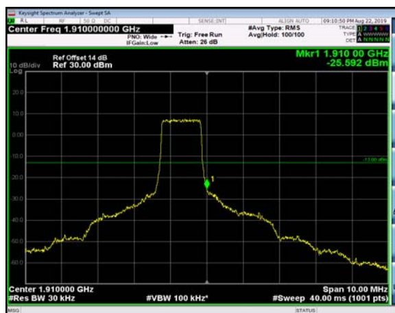
HighRange_FDD02_1.4MHz_1909.3 _fullRB_High_QPSK
