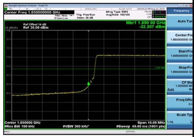
LowRange_FDD02_10MHz_1855_fullRB _Low_Q16
