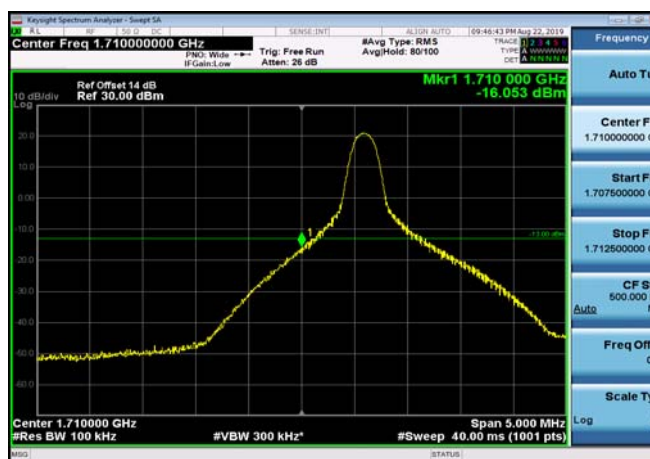
LowRange_FDD04_10MHz_1715_fullRB _Low_QPSK
