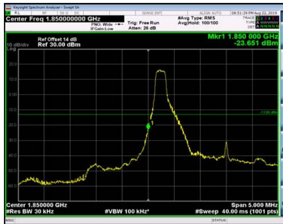
LowRange_FDD02_3MHz_1851.5_OneRB _low_QPSK
