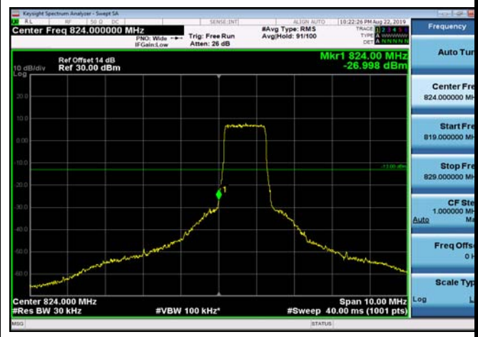
LowRange_FDD05_1.4MHz_824.7_fullRB _Low_Q16
