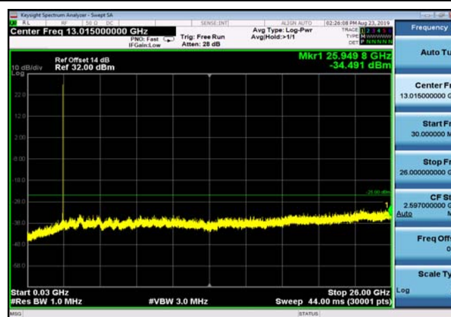
FDD07_LowRange_10MHz_30MHz~26GHz
