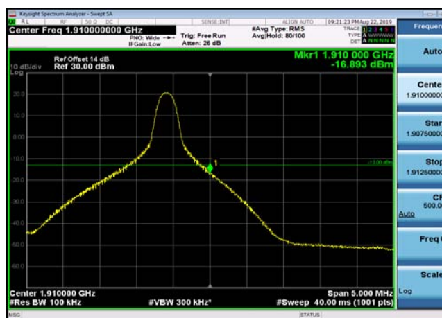
HighRange_FDD02_10MHz_1905_fullRB _High_QPSK
