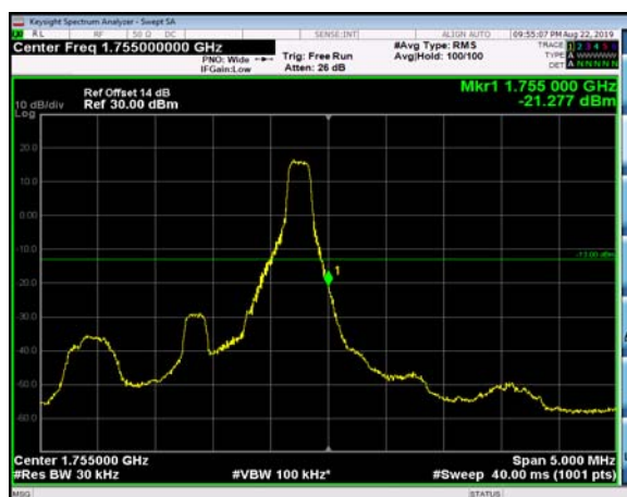
HighRange_FDD04_1.4MHz_1754.3 _fullRB_High_QPSK
