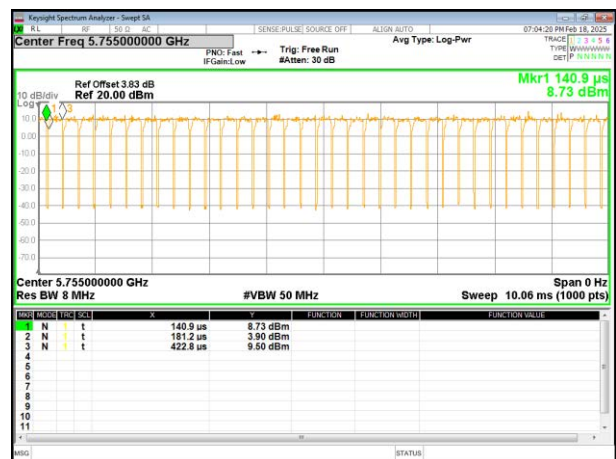
(802.11 ac40) plot
