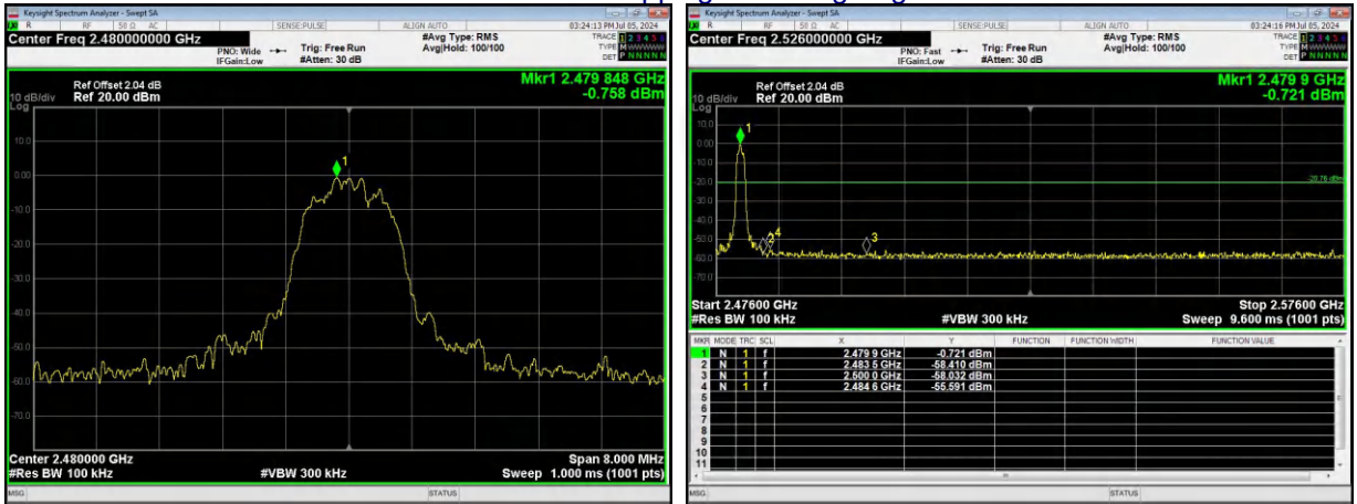
8-DPSK No-hopping Band edge-right side
