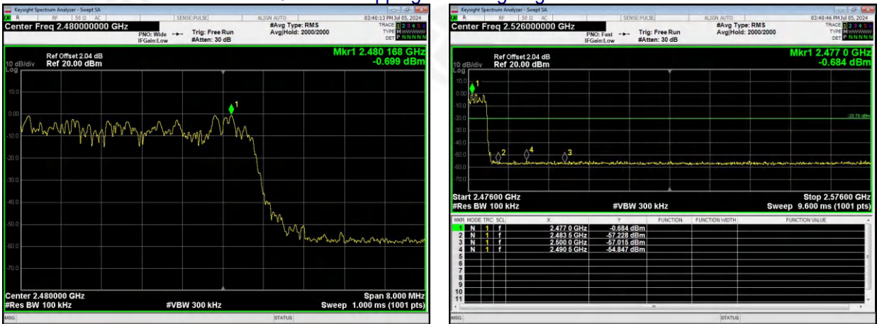
8-DPSK Hopping Band edge-right side
