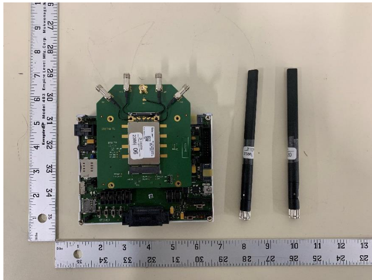
Figure B1. DUT Top View
