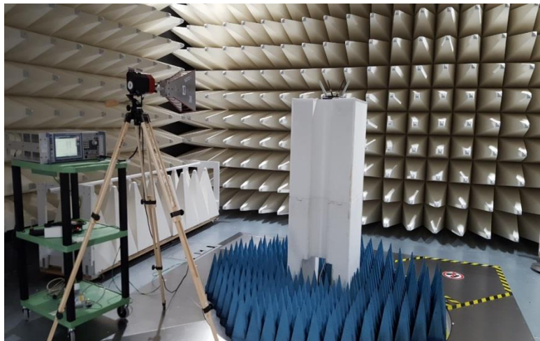
Figure B3. Radiated Setup HR
