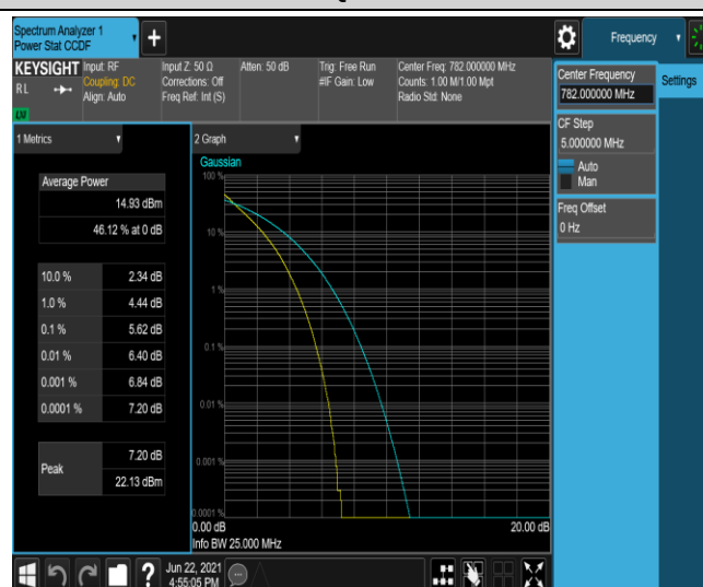
Band13-10MHz-16QAM-23230-1RB#0
