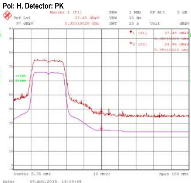
Figure 4-4: Band-Edge Compliance of RF Radiated Emission 802.11ac, Primary, Ch. 64, 5320 MHz, Centre of Band-Edge: 5350 MHz Pol: H, Detector: PK
