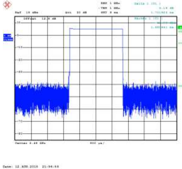
Figure 5-22: Time of Occupancy (Dwell Time) Freq. Hopping, Static PBRS, DH3
