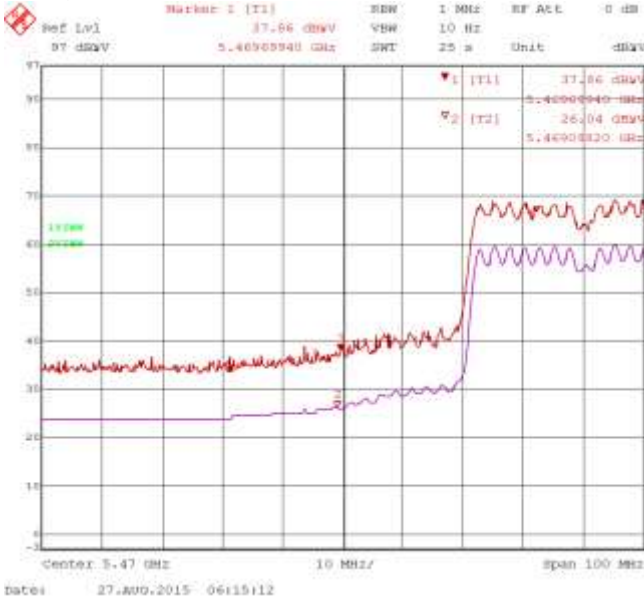
Figure 3-49: Band-Edge Compliance of RF Radiated Emission 802.11n, MIMO, Ch. 102, 55100 MHz, Centre of Band-Edge: 5470 MHz Pol: V, Detector: PK
