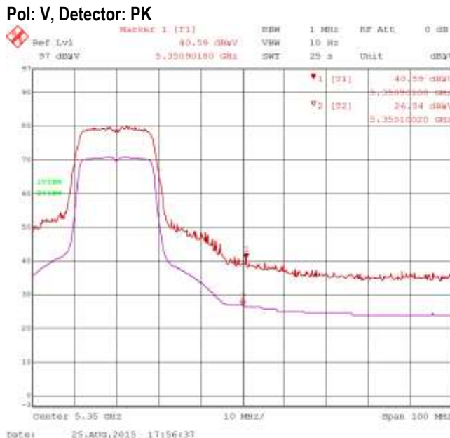
Figure 4-3: Band-Edge Compliance of RF Radiated Emission 802.11ac, Primary, Ch. 64, 5320 MHz, Centre of Band-Edge: 5350 MHz Pol: V, Detector: PK
