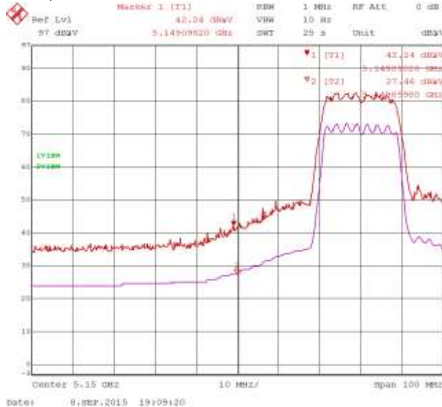
Figure 3-37: Band-Edge Compliance of RF Radiated Emission 802.11n, MIMO, Ch. 36, 5180 MHz, Centre of Band-Edge: 5150 MHz Pol: V, Detector: PK
