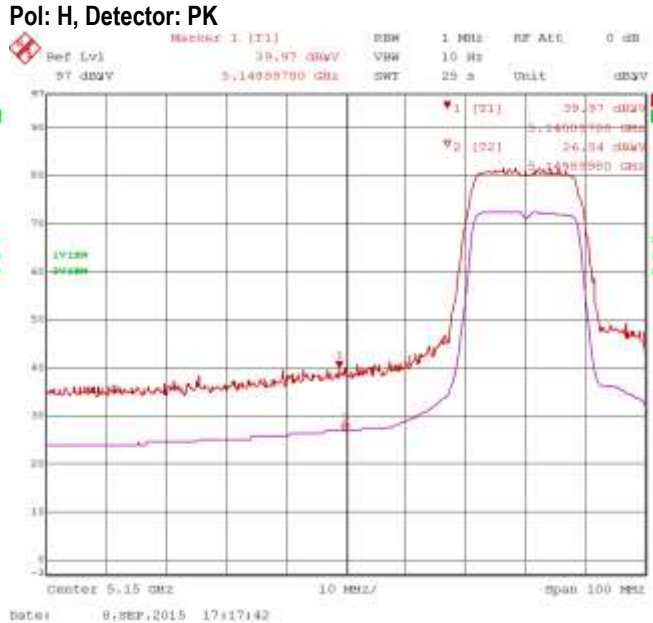
Figure 4-2: Band-Edge Compliance of RF Radiated Emission 802.11ac, Primary, Ch. 36, 5180 MHz, Centre of Band-Edge: 5150 MHz Pol: H, Detector: PK
