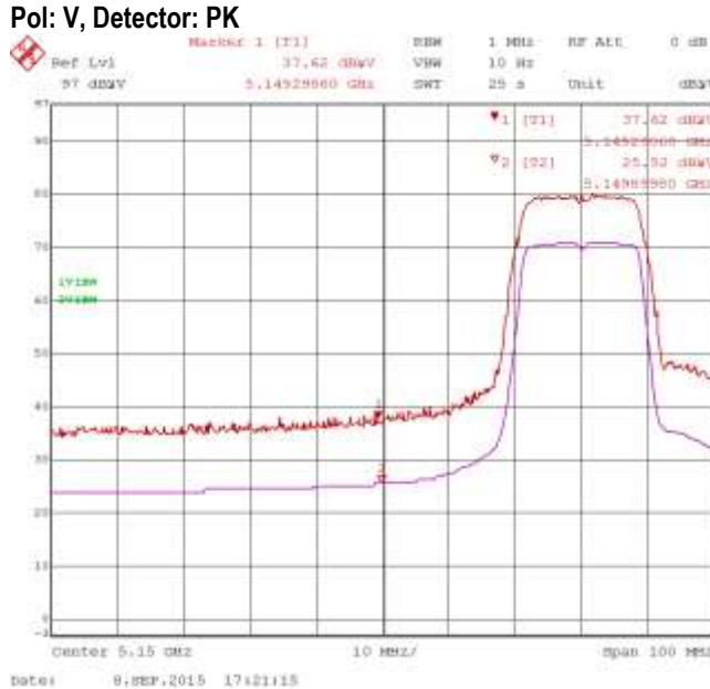
Figure 4-1: Band-Edge Compliance of RF Radiated Emission 802.11ac, Primary, Ch. 36, 5180 MHz, Centre of Band-Edge: 5150 MHz Pol: V, Detector: PK
