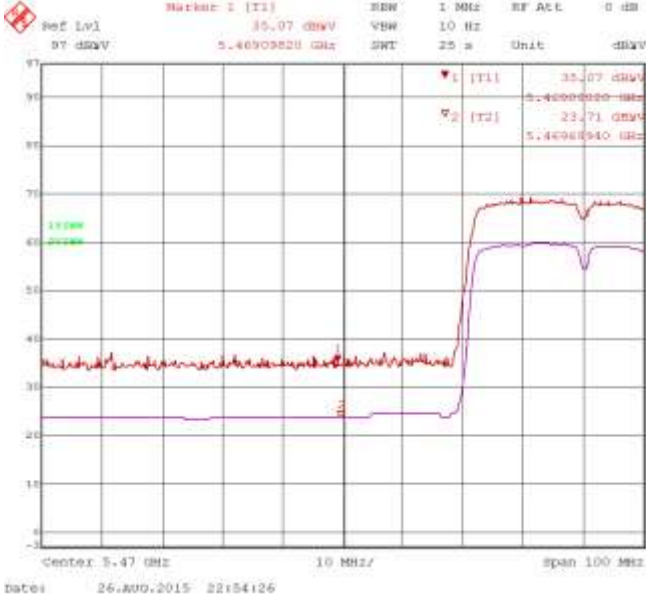
Figure 3-35: Band-Edge Compliance of RF Radiated Emission 802.11n, Secondary, Ch. 102, 55100 MHz, Centre of Band-Edge: 5470 MHz Pol: V, Detector: PK Figure 3-36: Band-Edge Compliance of RF Radiated Emission. 802.11n, Secondary, Ch. 102, 55100 MHz, Centre of Band-Edge: 5470 MHz Pol: H, Detector: PK
