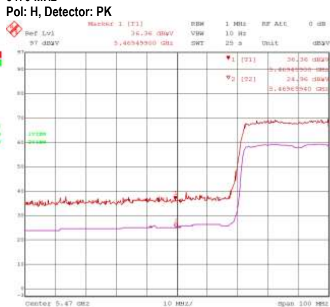
Figure 4-20: Band-Edge Compliance of RF Radiated Emission. 802.11ac, Primary, Ch. 106, 5530 MHz, Centre of Band-Edge: 5470 MHz Pol: H, Detector: PK
